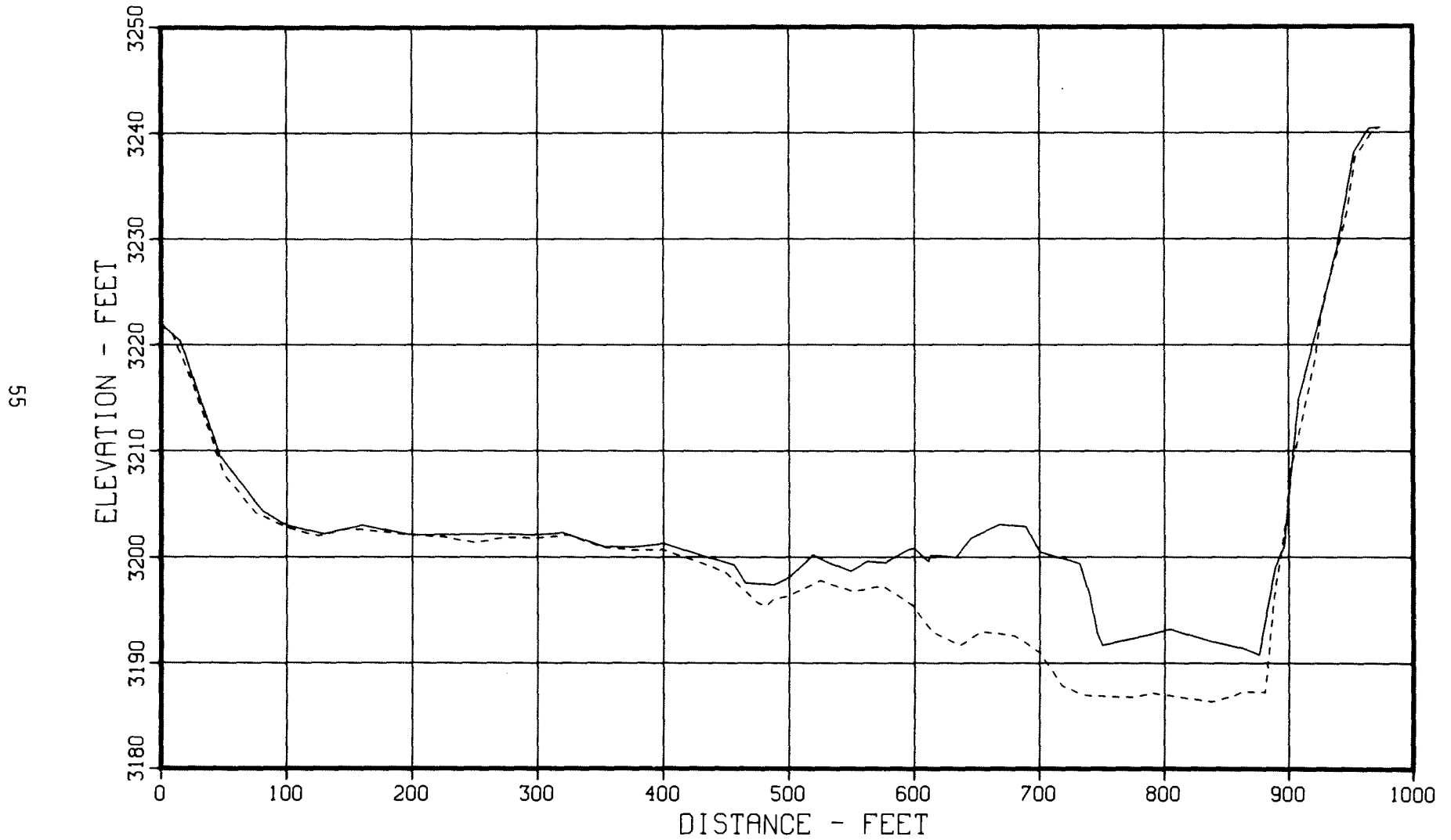
Figure 33. - 1949 and 1979 sedimentation range profiles, Cheyenne River - Range 14.
