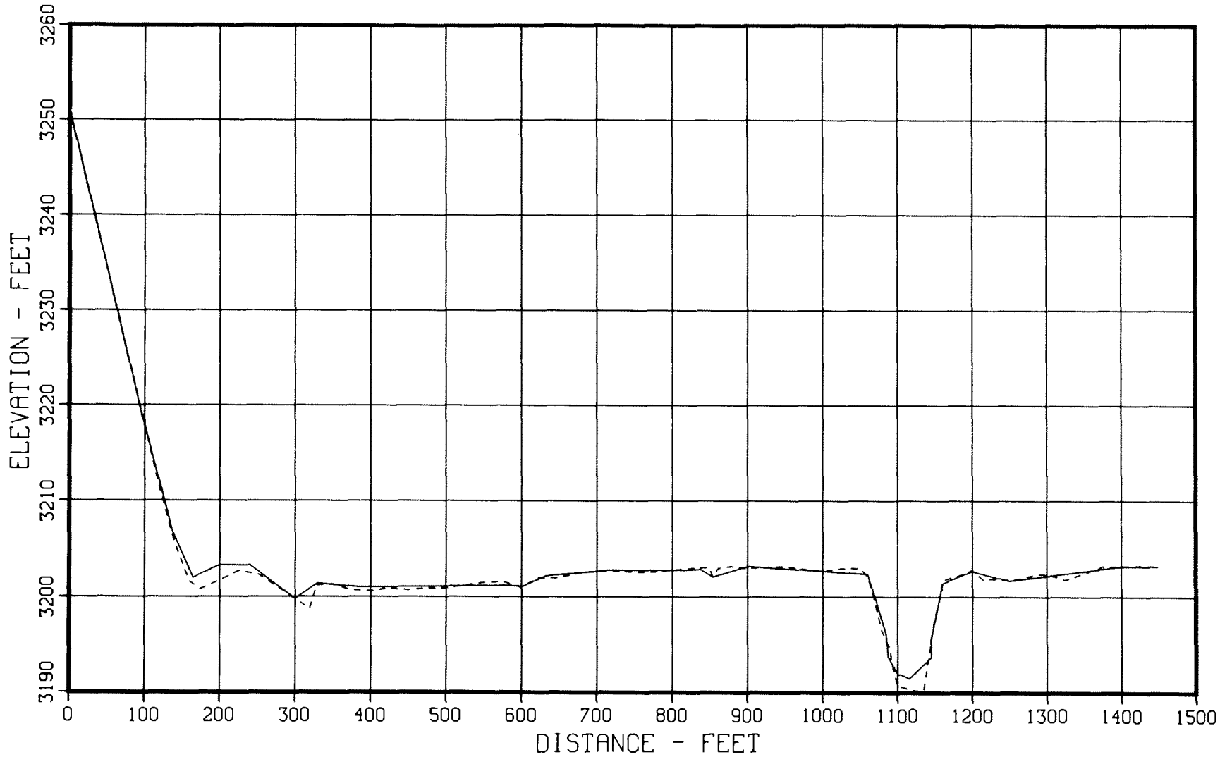
Figure 53. - 1949 and 1979 sedimentation range profiles, Horsehead Creek - Range 48.
