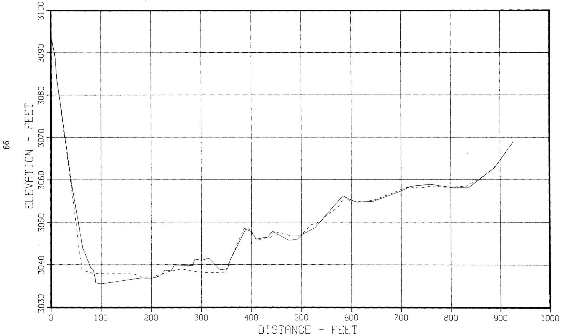
Figure 76. - Degradation range profiles - Range 4.0.
