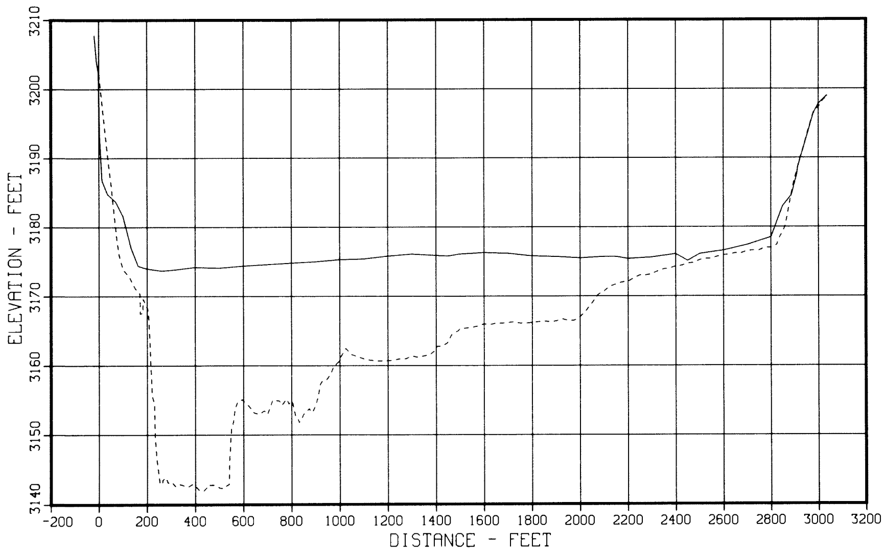
Figure 26. - 1949 and 1979 sedimentation range profiles, Cheyenne River - Range 7.
