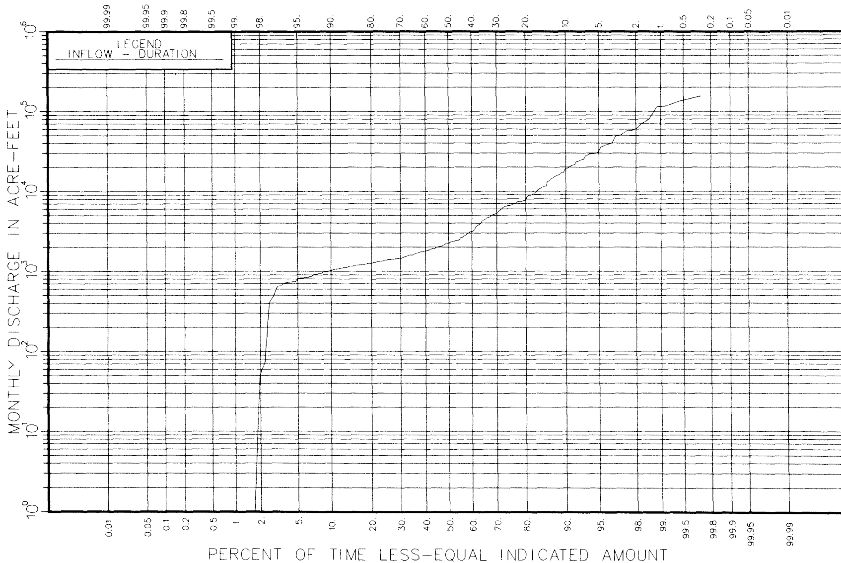
Figure 3. - Inflow-duration curve for monthly inflow discharges.
