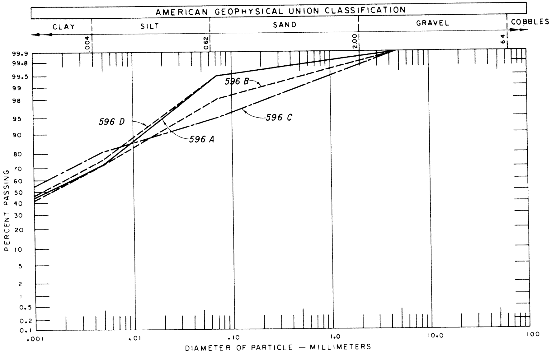
Figure 65. - Particle size analyses curves - Range 7 - Sheet 2 of 2.
