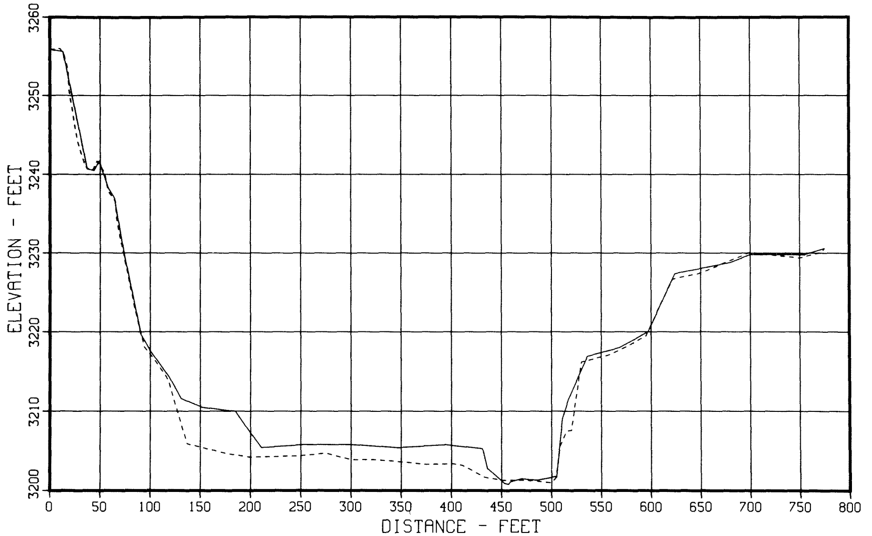
Figure 37. - 1949 and 1979 sedimentation range profiles, Cheyenne River - Range 17.
