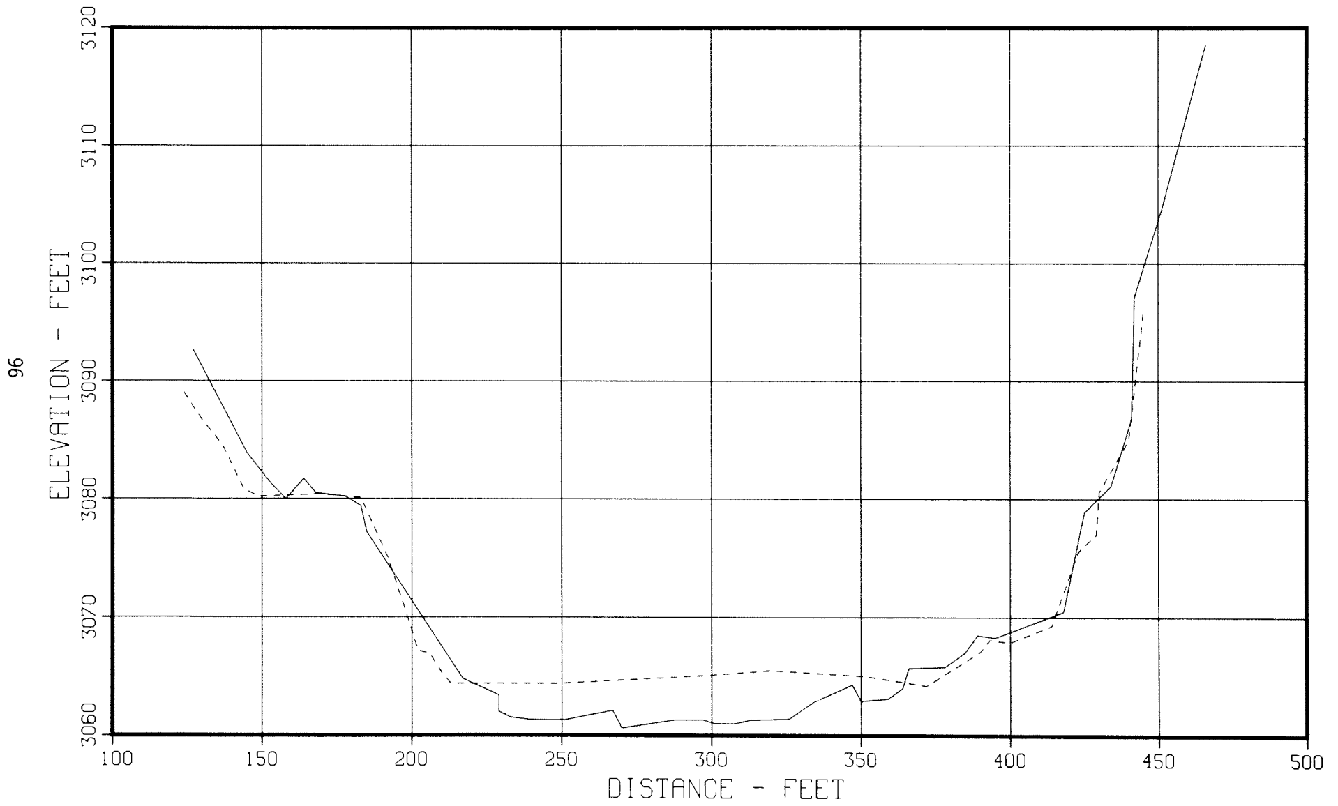
Figure 73. - Degradation range profiles - Range 0.2.
