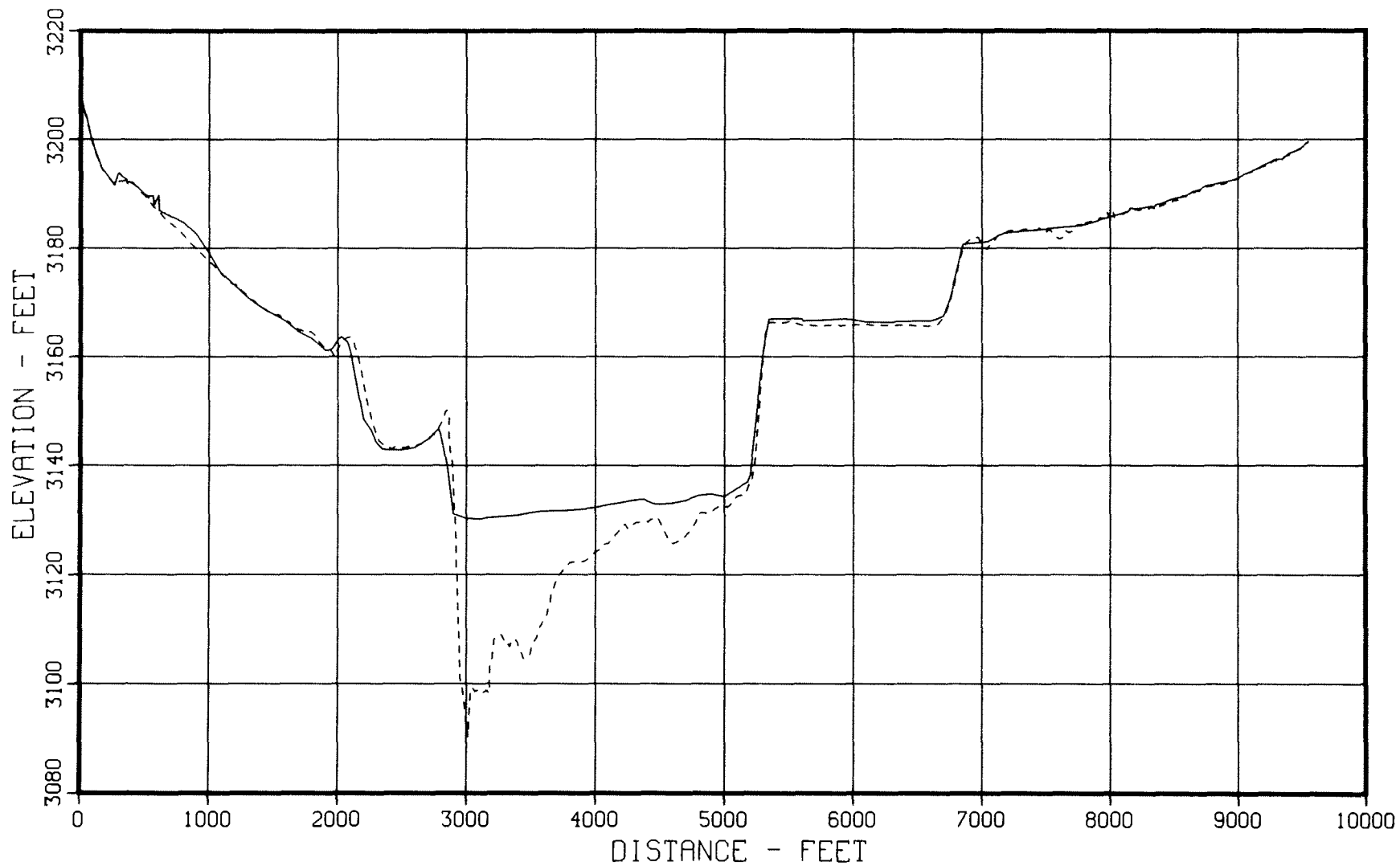
Figure 23. - 1949 and 1979 sedimentation range profiles, Cheyenne River - Range 5.
