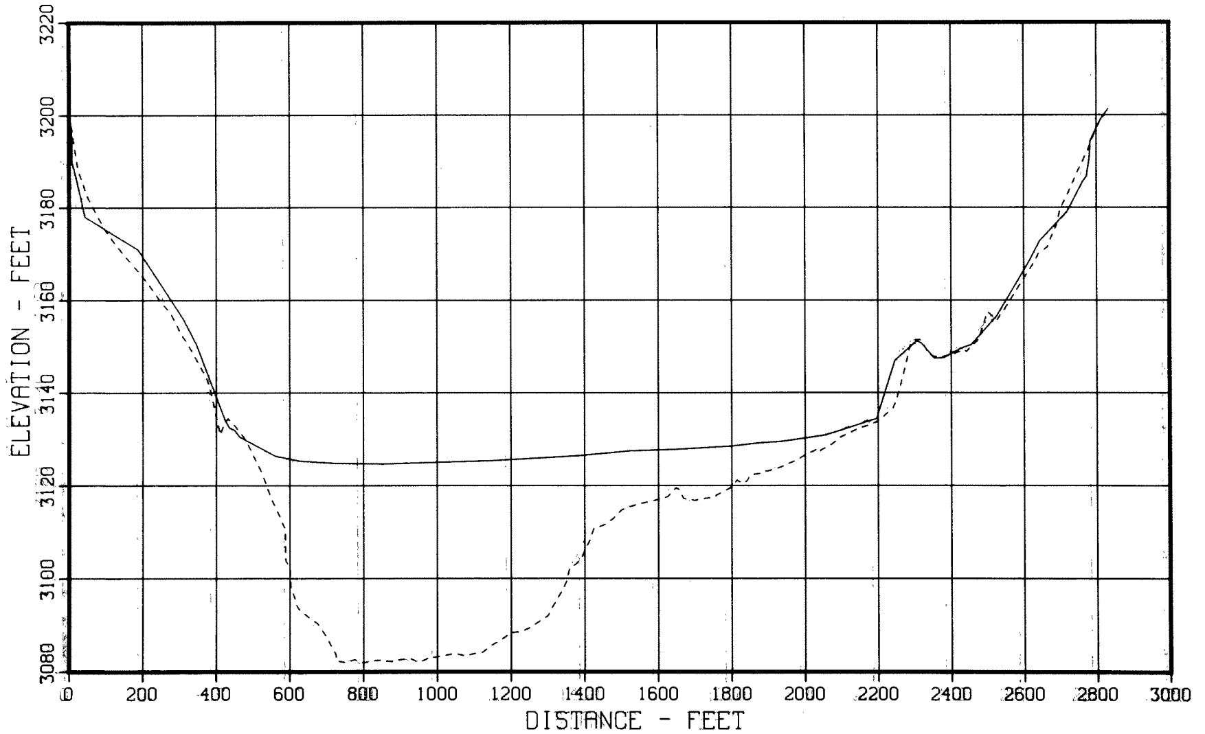
Figure 20. - 1949 and 1979 sedimentation range profiles, Cheyenne River - Range 3.
