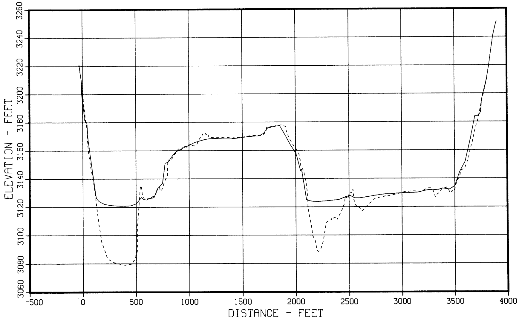
Figure 18. - 1949 and 1979 sedimentation range profiles, Cheyenne River - Range 2.
