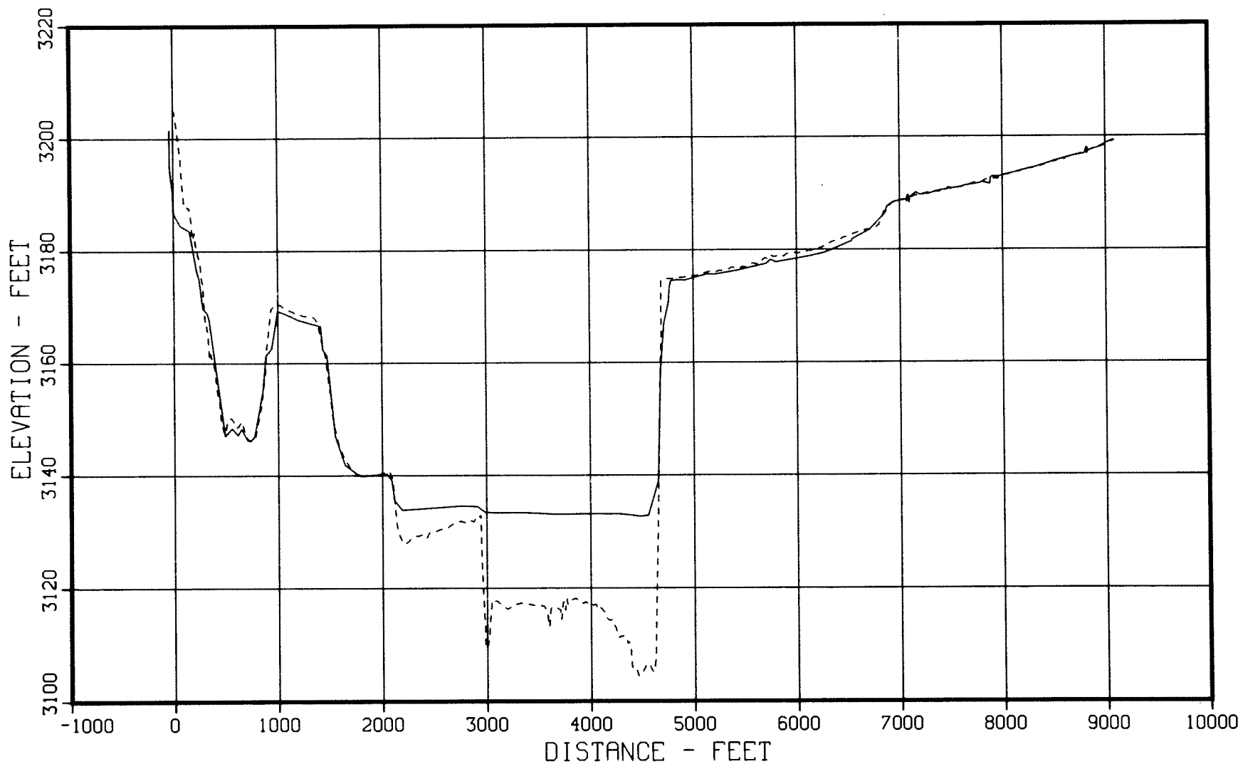
Figure 24. - 1949 and 1979 sedimentation range profiles, Cheyenne River - Range 6.
