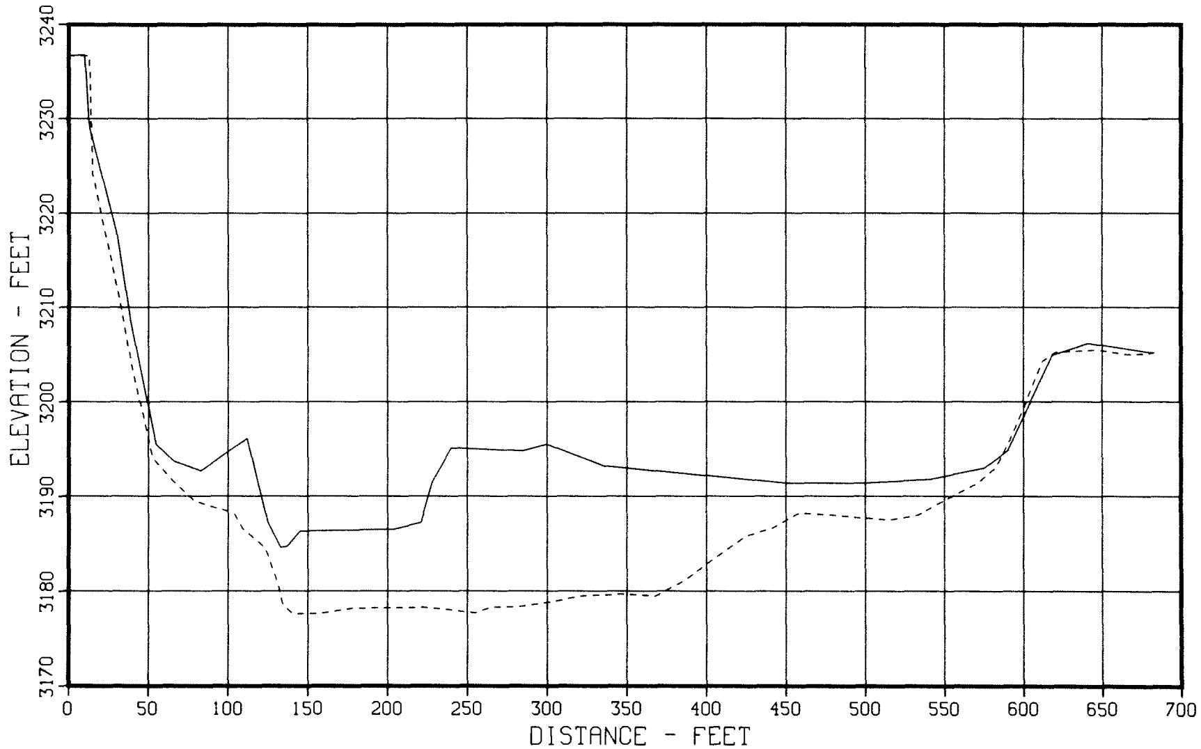
Figure 31. - 1949 and 1979 sedimentation range profiles, Cheyenne River - Range 12.
