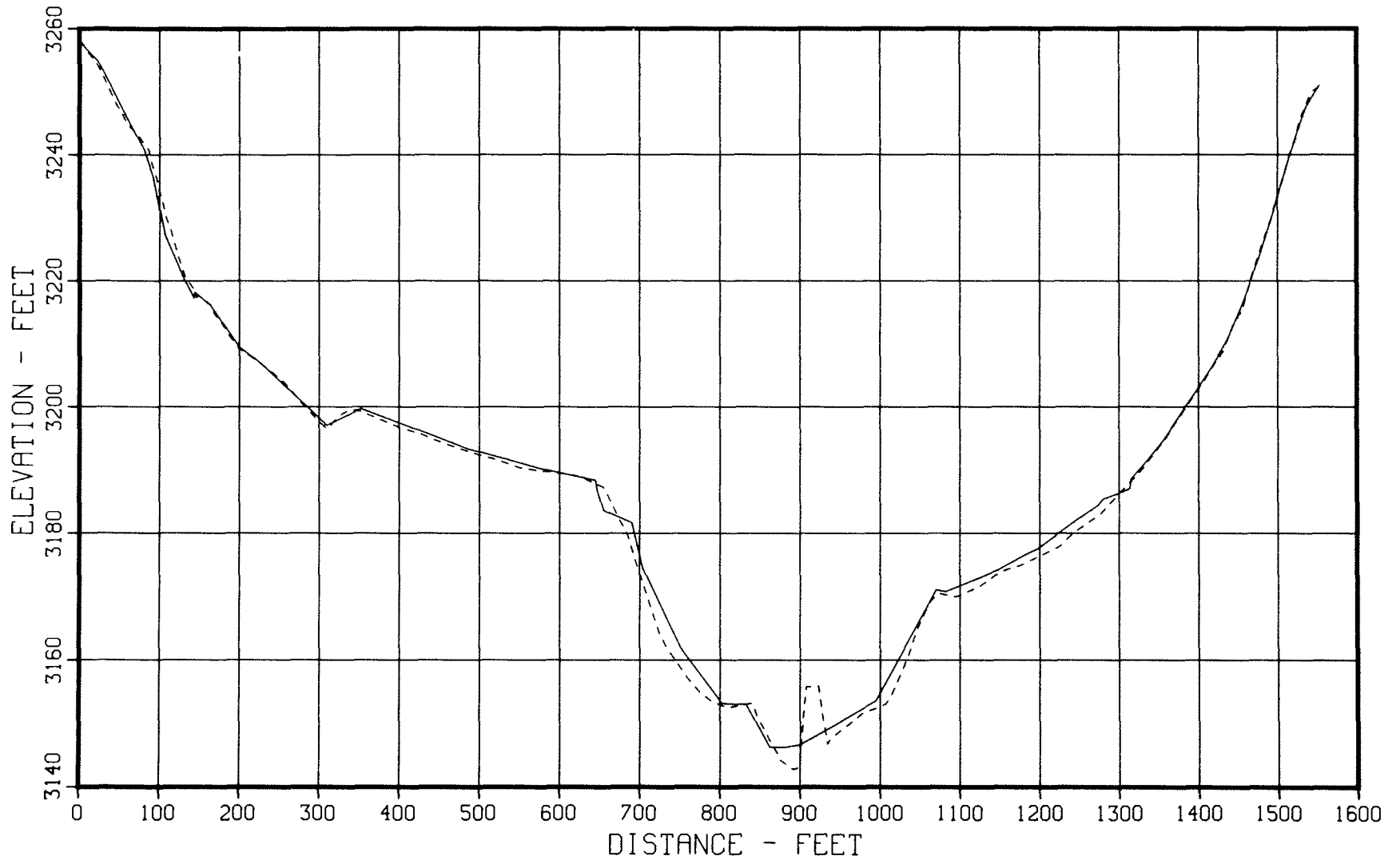
Figure 39. - 1949 and 1979 sedimentation range profiles at mouth of first downstream unnamed canyon - Range 20.
