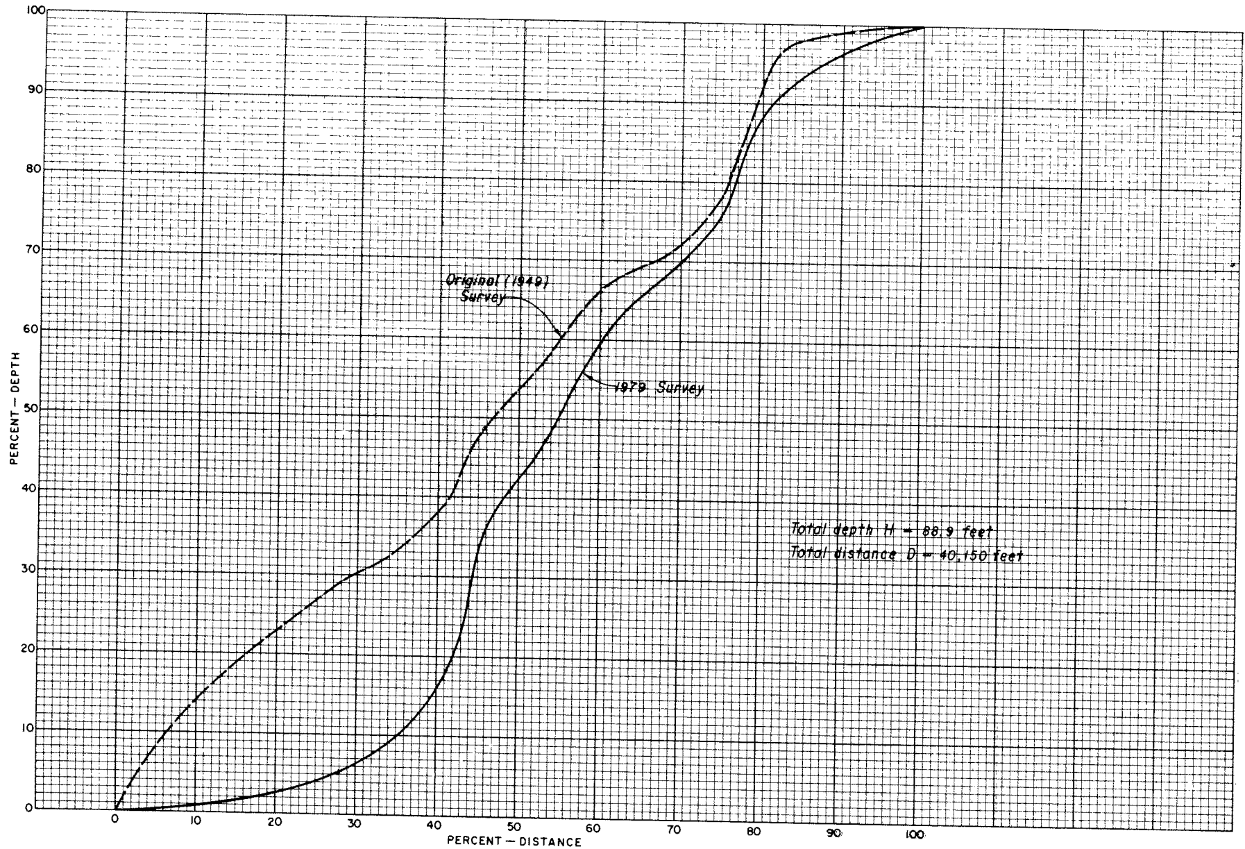
Figure 13. - Percent depth-percent distance for Horsehead Creek above confluence of Cheyenne River and Horsehead Creek.
