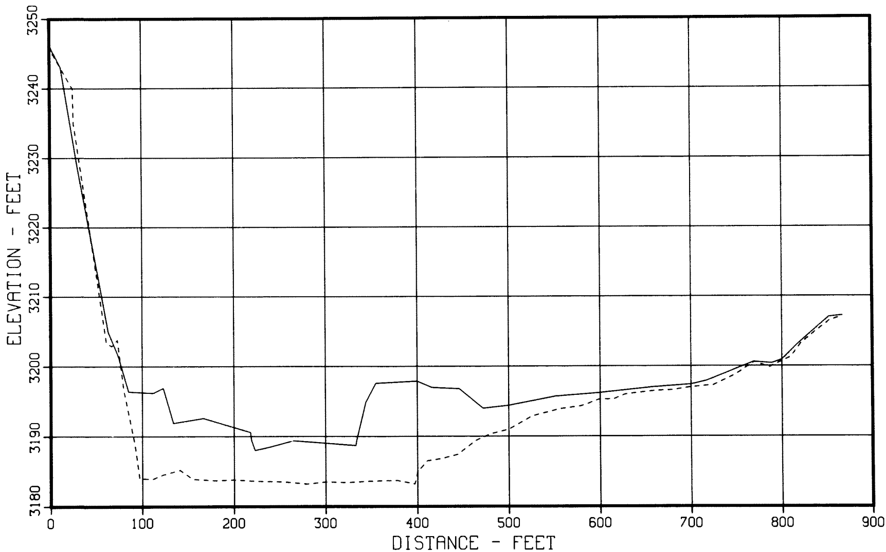
Figure 32. - 1949 and 1979 sedimentation range profiles, Cheyenne River - Range 13.
