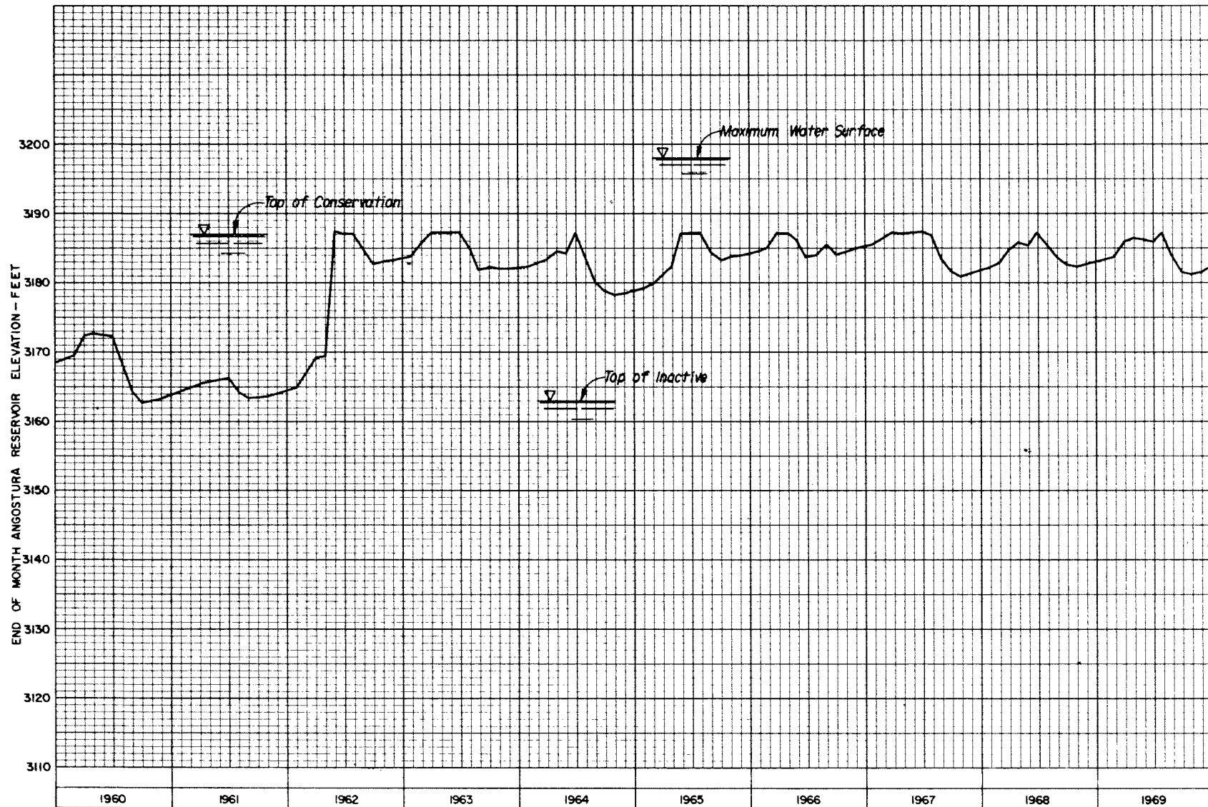
Figure 5. - End-of-month Angostura Reservoir elevation - Sheet 2 of 3.
