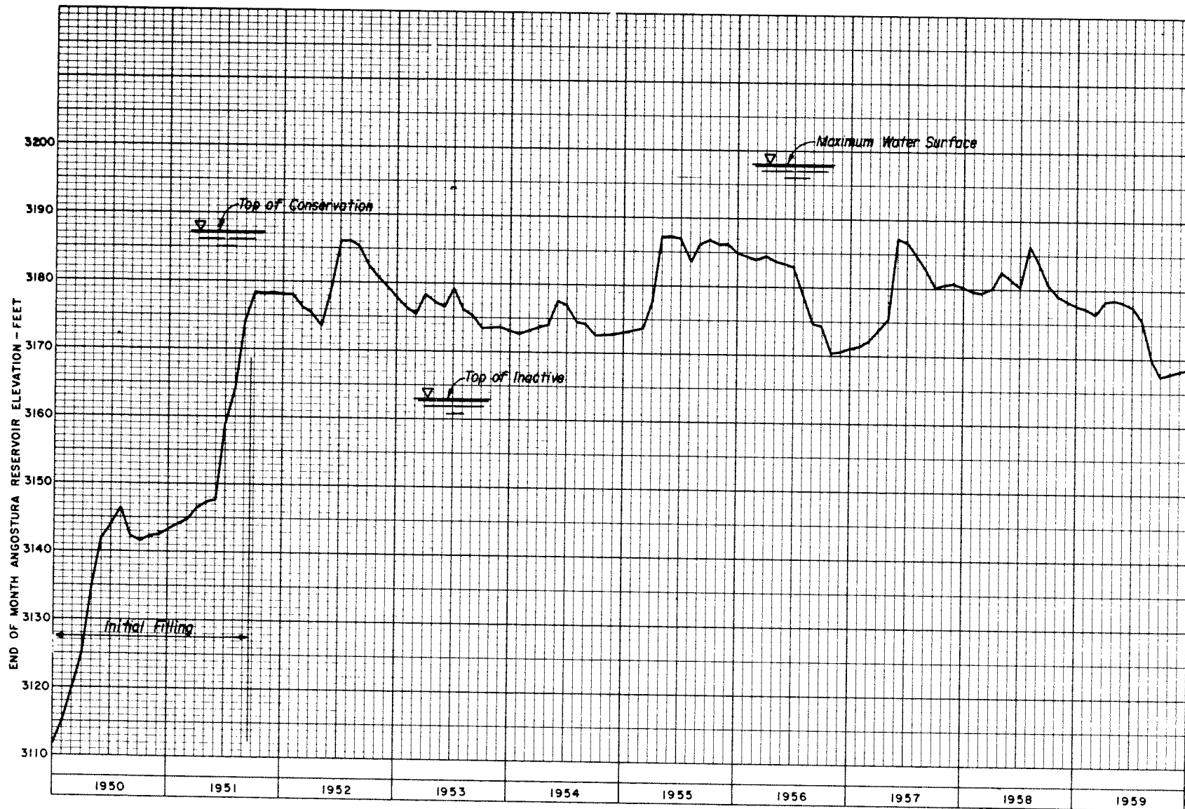
Figure 5. - End-of-month Angostura Reservoir elevation - Sheet 1 of 3.
