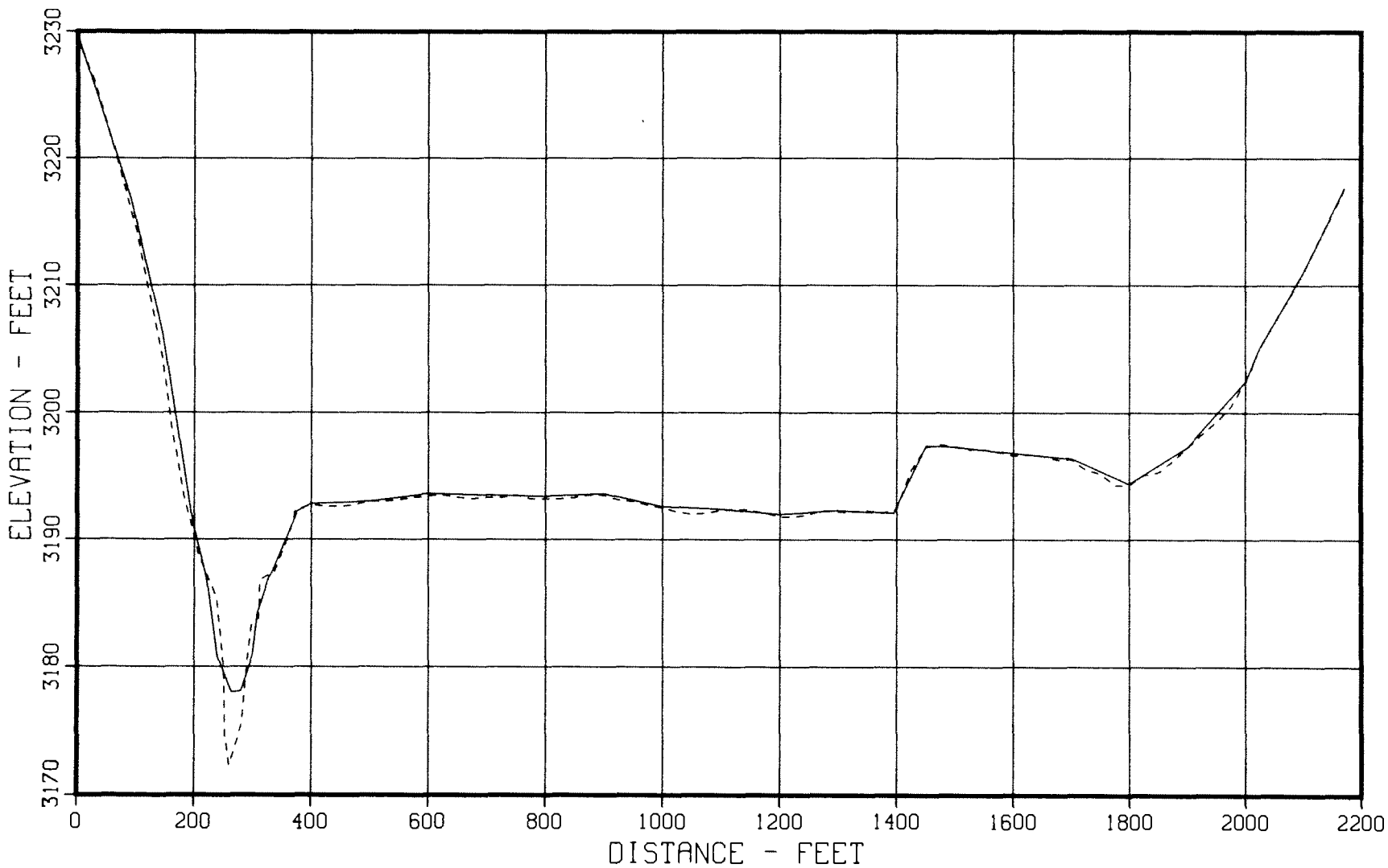
Figure 51. - 1949 and 1979 sedimentation range profiles, Horsehead Creek - Range 46.
