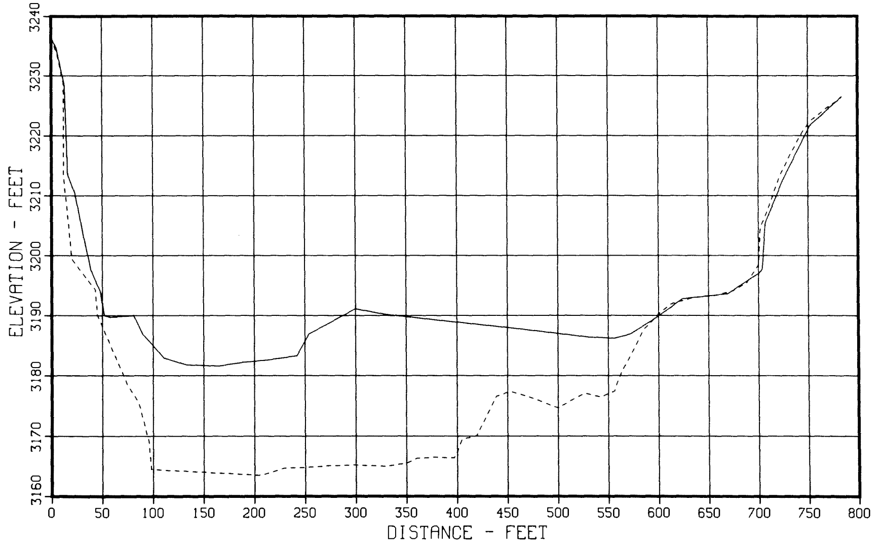
Figure 29. - 1949 and 1979 sedimentation range profiles, Cheyenne River - Range 10.
