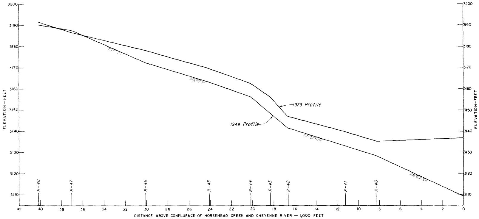
Figure 11. - Longitudinal profiles for Horsehead Creek.
