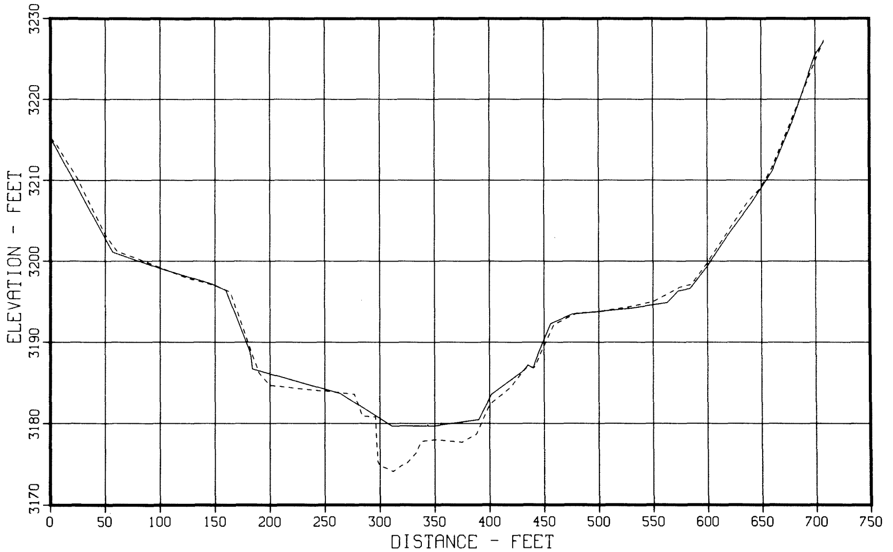
Figure 59. - 1949 and 1979 sedimentation range profiles, Dry Creek - Range 62.
