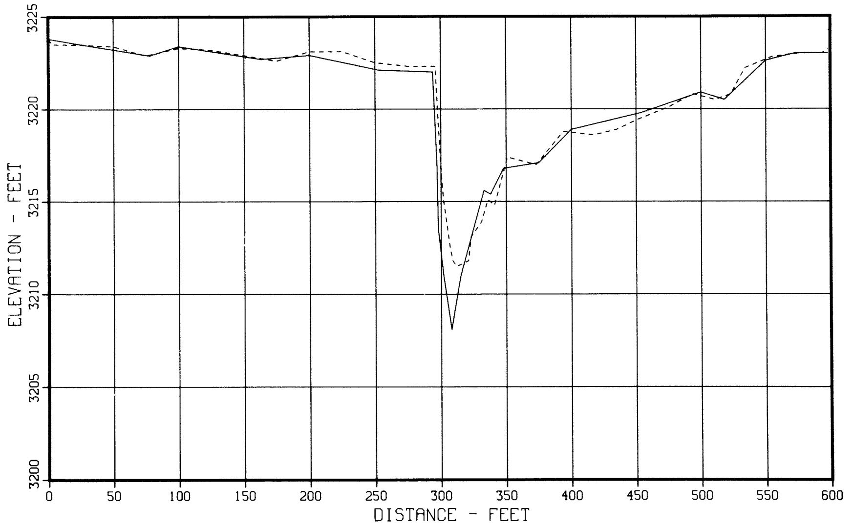
Figure 56. - 1949 and 1979 sedimentation range profiles, Horsehead Creek - Range 51.
