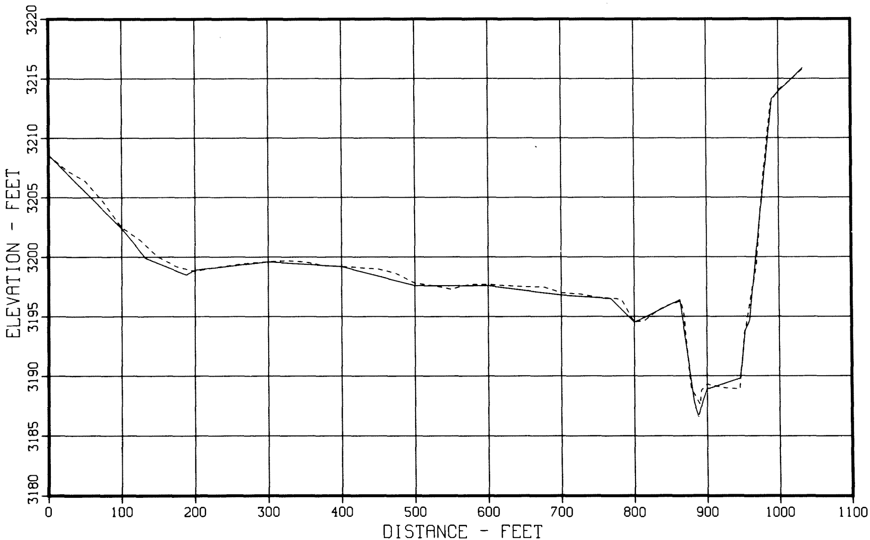
Figure 52. - 1949 and 1979 sedimentation range profiles, Horsehead Creek - Range 47.
