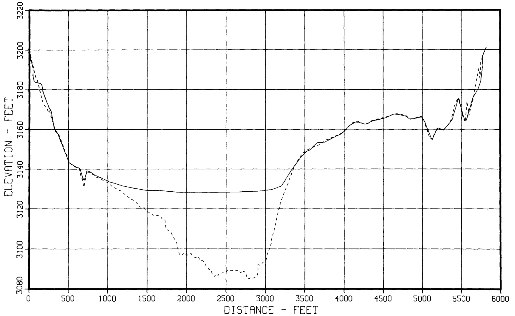
Figure 21. - 1949 and 1979 sedimentation range profiles, Cheyenne River - Range 3A.
