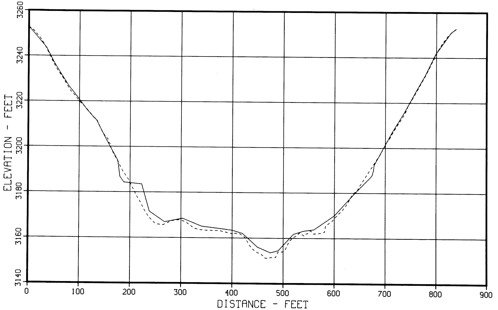
Figure 41. - 1949 and 1979 sedimentation range profiles, Sheps Canyon, Range 31.
