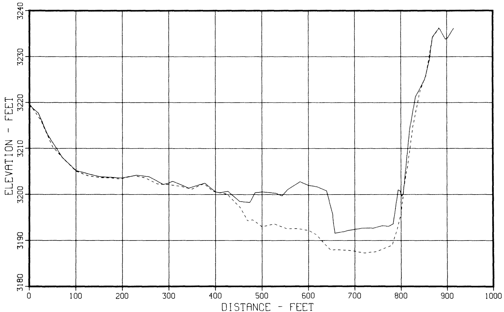
Figure 34. - 1949 and 1979 sedimentation range profiles, Cheyenne River - Range 14A.
