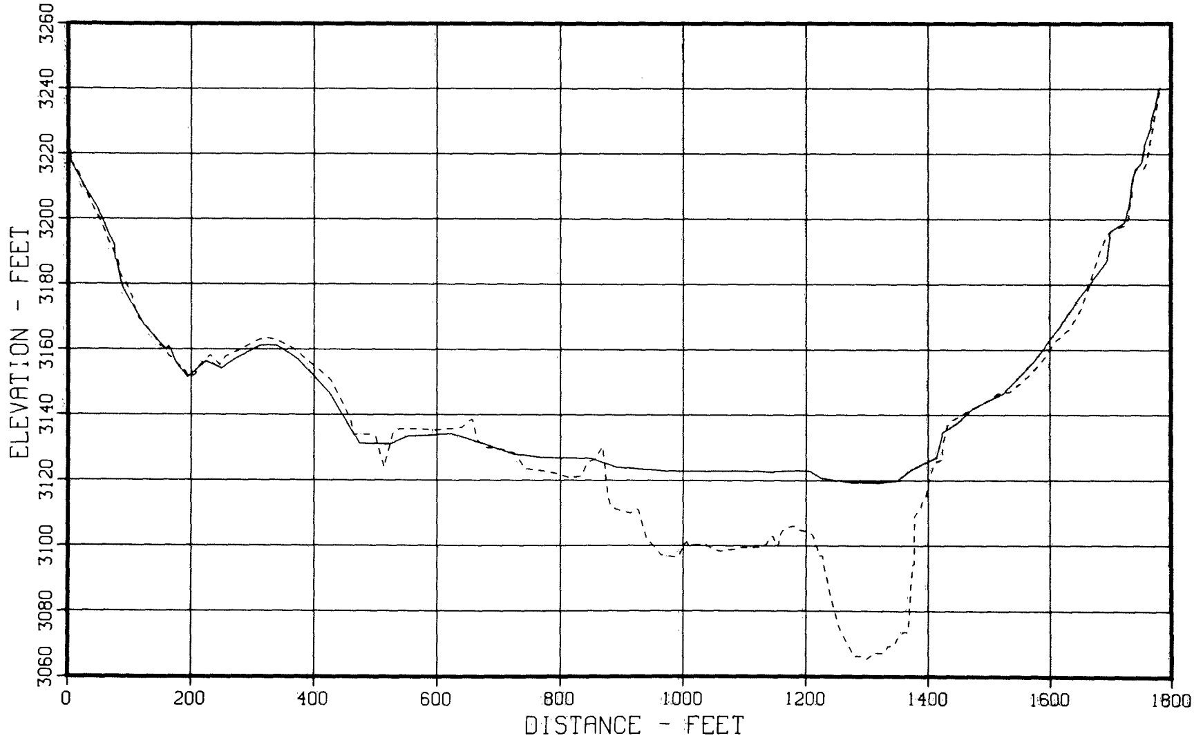
Figure 17. - 1949 and 1979 sedimentation range profiles, Cheyenne River - Range 1.
