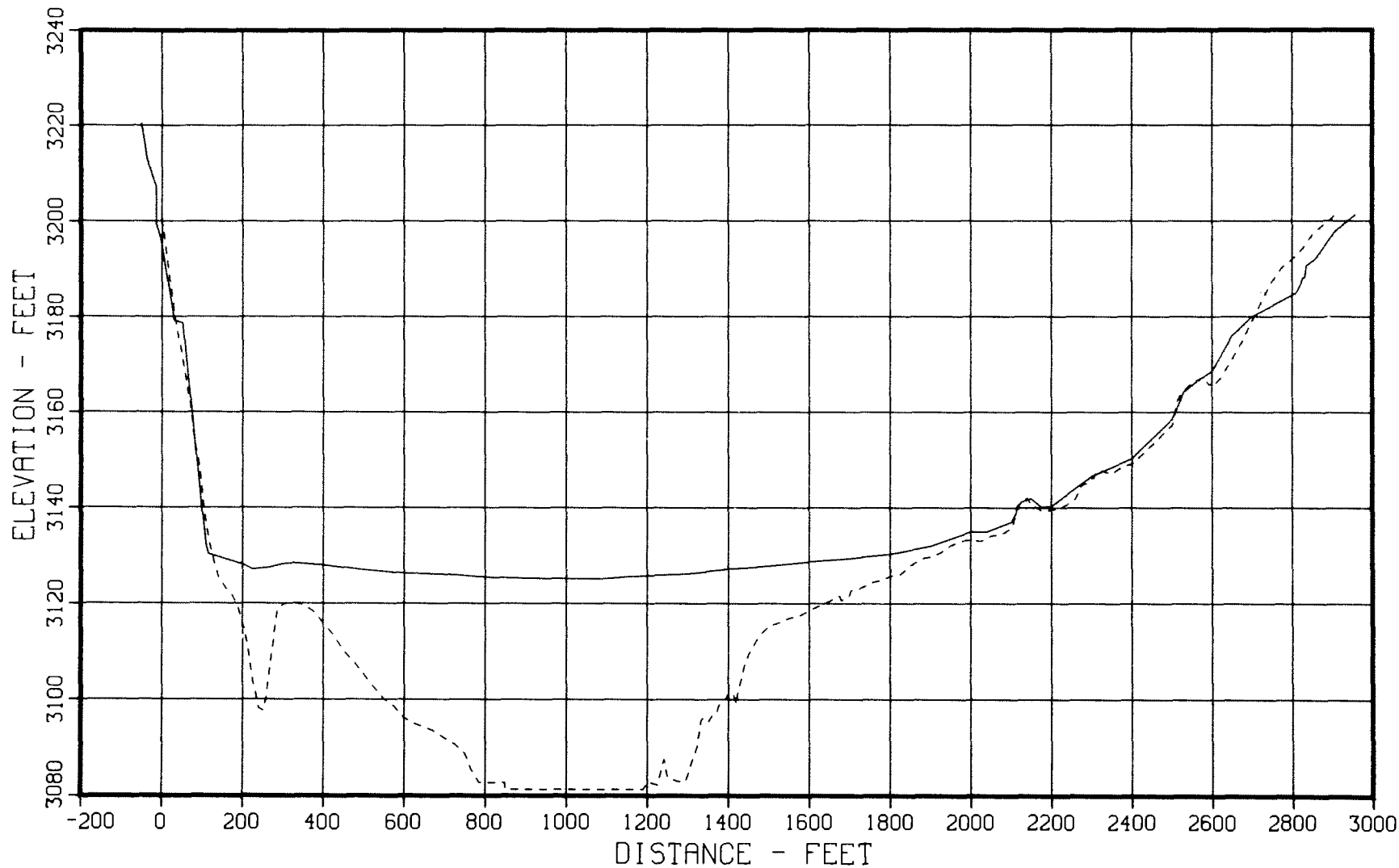
Figure 19. - 1949 and 1979 sedimentation range profiles, Cheyenne River - Range 2A.
