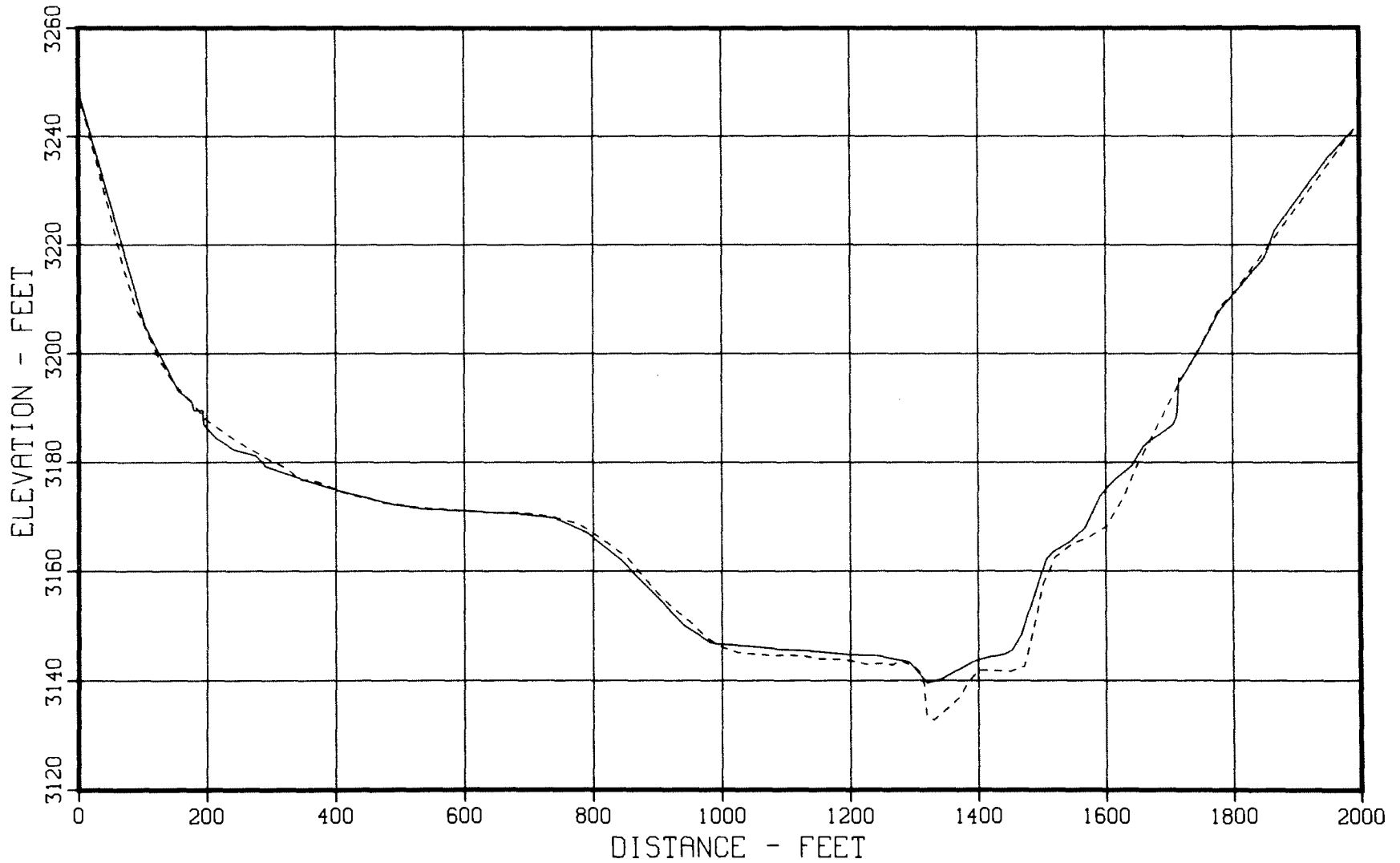
Figure 46. - 1949 and 1979 sedimentation range profiles, Horsehead Creek - Range 41.
