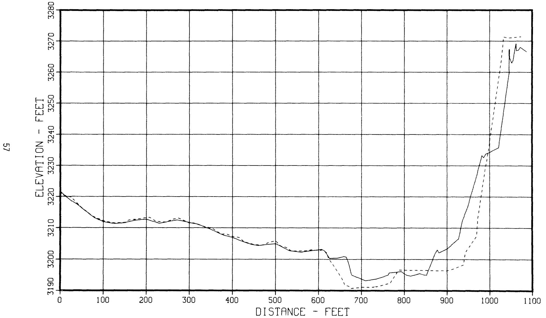
Figure 35. - 1949 and 1979 sedimentation range profiles, Cheyenne River - Range 15.
