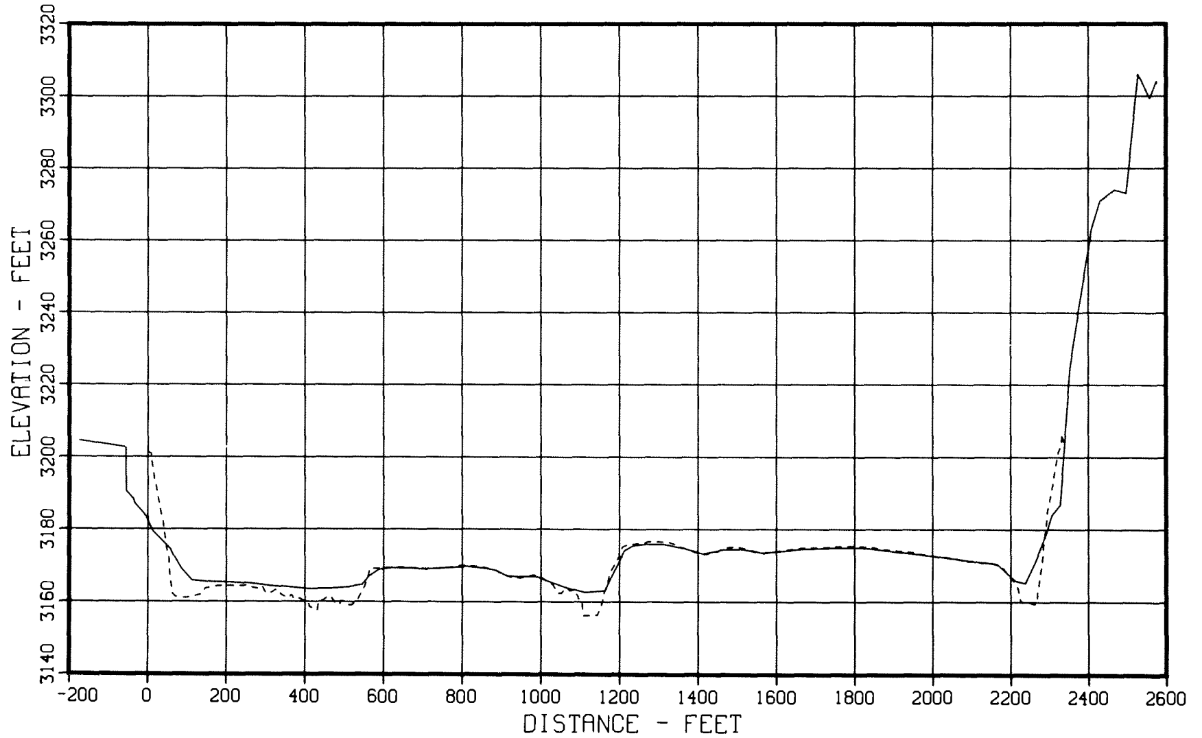
Figure 49. - 1949 and 1979 sedimentation range profiles, Horsehead Creek - Range 44.
