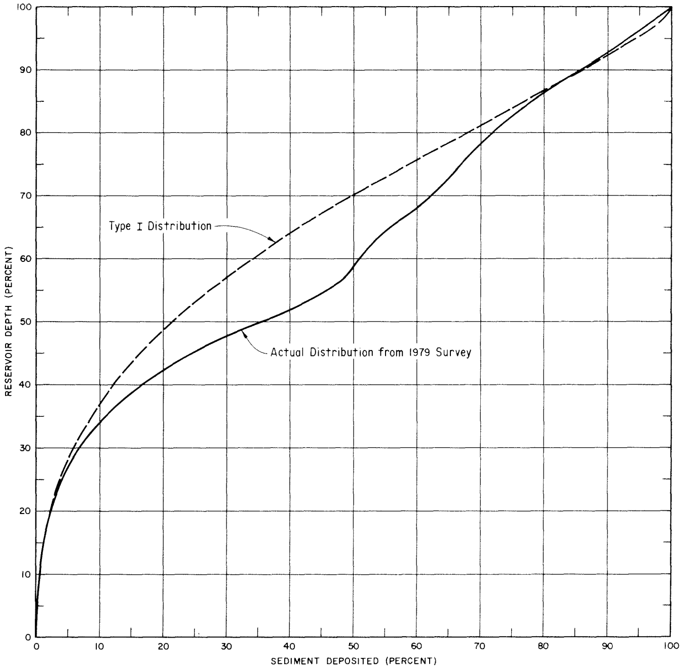
Figure 15. - Sediment distribution curves.
