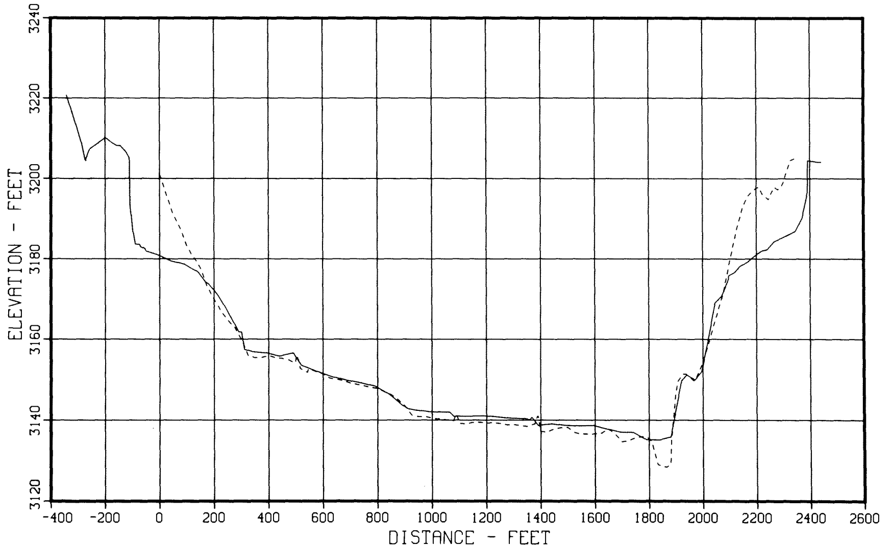
Figure 45. - 1949 and 1979 sedimentation range profiles, Horsehead Creek - Range 40.
