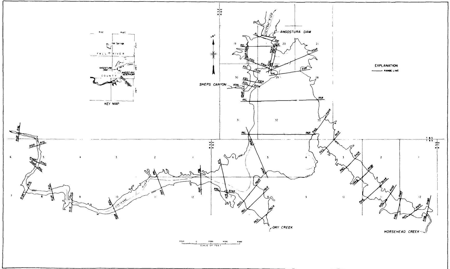
Figure 7. - Layout of reservoir sedimentation ranges.
