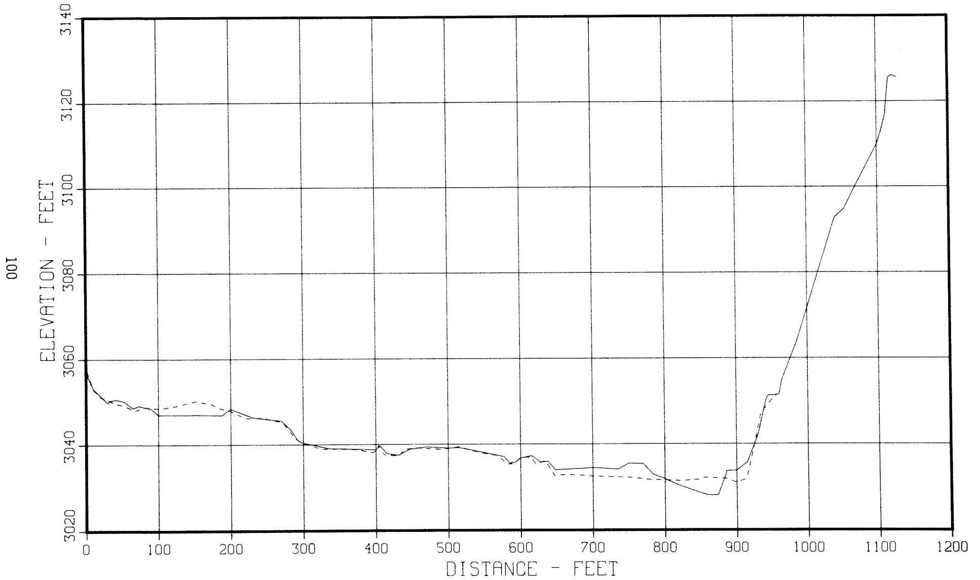
Figure 77. - Degradation range profiles - Range 5.0.
