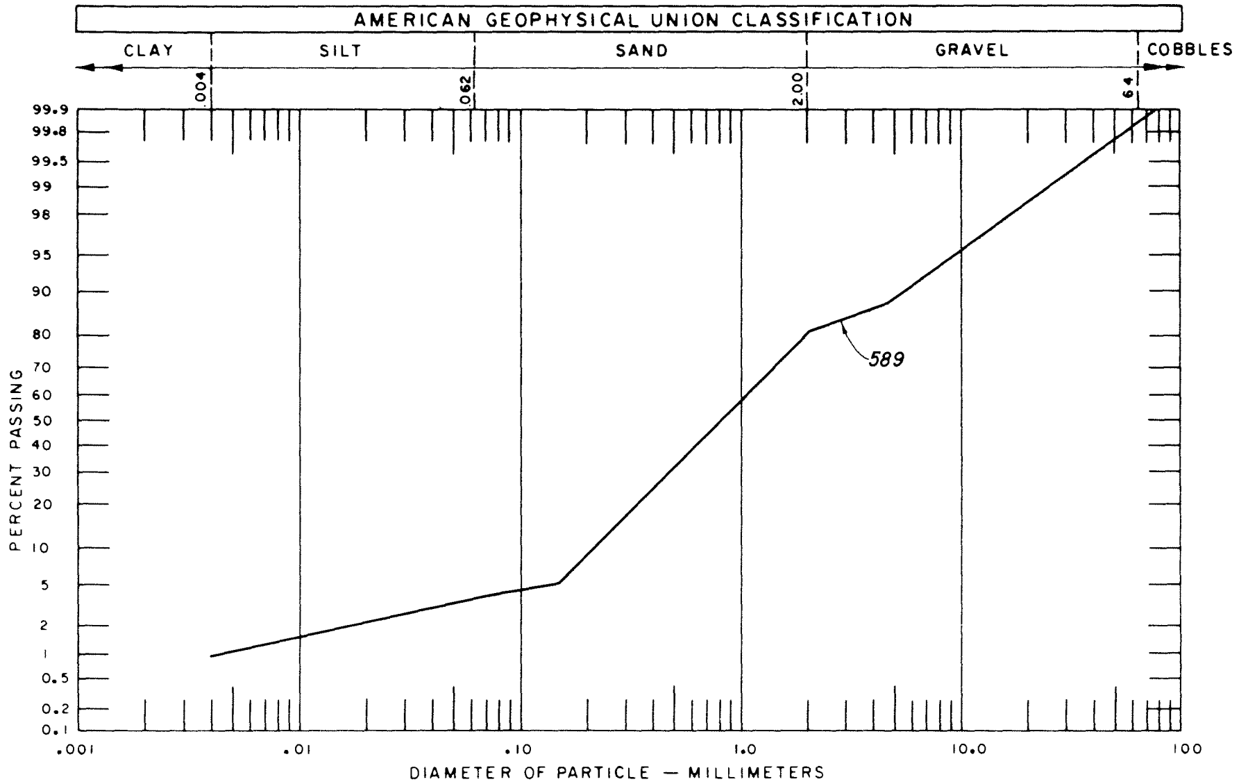
Figure 70. - Particle size analyses curve - Range 14.
