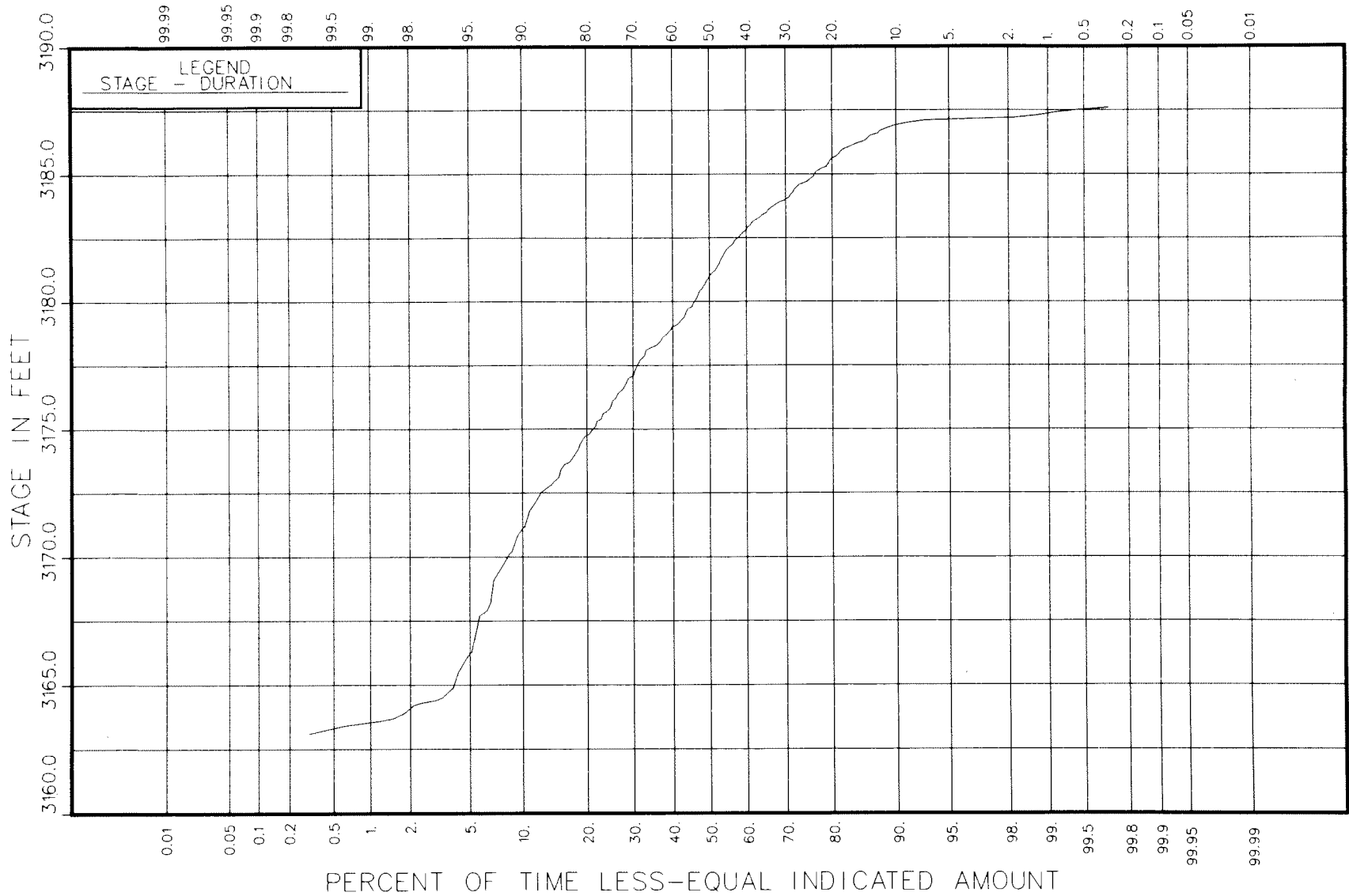
Figure 16. - Stage-duration curve for end-of-month elevations.
