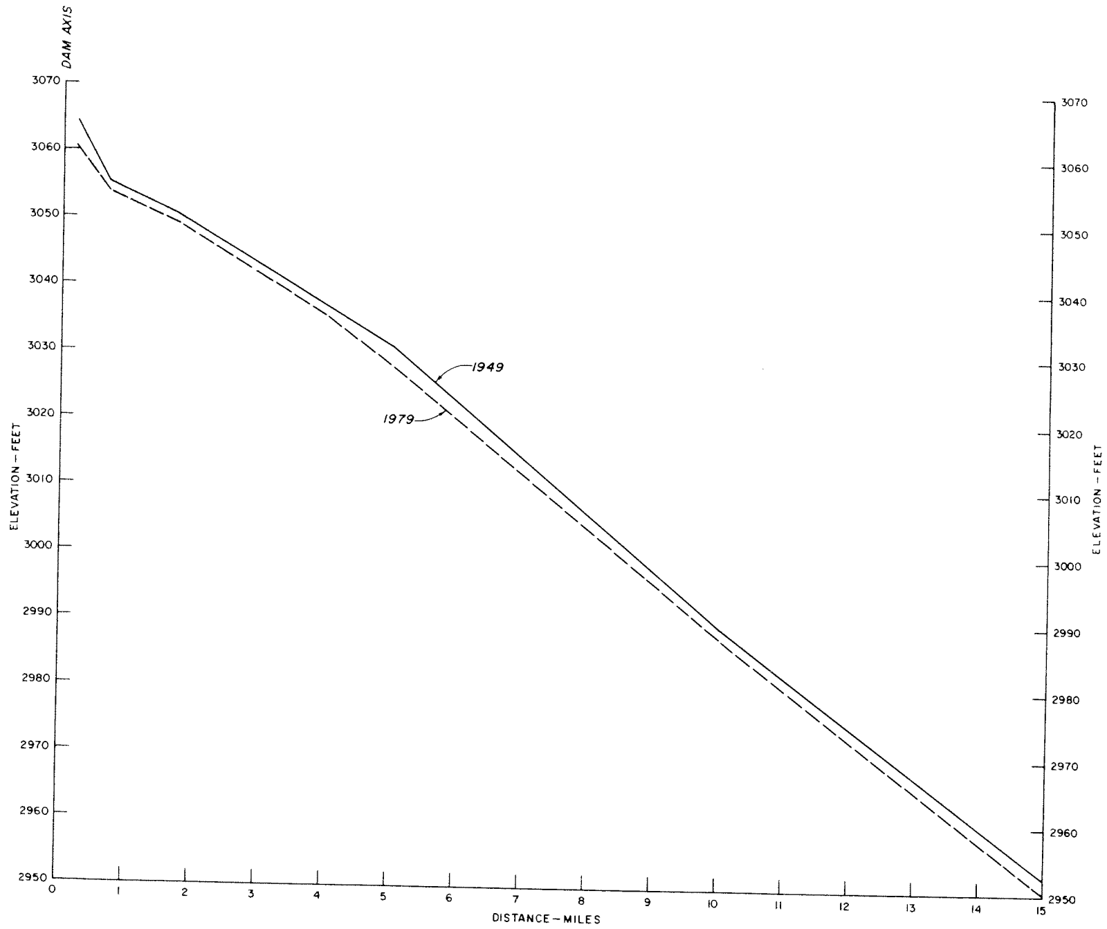
Figure 80. - Longitudinal degradation profiles.
