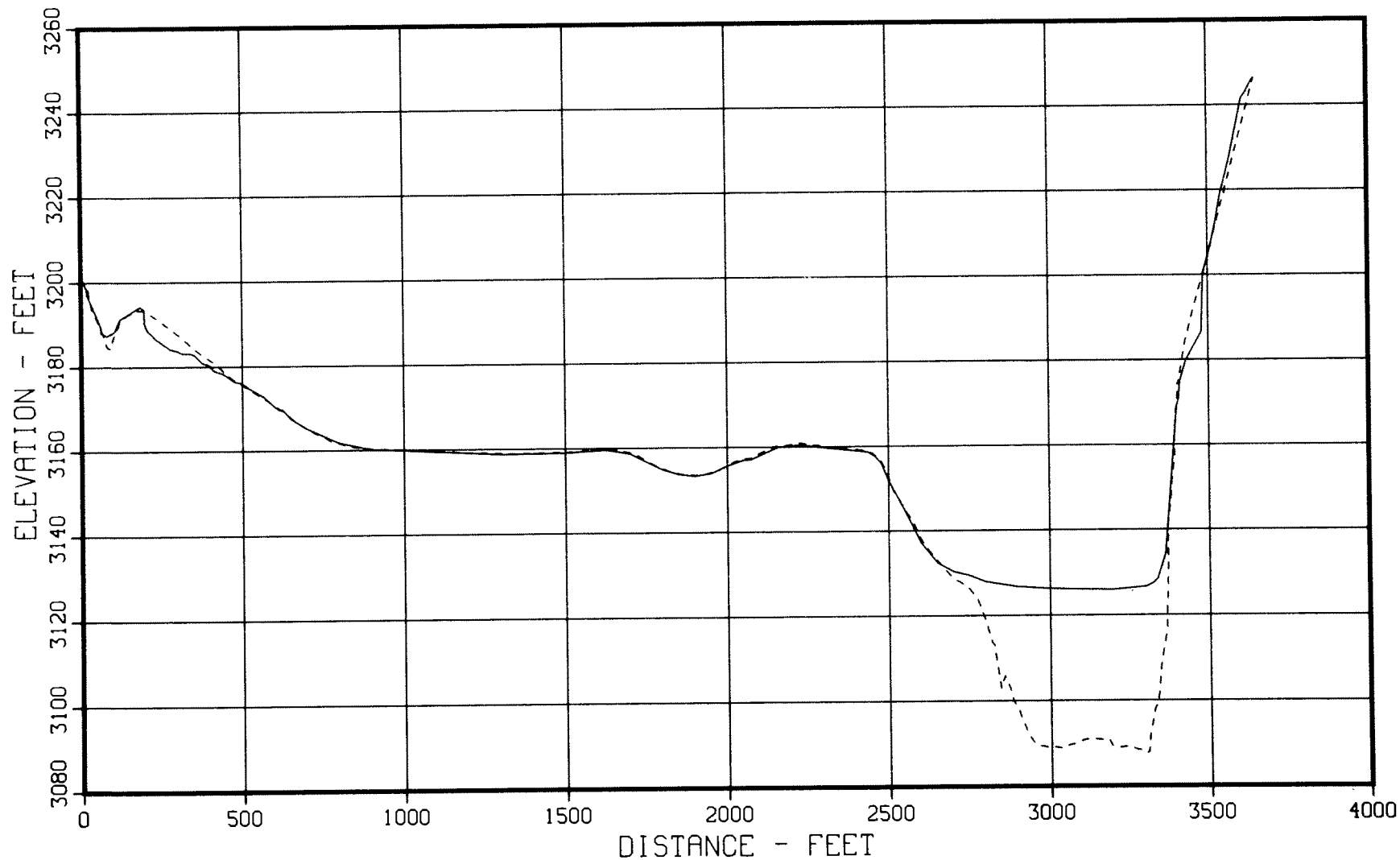
Figure 22. - 1949 and 1979 sedimentation range profiles, Cheyenne River - Range 4.
