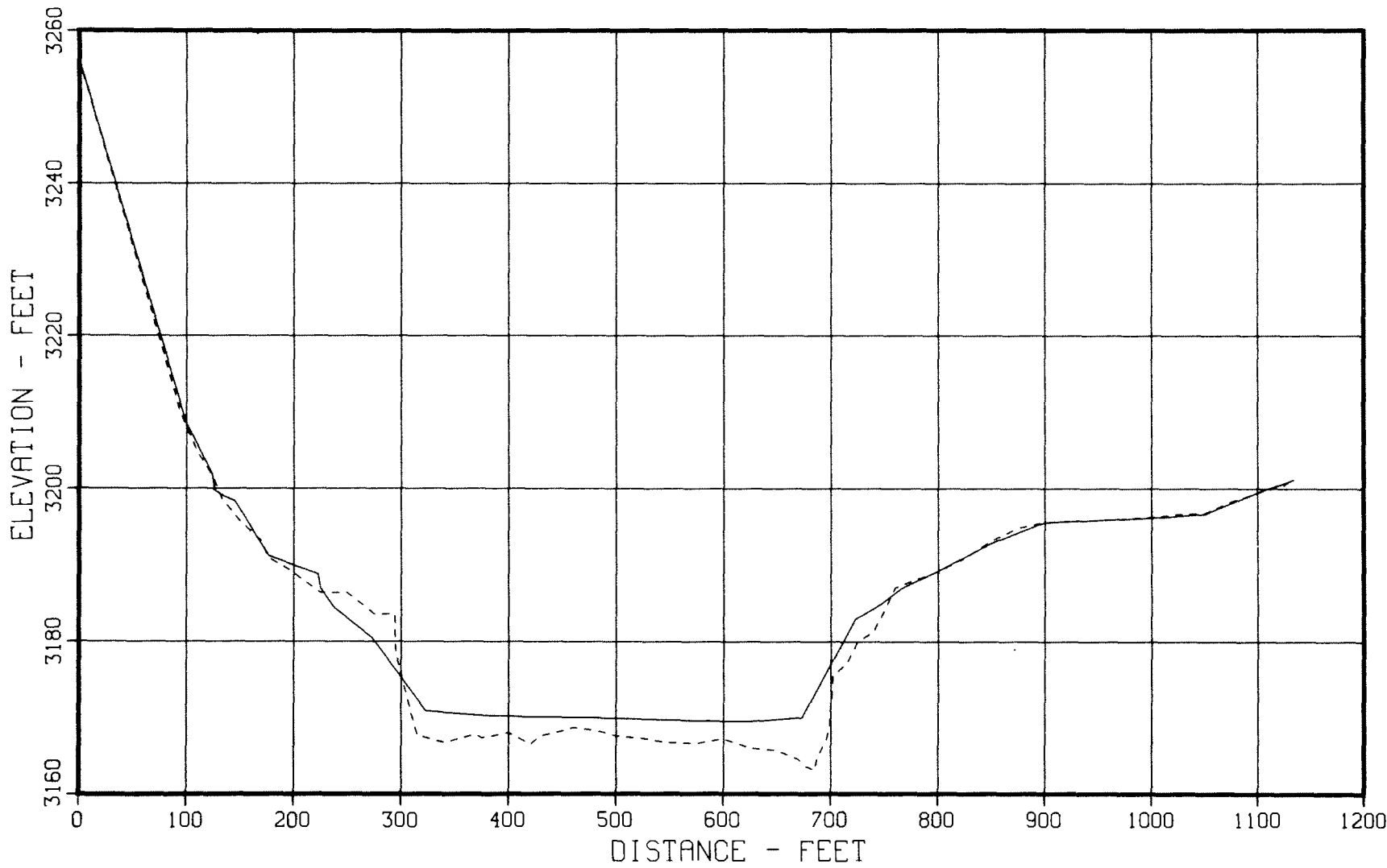
Figure 50. - 1949 and 1979 sedimentation range profiles, Horsehead Creek - Range 45.
