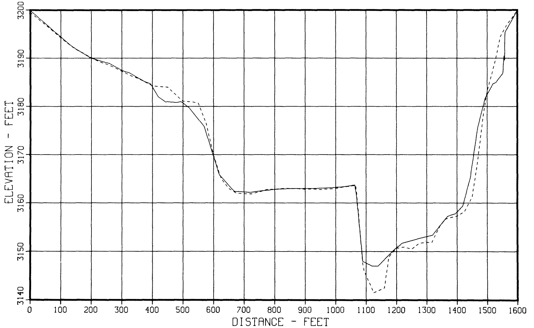
Figure 47. - 1949 and 1979 sedimentation range profiles, Horsehead Creek - Range 42.
