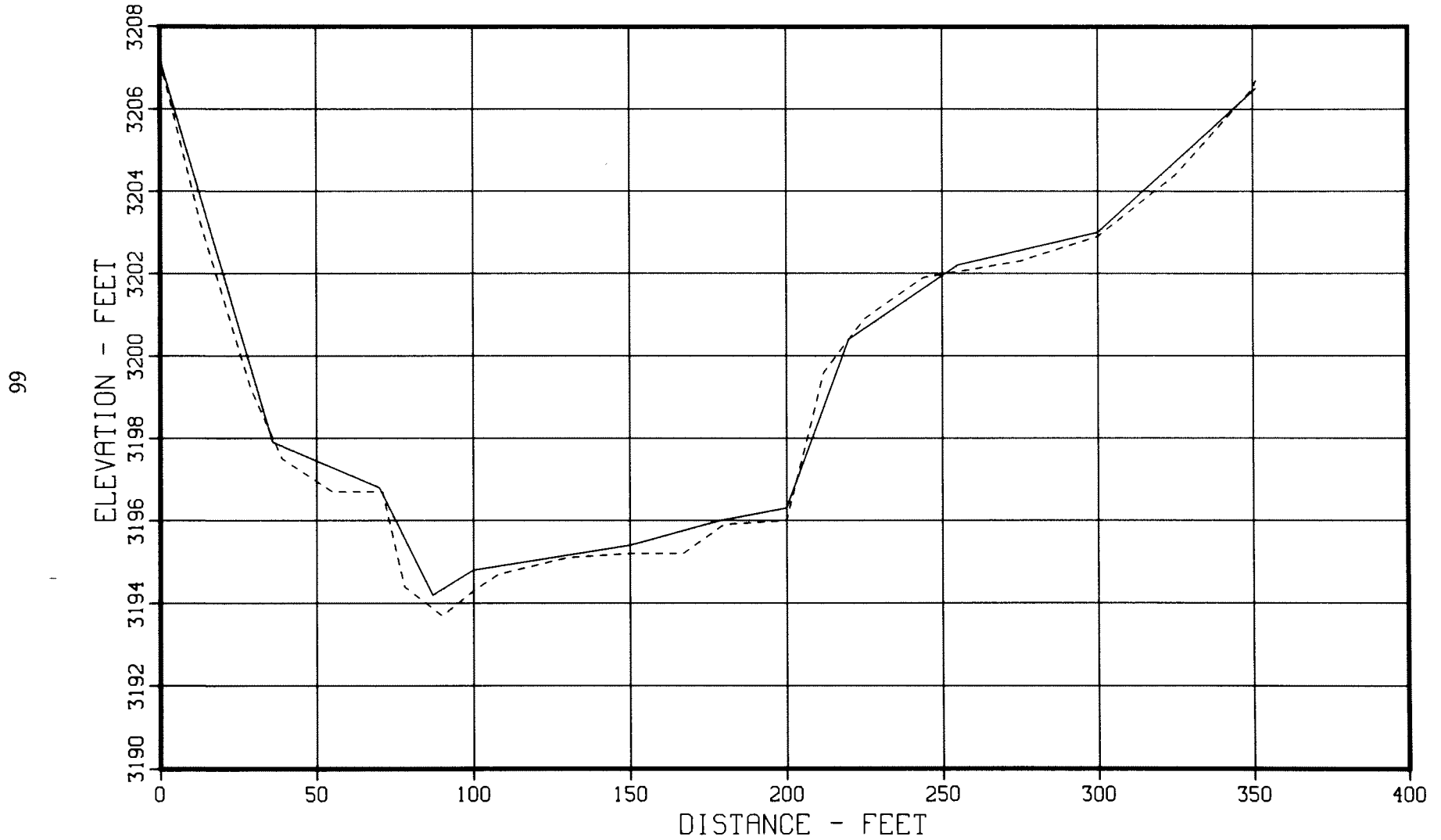
Figure 44. - 1949 and 1979 sedimentation range profiles, Sheps Canyon - Range 34.
