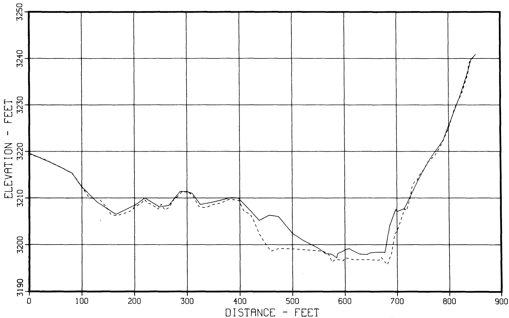
Figure 36. - 1949 and 1979 sedimentation range profiles, Cheyenne River - Range 16.
