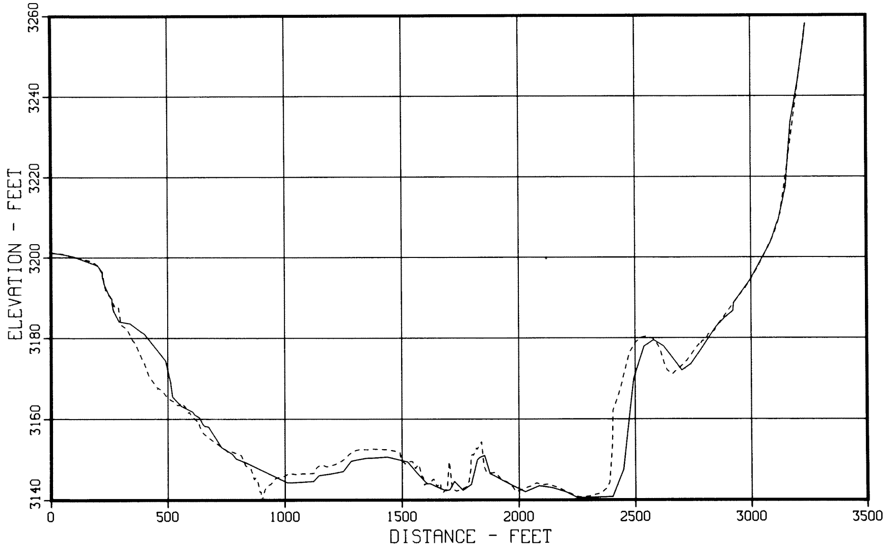
Figure 40. - 1949 and 1979 sedimentation range profiles, Sheps Canyon, Range 30.
