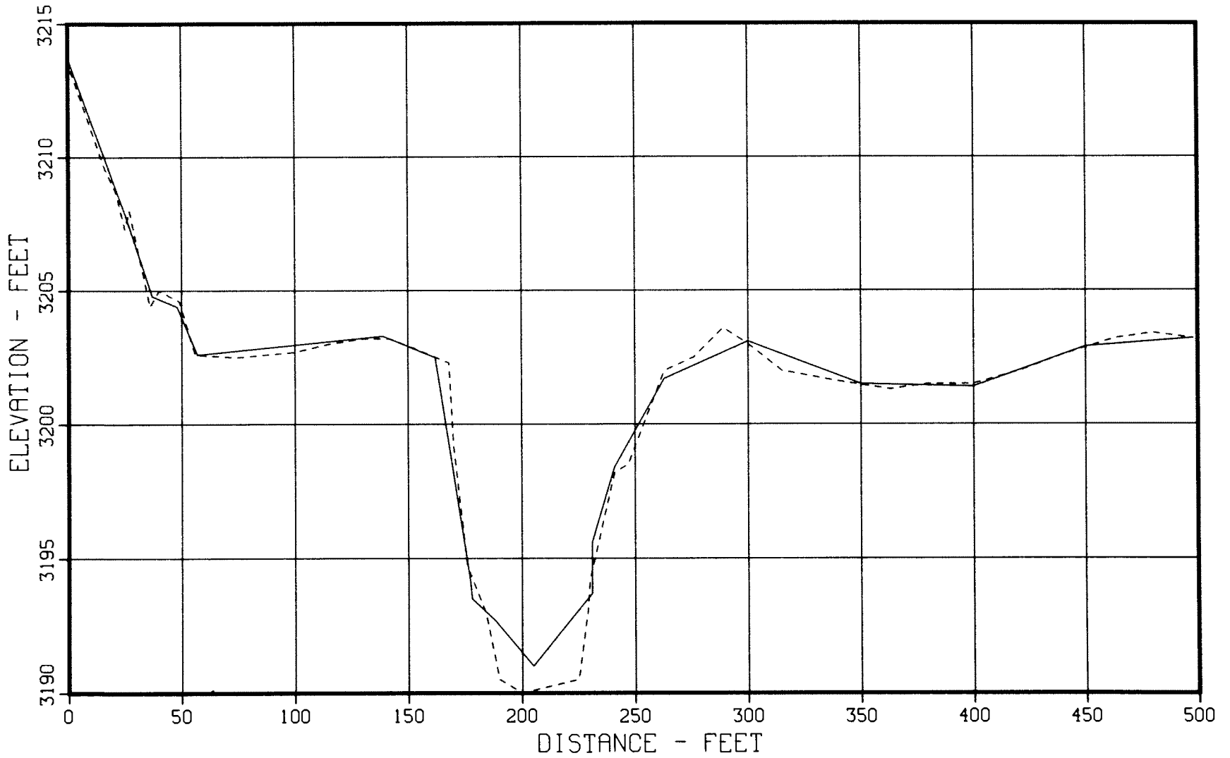
Figure 54. - 1949 and 1979 sedimentation range profiles, Horsehead Creek - Range 48A.
