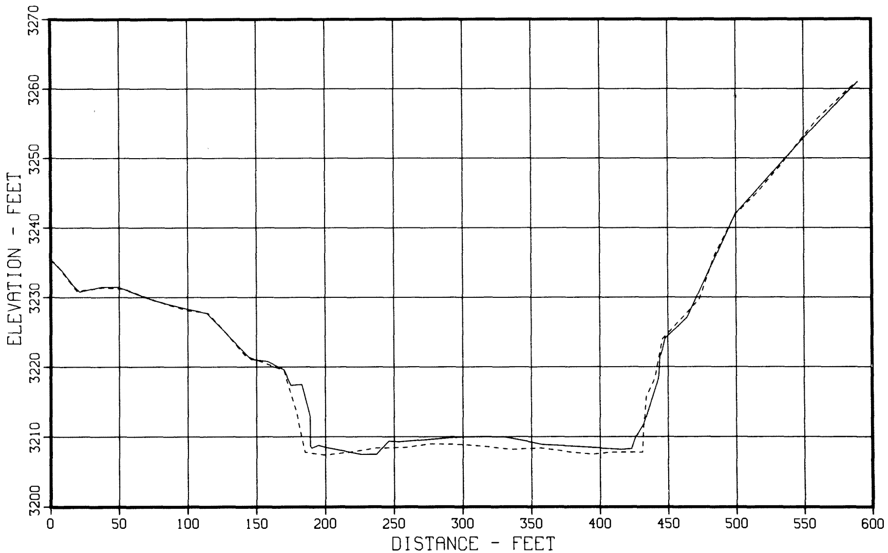
Figure 38. - 1949 and 1979 sedimentation range profiles, Cheyenne River - Range 18.
