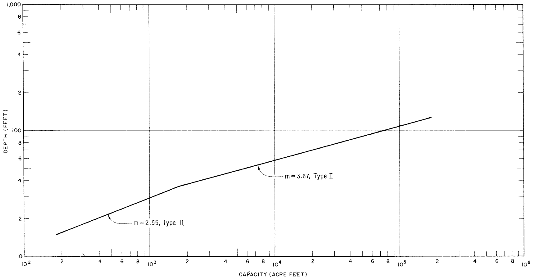
Figure 14. - Depth-capacity relationship.
