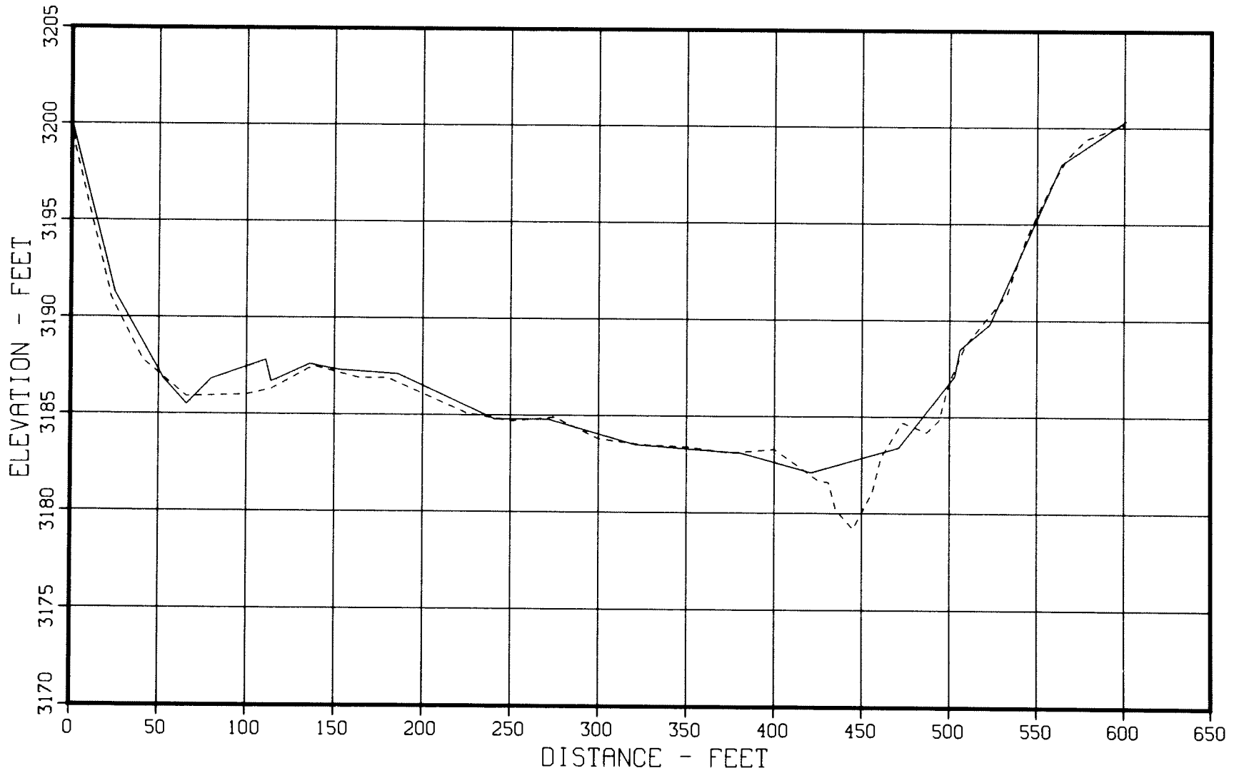
Figure 43. - 1949 and 1979 sedimentation range profiles, Sheps Canyon - Range 33.
