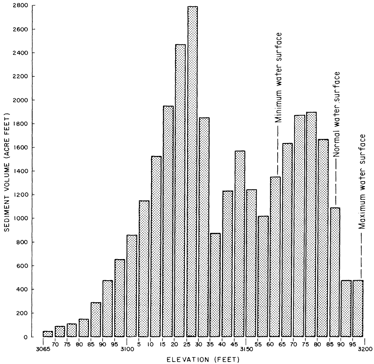
Figure 62. - Sediment accumulations in elevation intervals.
