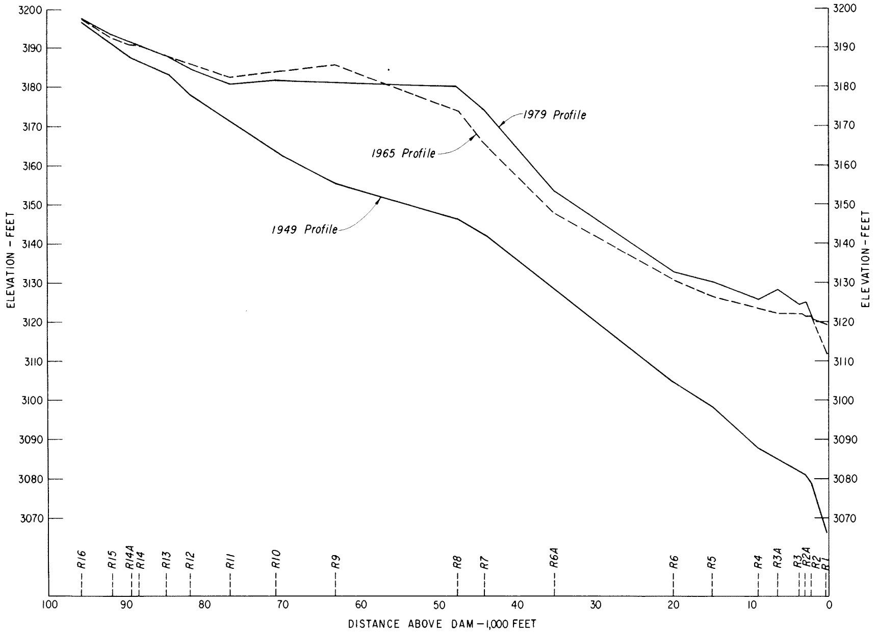
Figure 10. - Longitudinal profiles for Cheyenne River.
