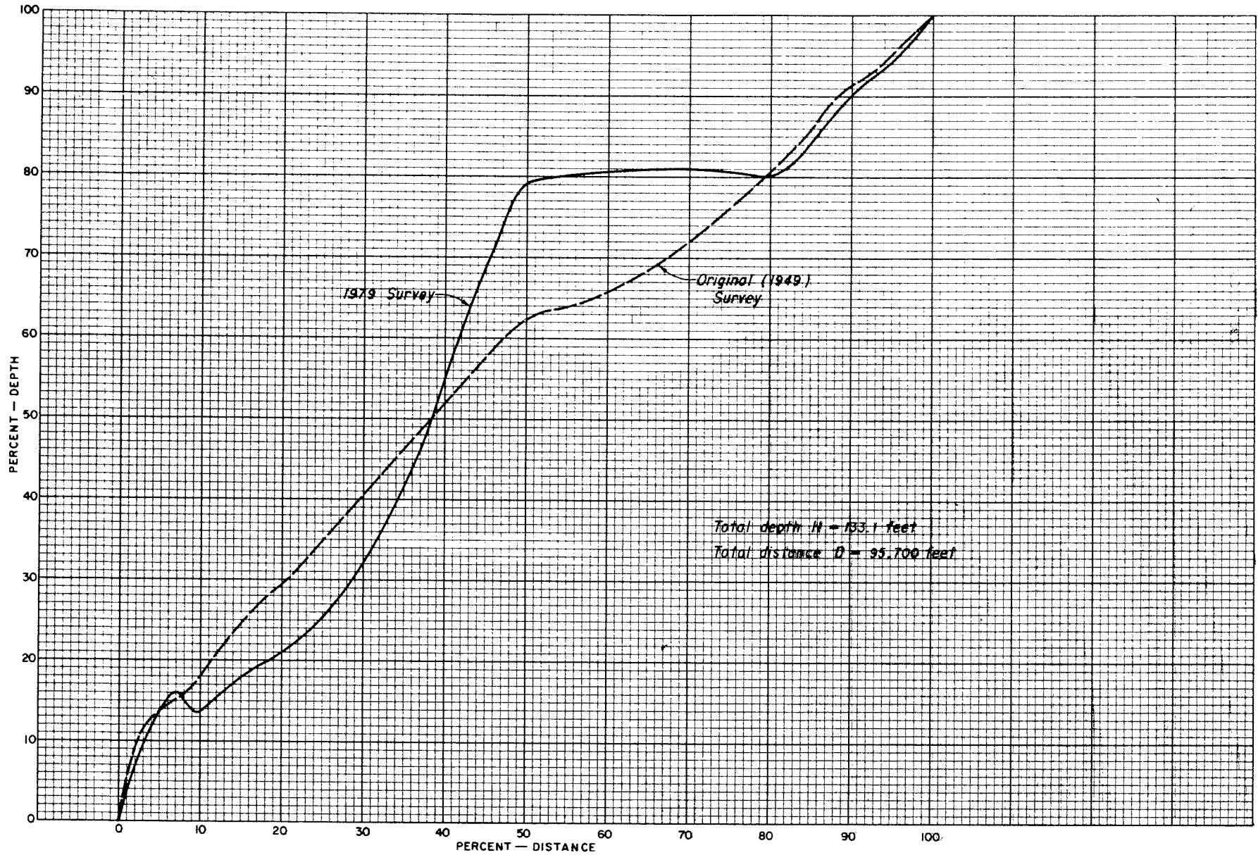
Figure 12. - Percent depth-percent distance relationship for Cheyenne River above Angostura Dam.
