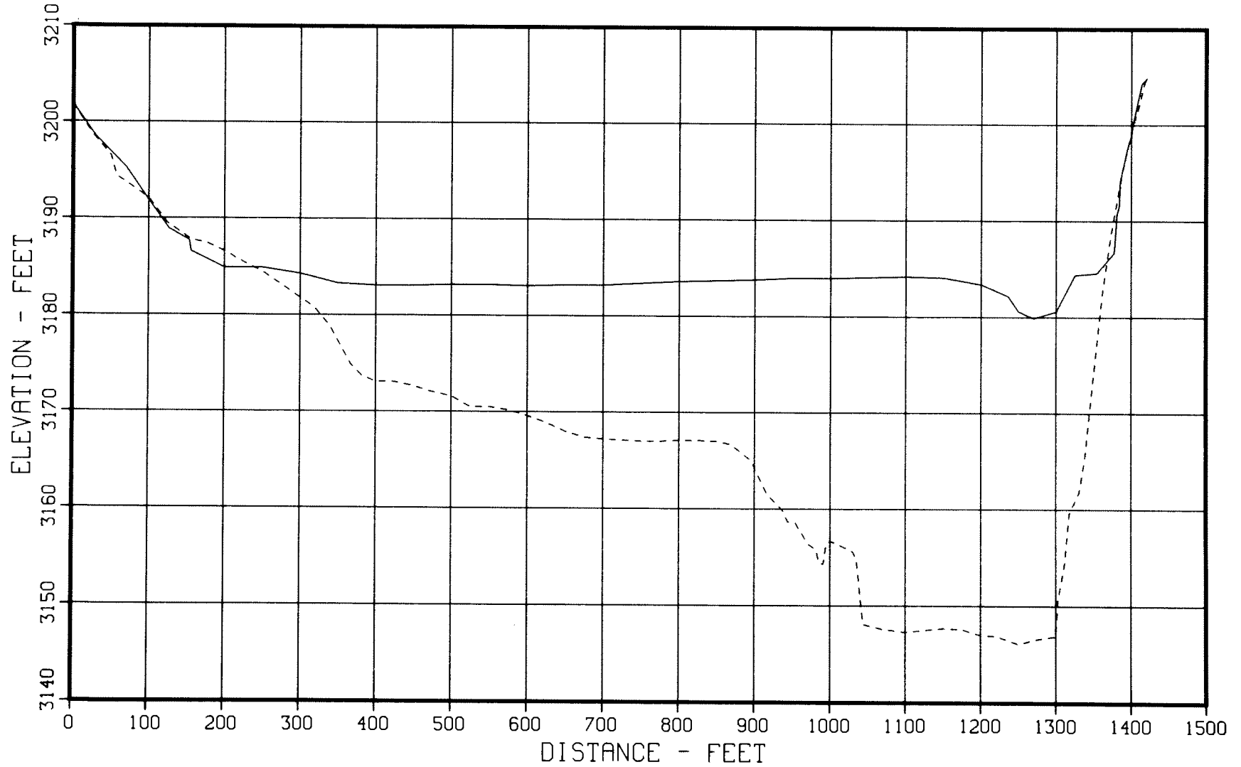
Figure 27. - 1949 and 1979 sedimentation range profiles, Cheyenne River - Range 8.
