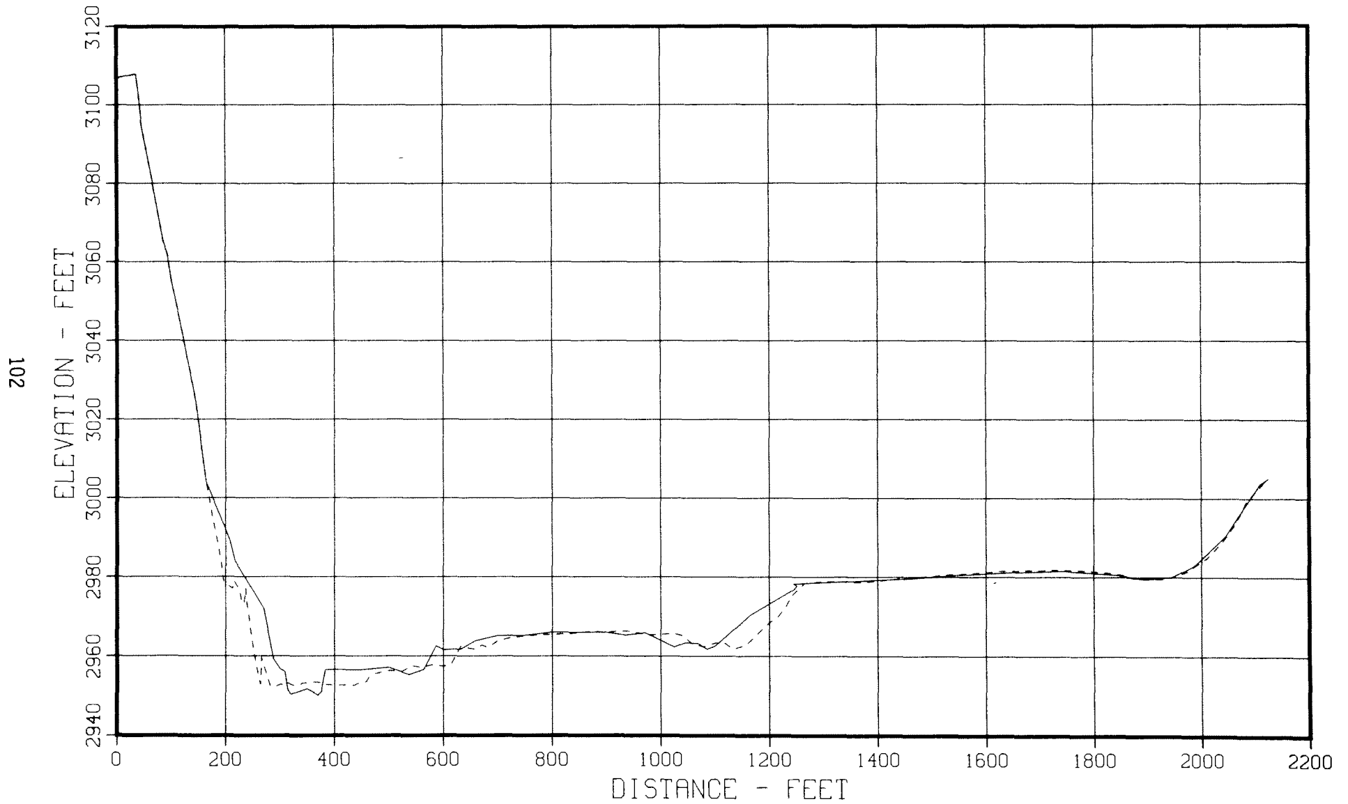
Figure 79. - Degradation range profiles - Range 15.0.
