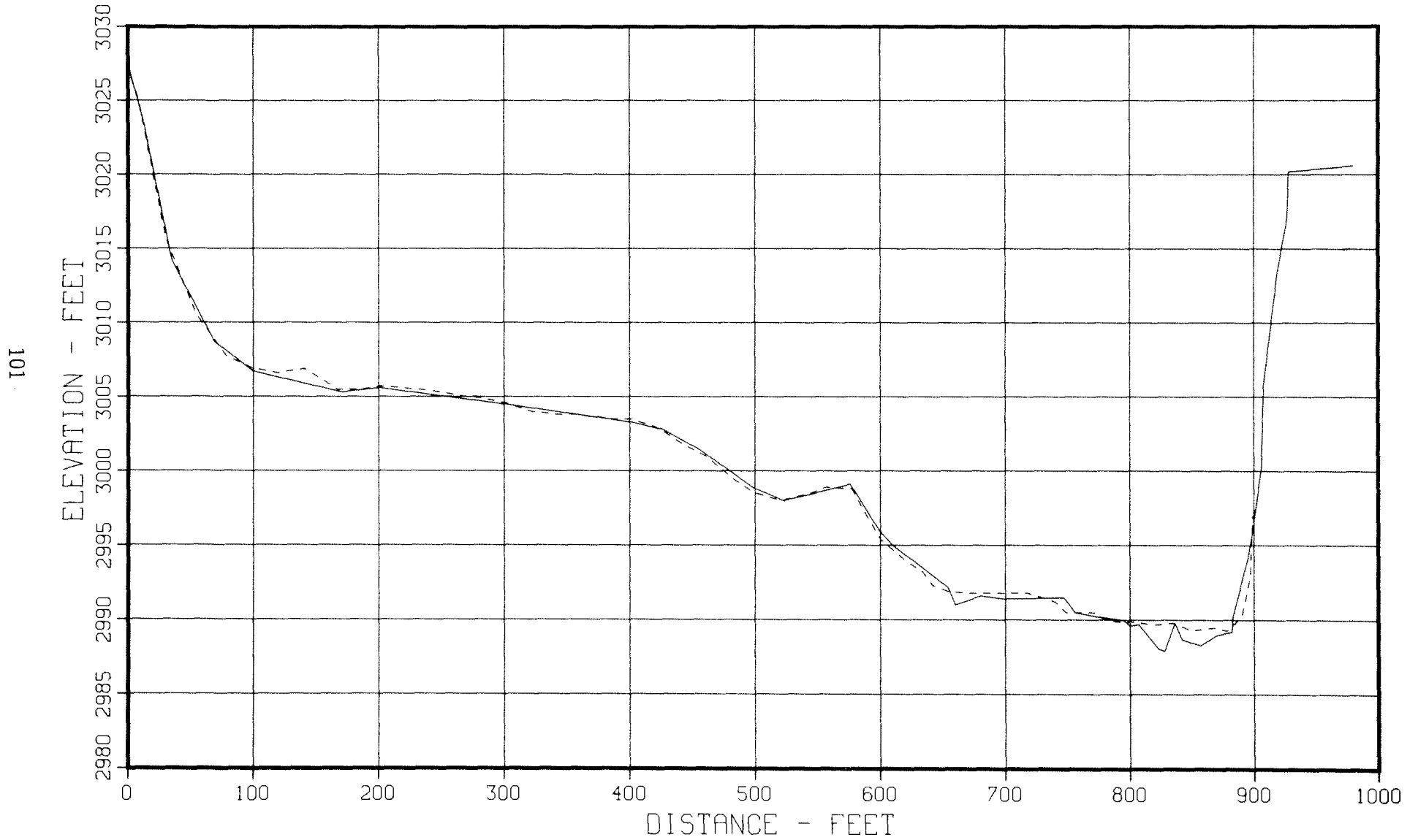
Figure 78. - Degradation range profiles - Range 10.0.
