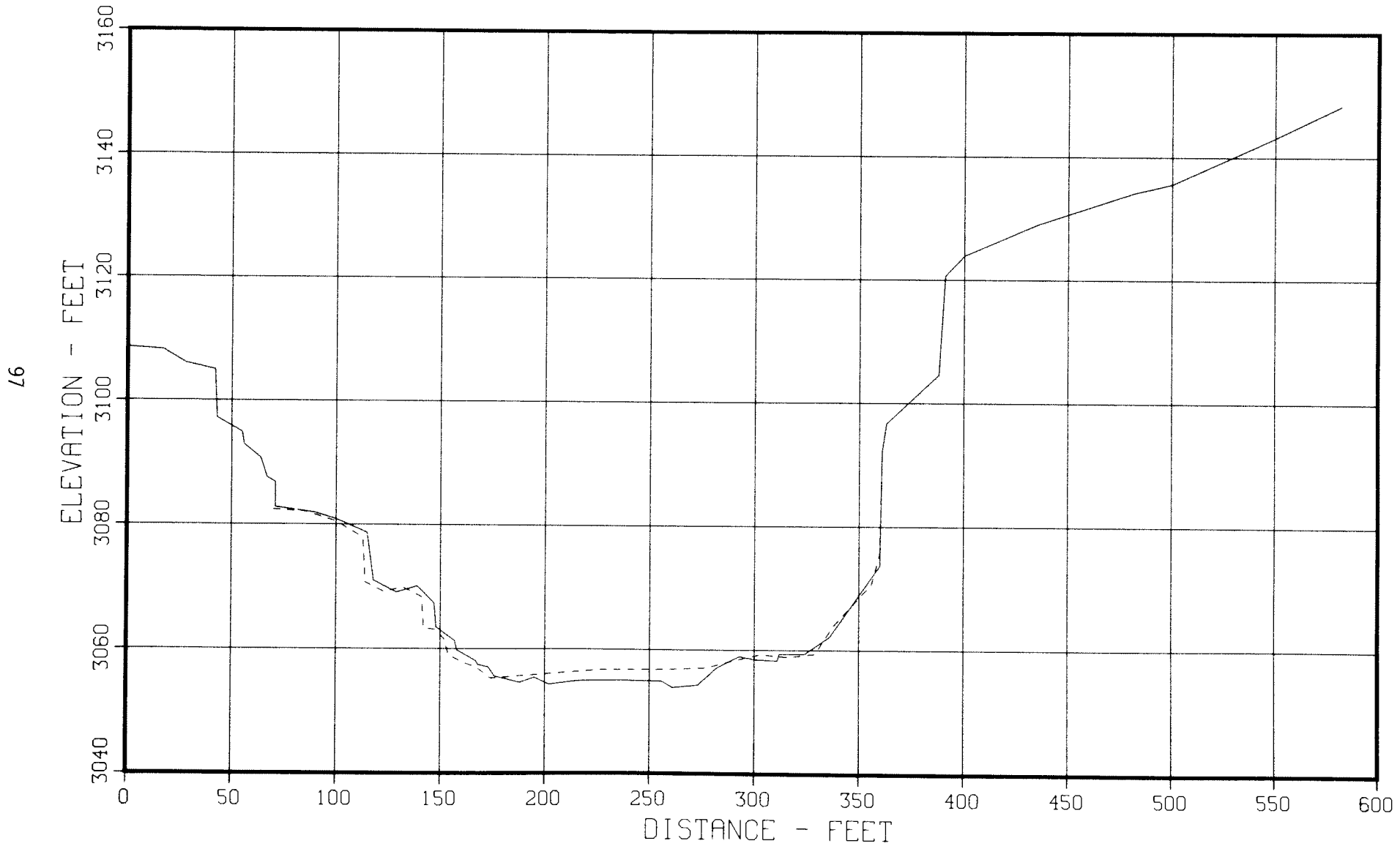
Figure 74. - Degradation range profiles - Range 0.7.
