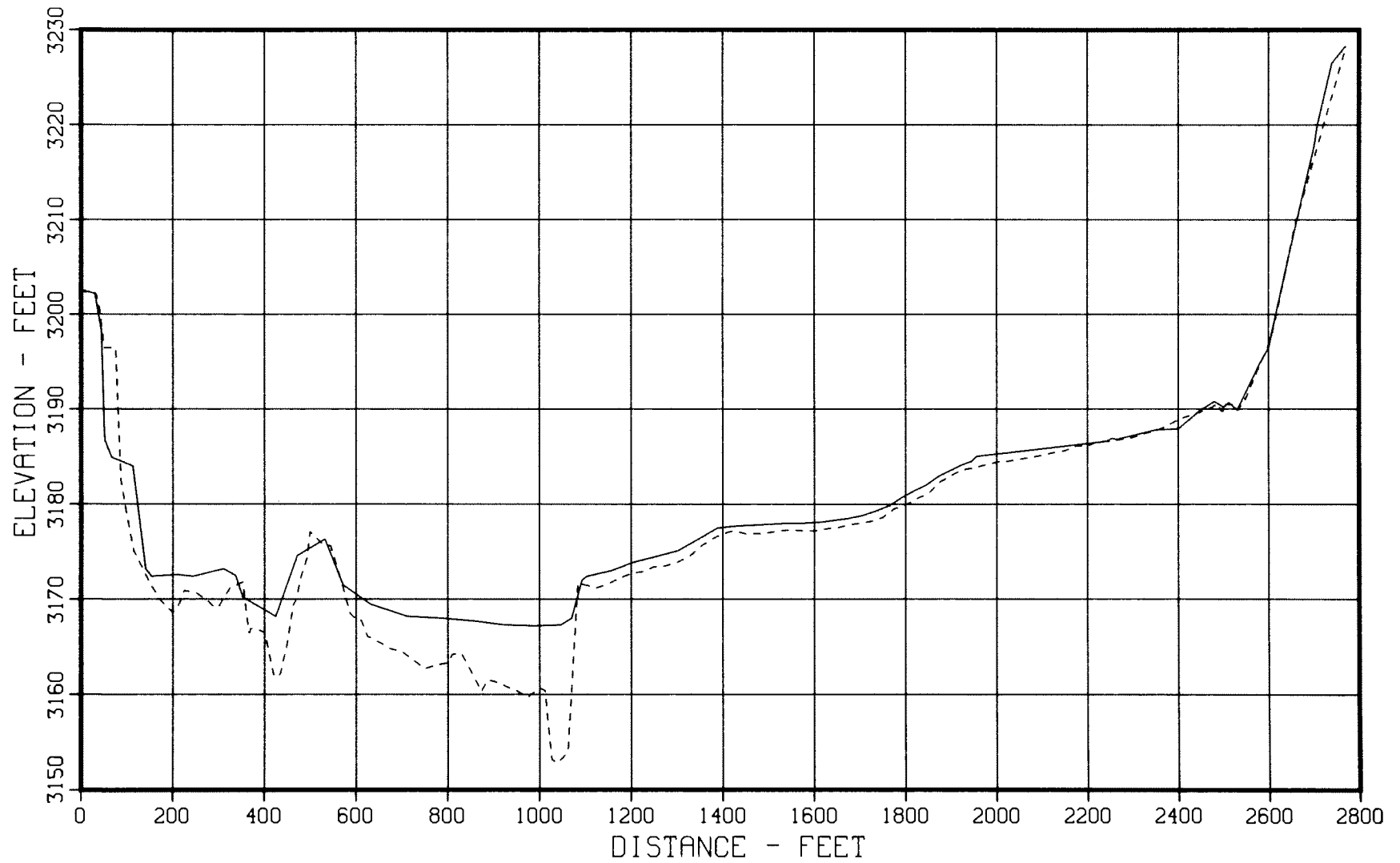
Figure 58. - 1949 and 1979 sedimentation range profiles, Dry Creek - Range 61.
