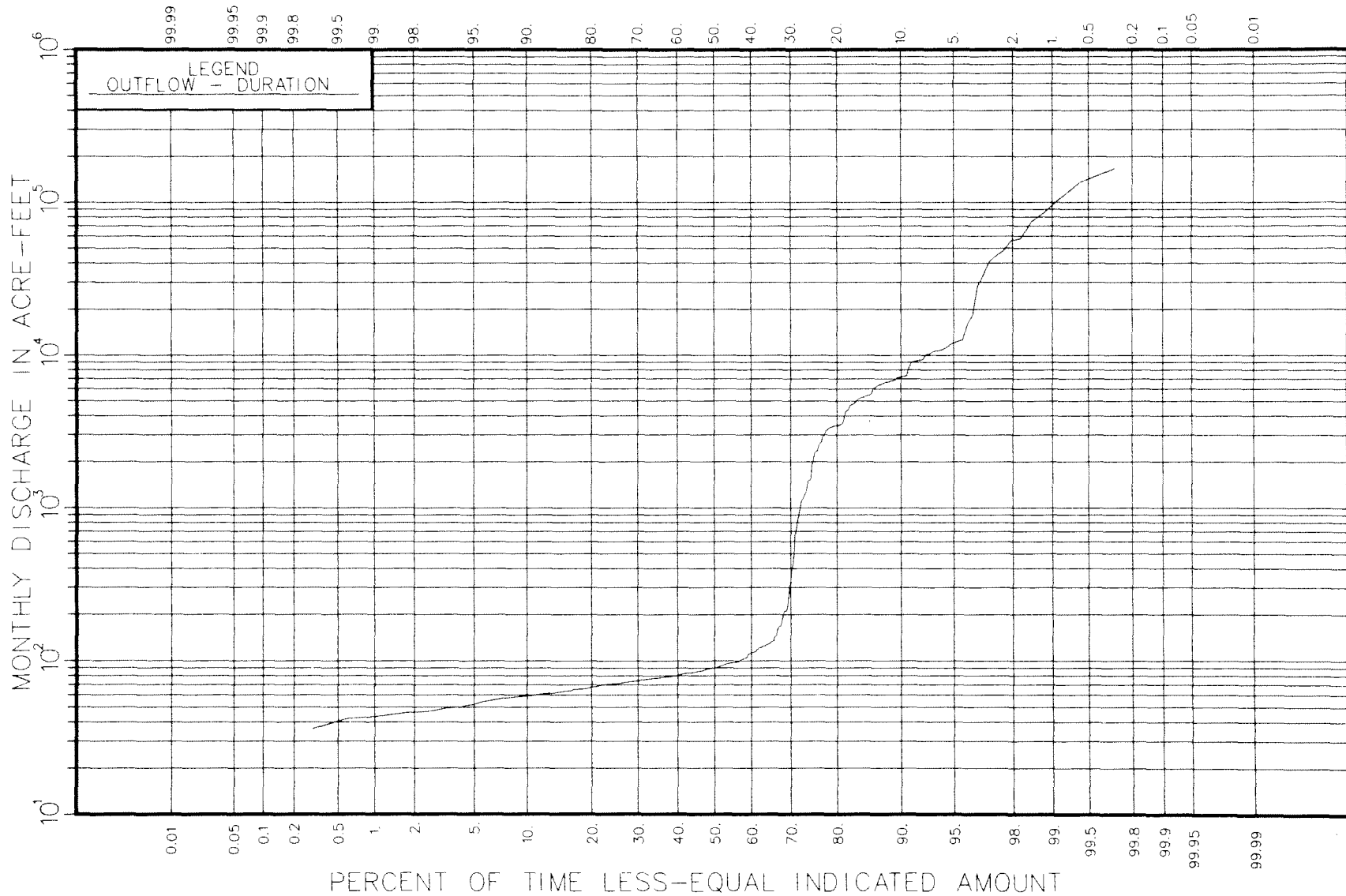
Figure 81. - Outflow duration curve for monthly outflow discharges.
