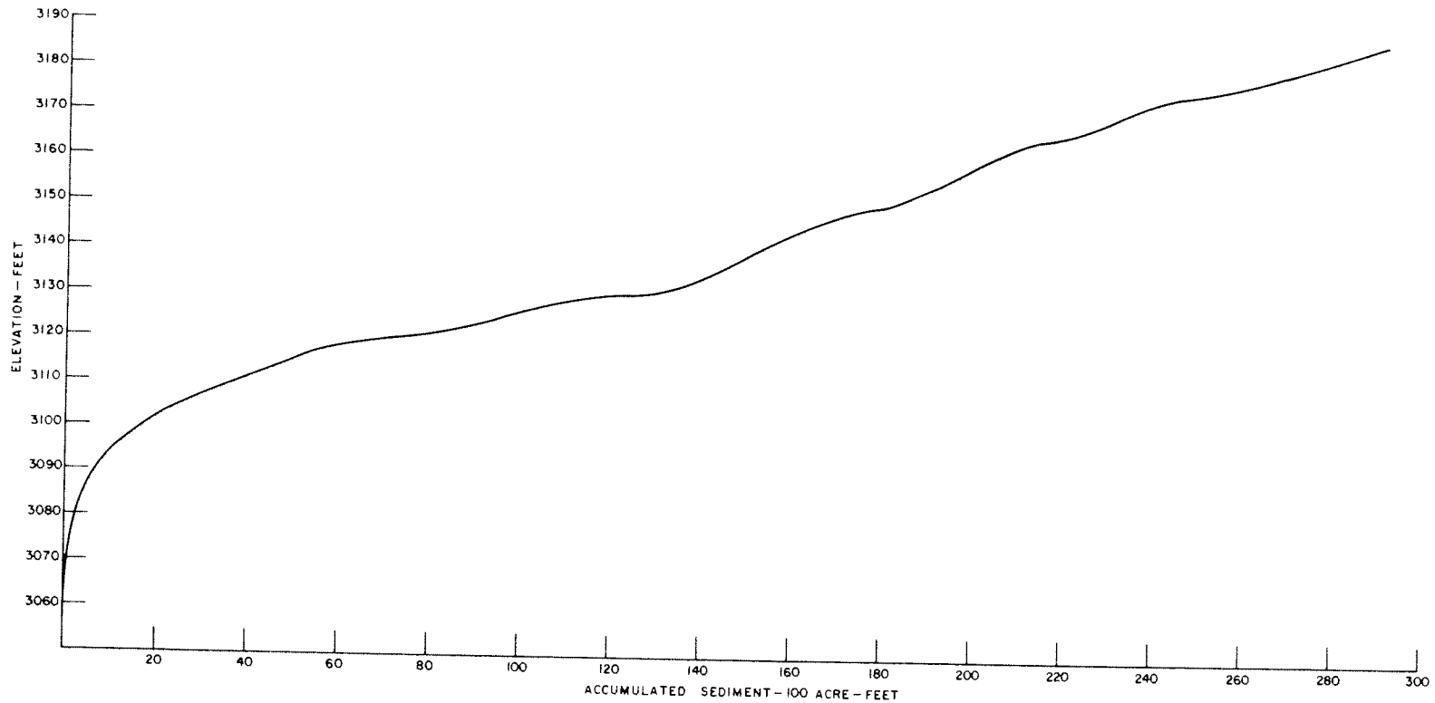
Figure 61. - Sediment accumulation curve.
