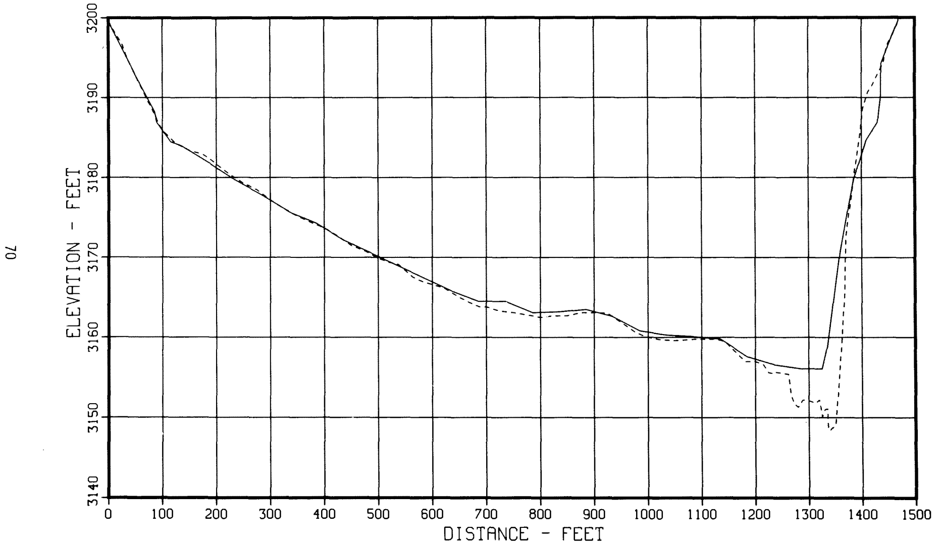
Figure 48. - 1949 and 1979 sedimentation range profiles, Horsehead Creek - Range 43.
