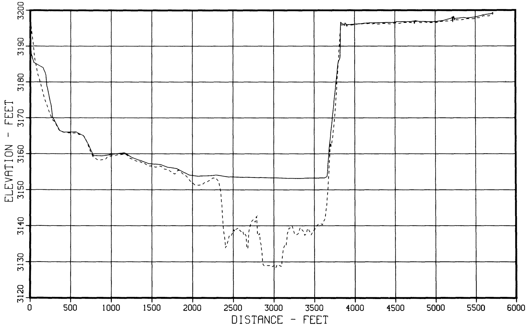
Figure 25. - 1949 and 1979 sedimentation range profiles, Cheyenne River - Range 6A.
