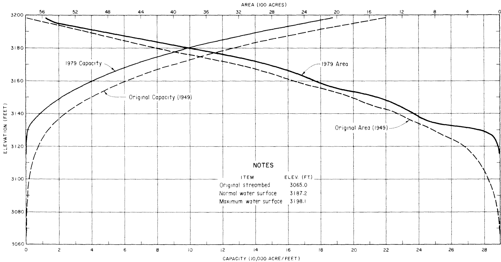
Figure 82. - Area-capacity curves for Angostura Reservoir.
