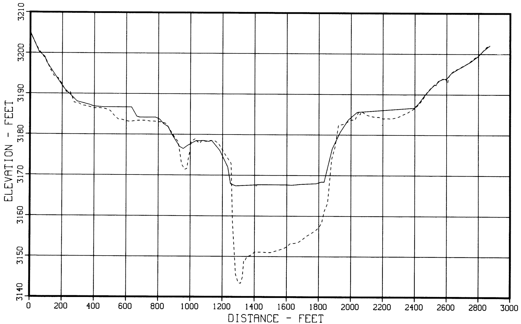
Figure 57. - 1949 and 1979 sedimentation range profiles, Dry Creek - Range 60.
