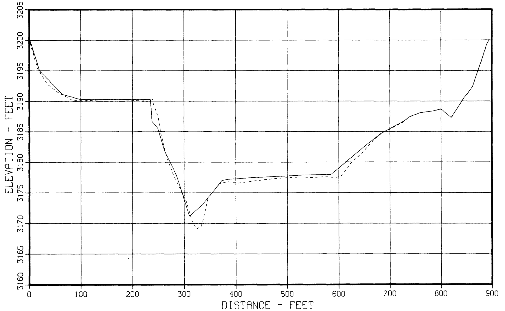
Figure 42. - 1949 and 1979 sedimentation range profiles, Sheps Canyon - Range 32.
