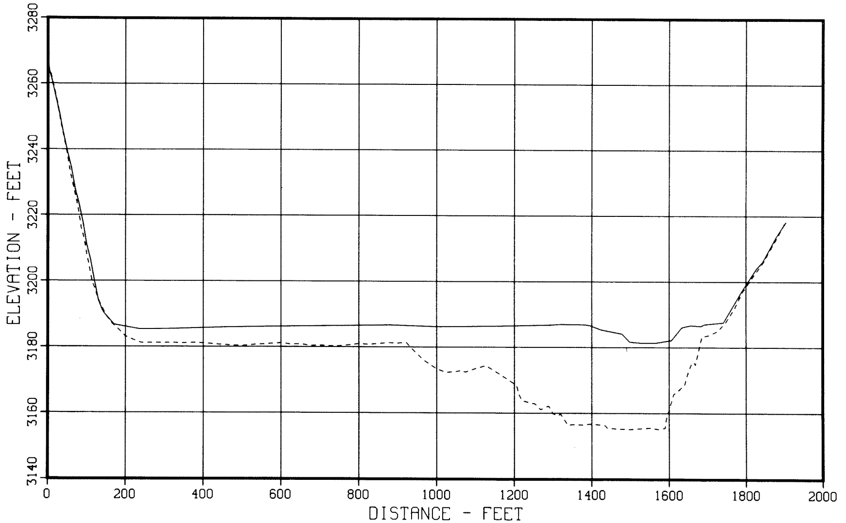
Figure 28. - 1949 and 1979 sedimentation range profiles, Cheyenne River - Range 9.
