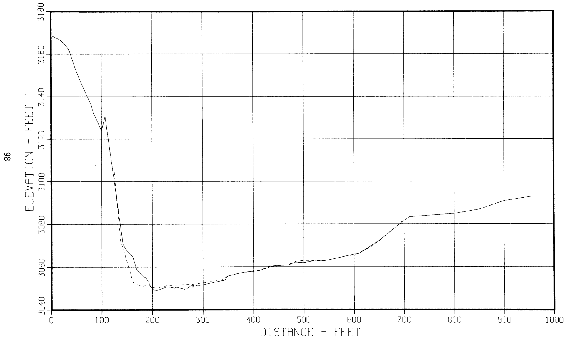
Figure 75. - Degradation range profiles - Range 1.75.
