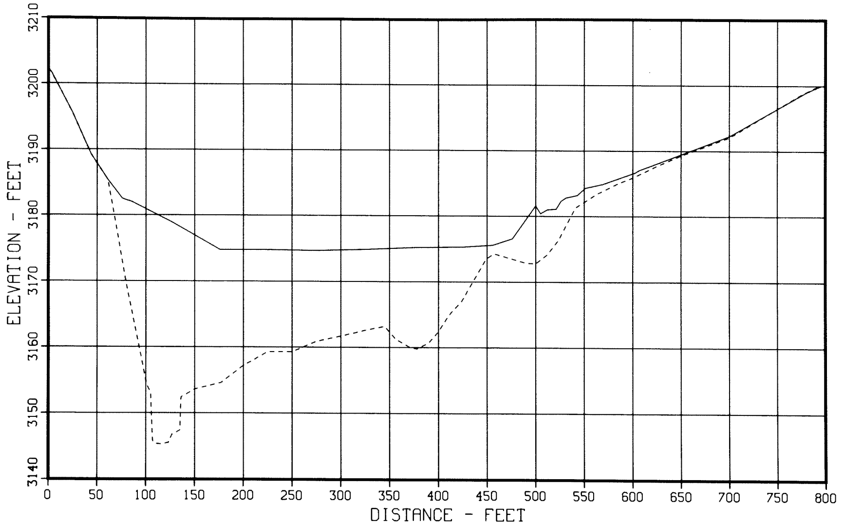
Figure 60. - 1949 and 1979 sedimentation range profiles at mouth of unnamed canyon entering reservoir upstream of Range 7 - Range 7A.
