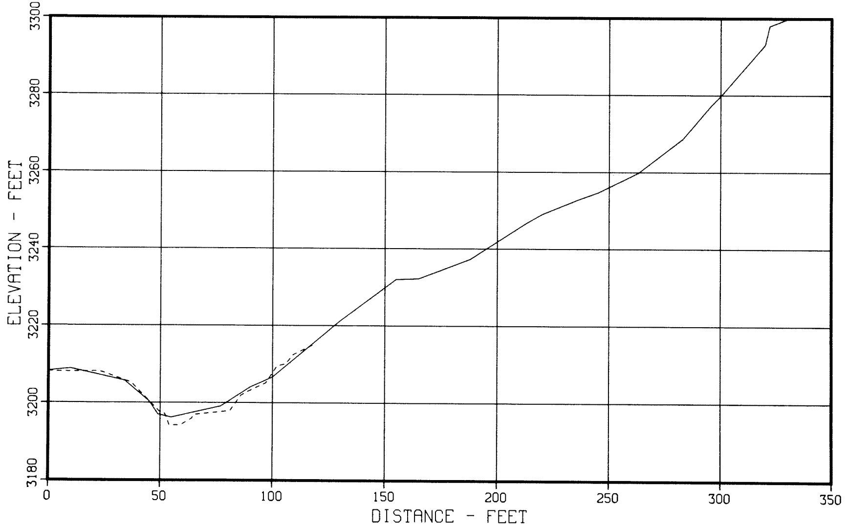
Figure 55. - 1949 and 1979 sedimentation range profiles, Horsehead Creek - Range 49.
