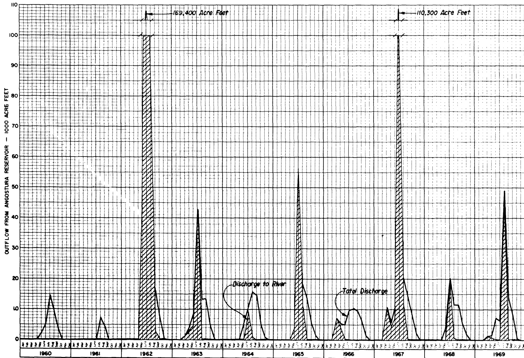
Figure 4. - Monthly outflow from Angostura Reservoir - Sheet 2 of 3.
