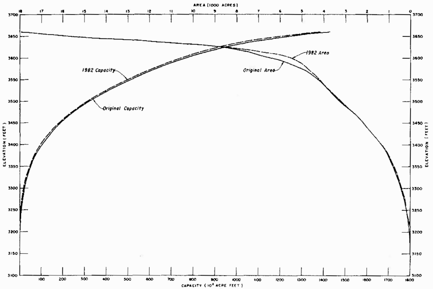
Figure 12. - Area-capacity curve.
