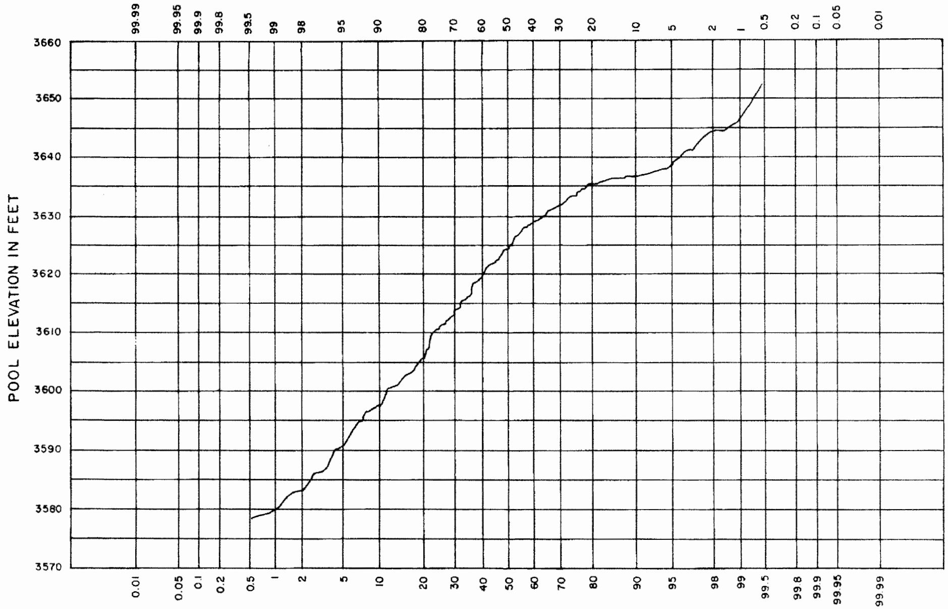
Figure 5. - Reservoir stage duration curve.
