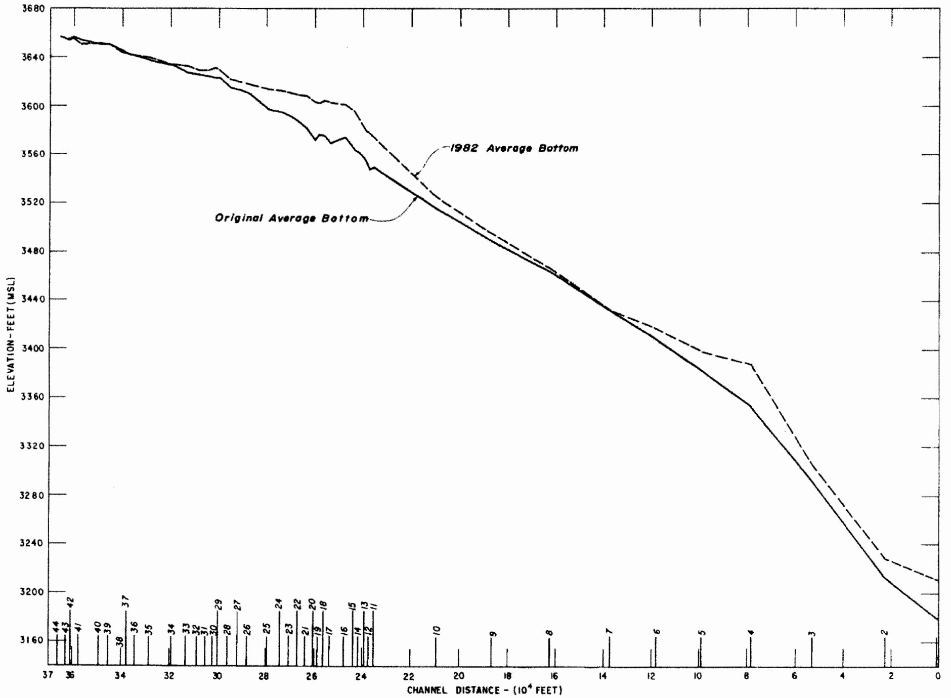
Figure 31. - Average bottom profiles for Bighorn Lake.
