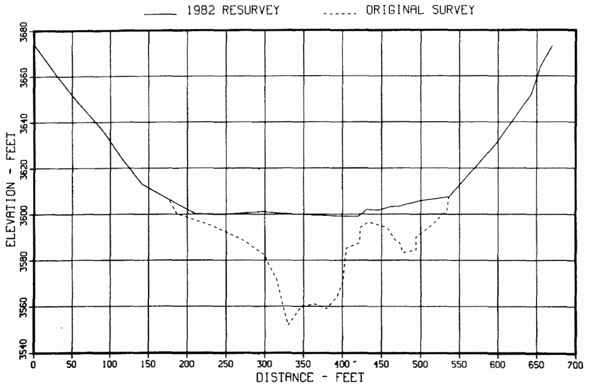
Figure 53. - Original and 1982 sedimentation range profiles, range 19.
