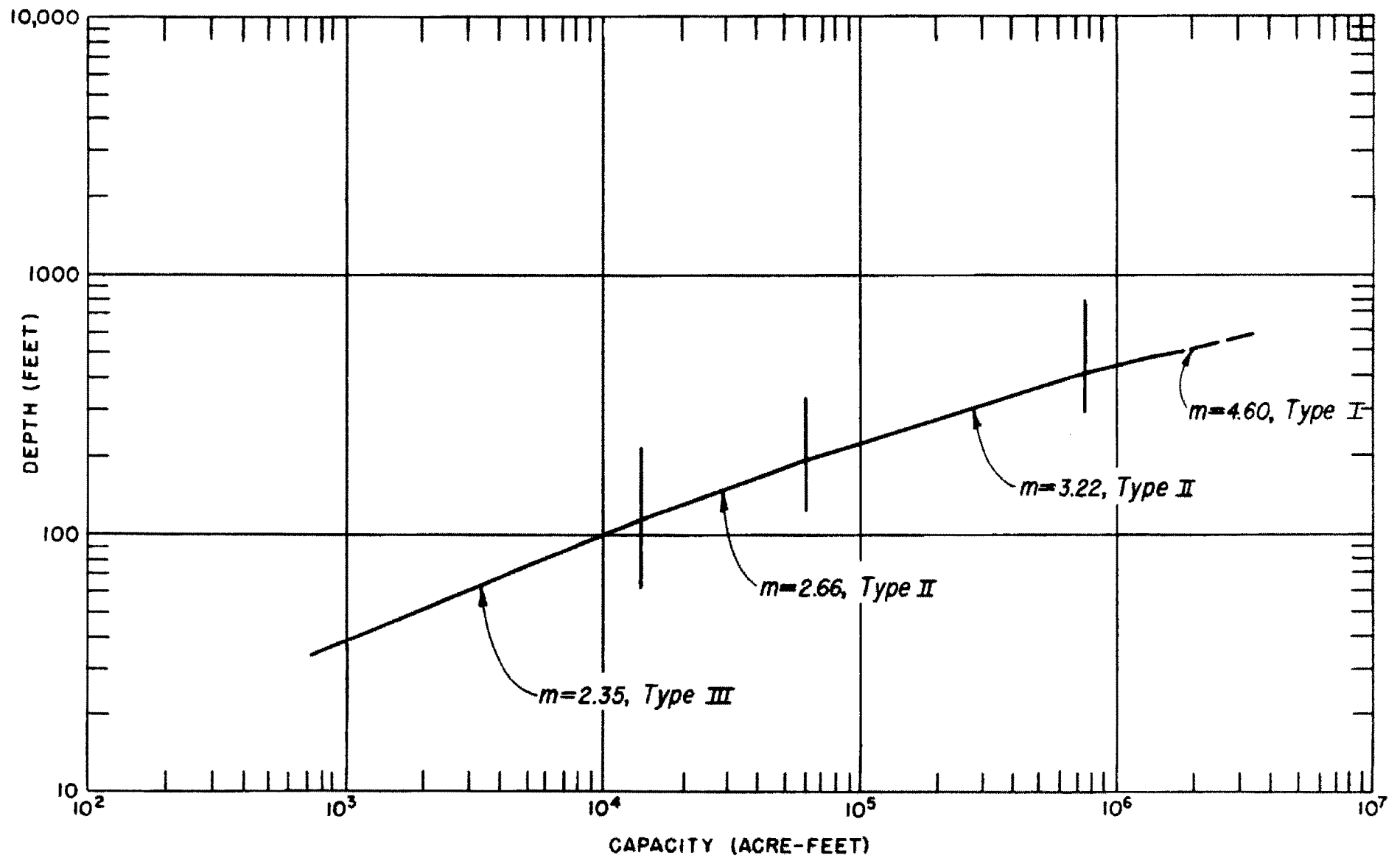
Figure 34. - Depth-capacity relationship.
