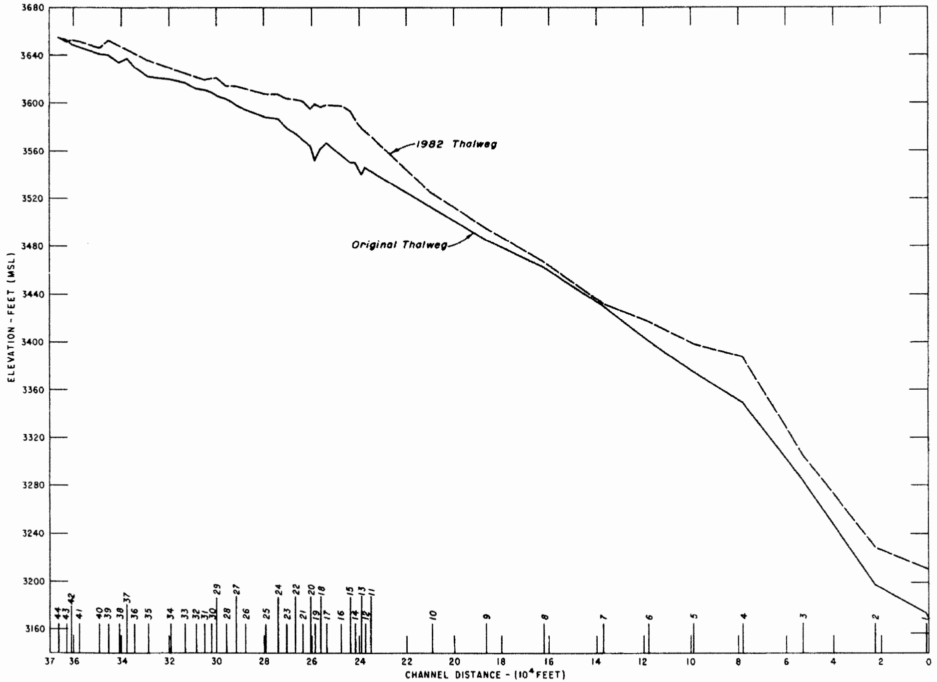
Figure 30. - Longitudinal thalweg profiles for Bighorn Lake.
