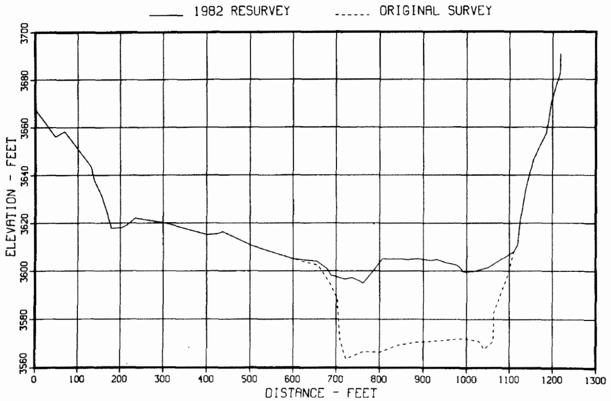
Figure 54. - Original and 1982 sedimentation range profiles, range 20.
