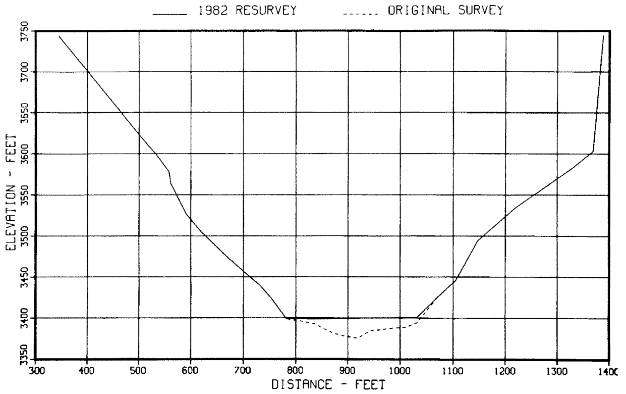
Figure 39. - Original and 1982 sedimentation range profiles, range 5.
