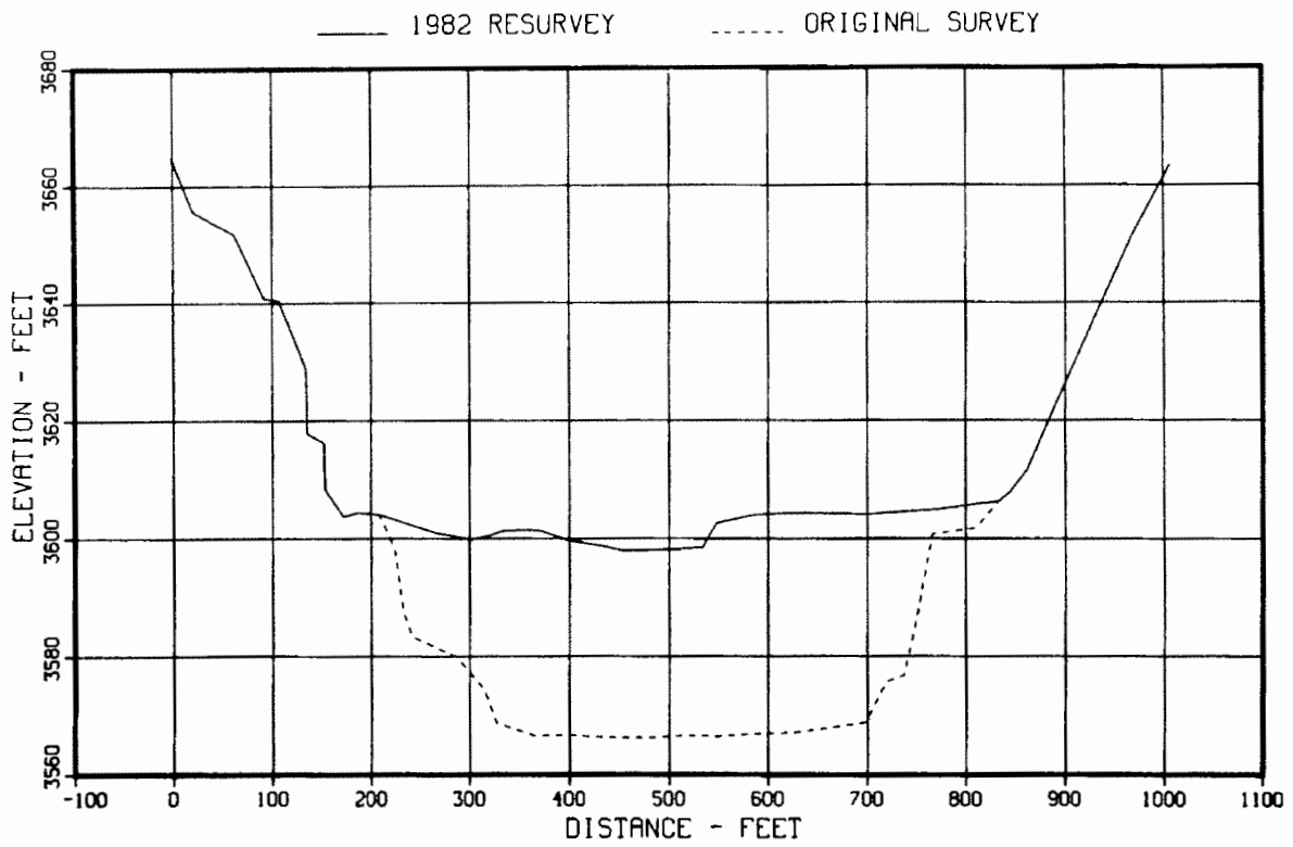
Figure 51. - Original and 1982 sedimentation range profiles, range 17.
