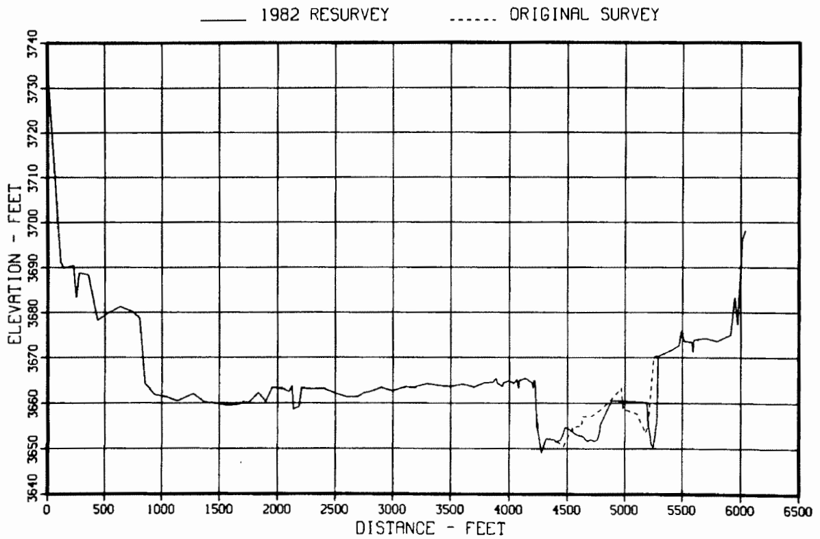
Figure 76. - Original and 1982 sedimentation range profiles, range 42.
