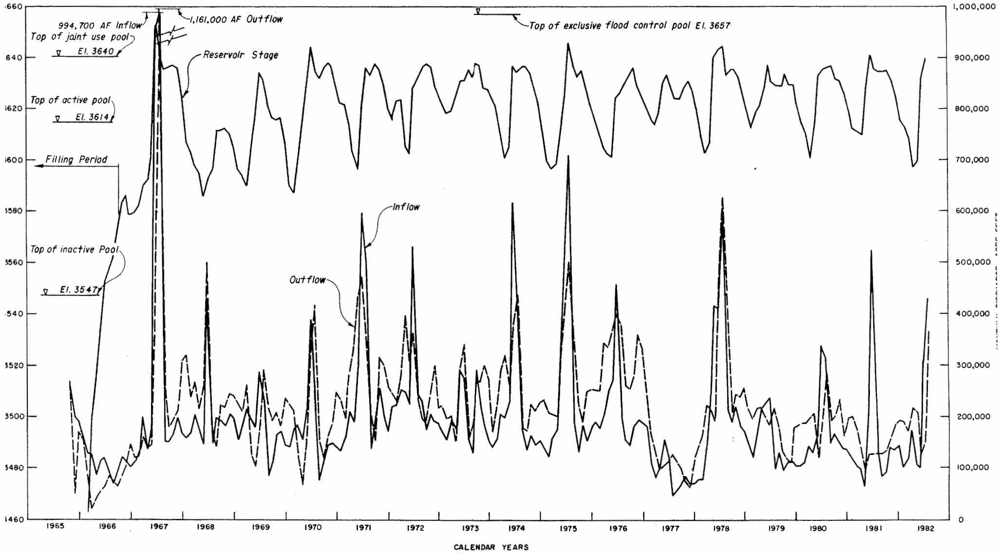
Figure 4. - Reservoir operation, 1965-1982.
