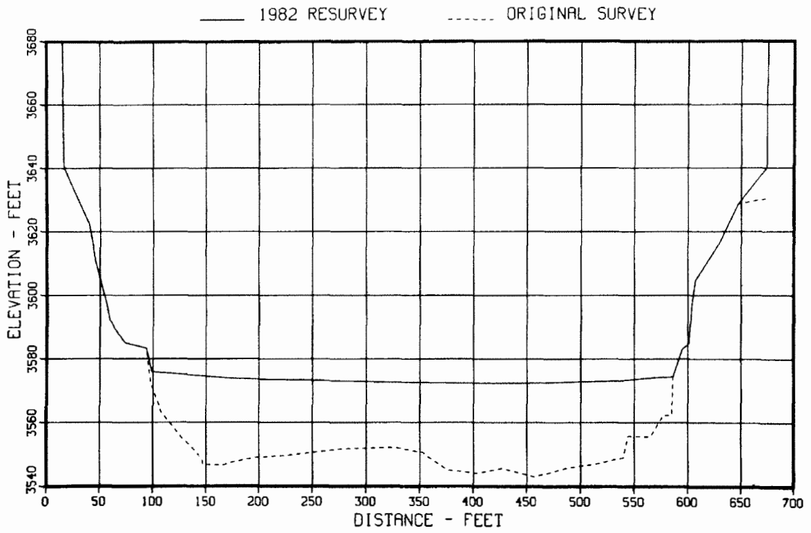
Figure 45. - Original and 1982 sedimentation range profiles, range 11.
