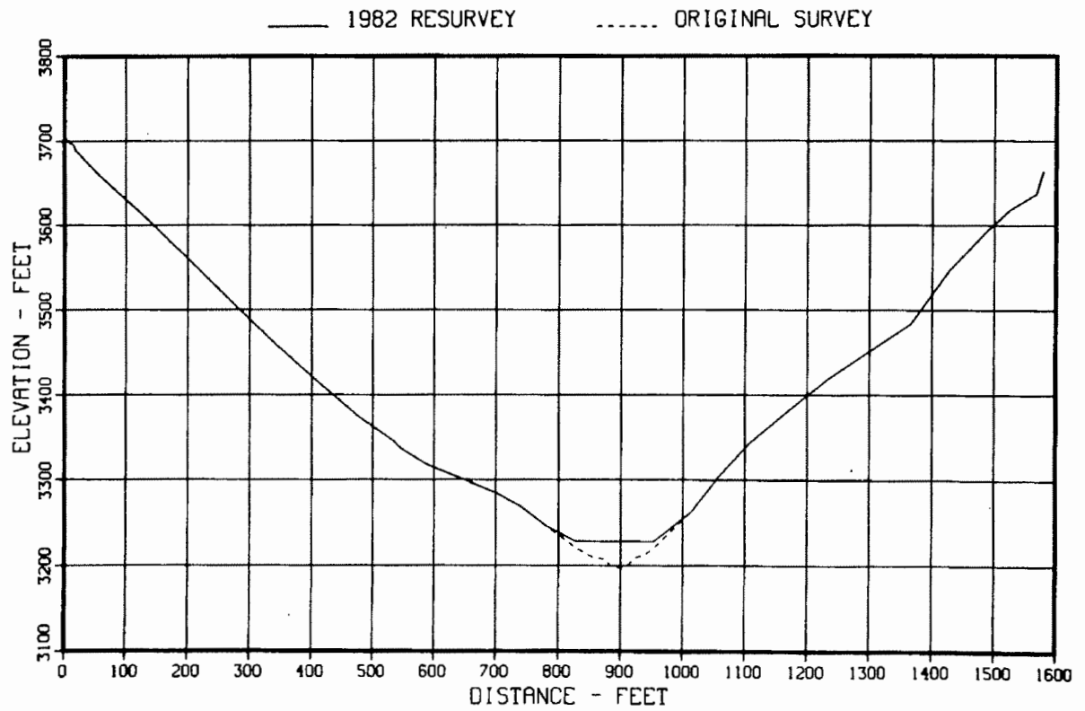
Figure 36. - Original and 1982 sedimentation range profiles, range 2.
