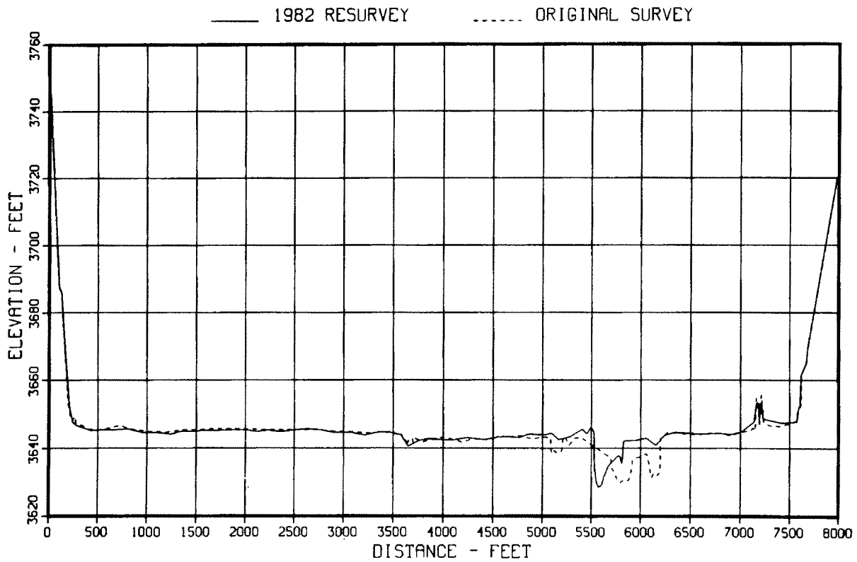
Figure 70. - Original and 1982 sedimentation range profiles, range 36.
