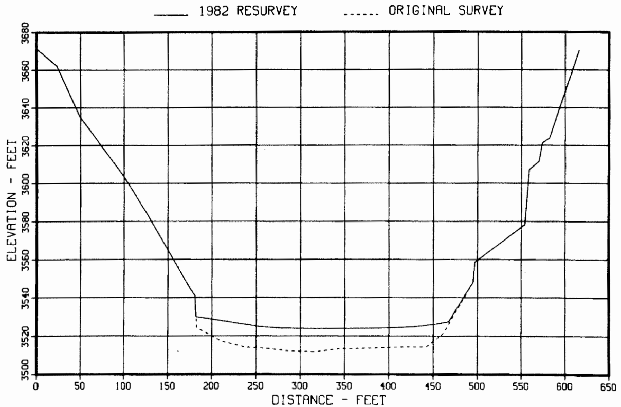
Figure 44. - Original and 1982 sedimentation range profiles, range 10.
