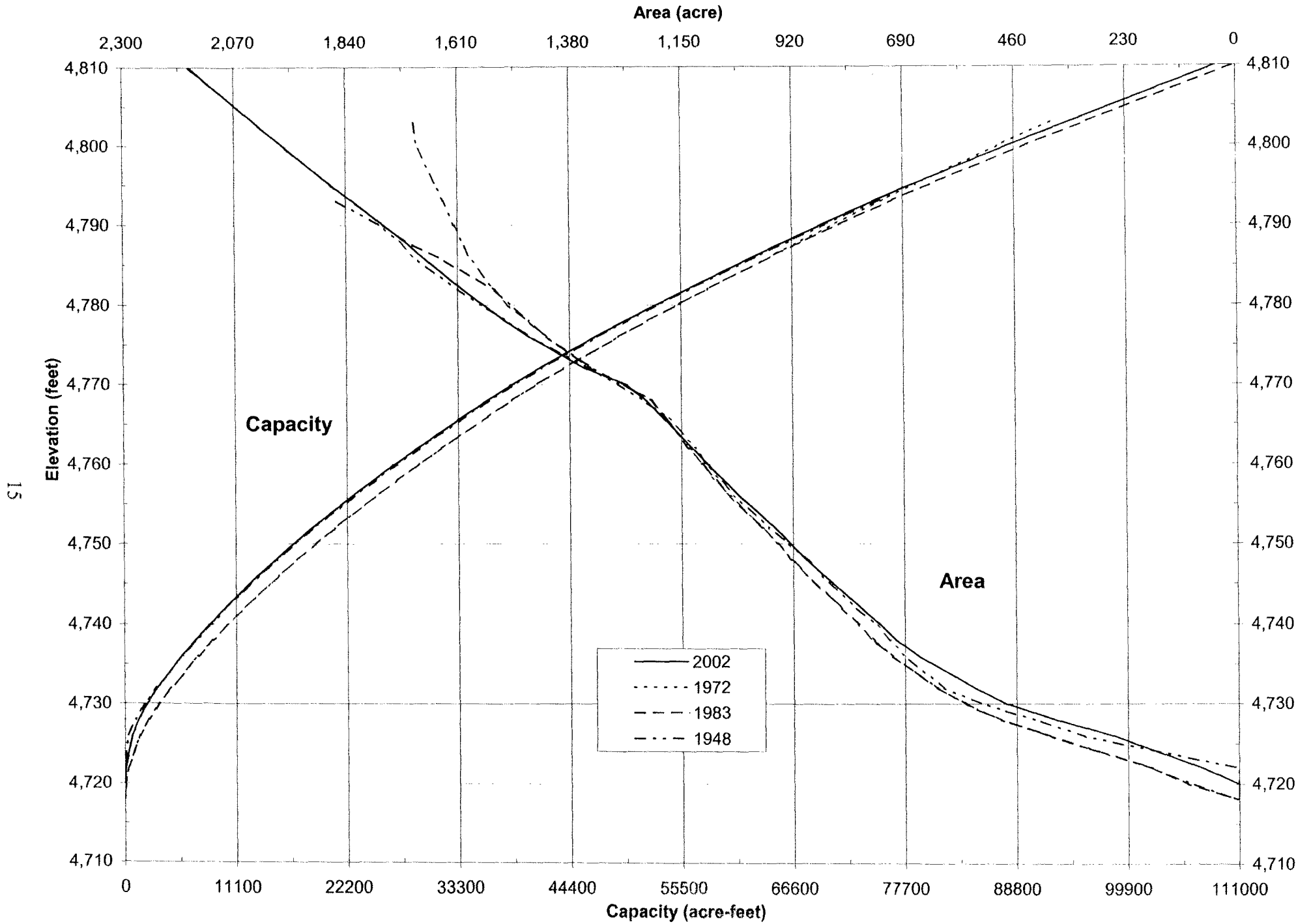
Figure 3. - 2002 area and capacity curves.
