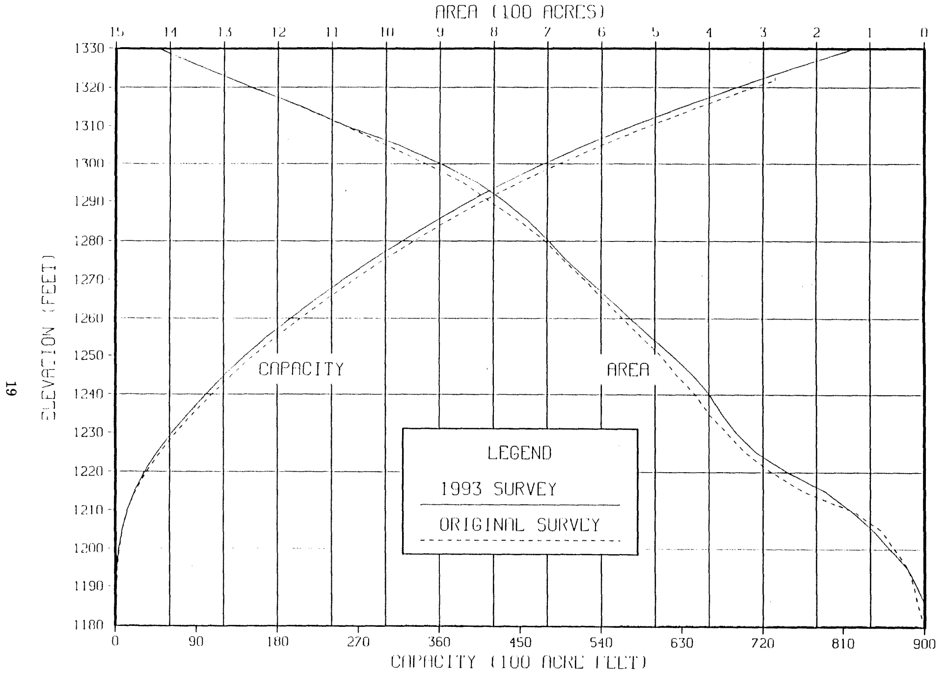
Figure 4. - Area and capacity curves — McKay Reservoir.
