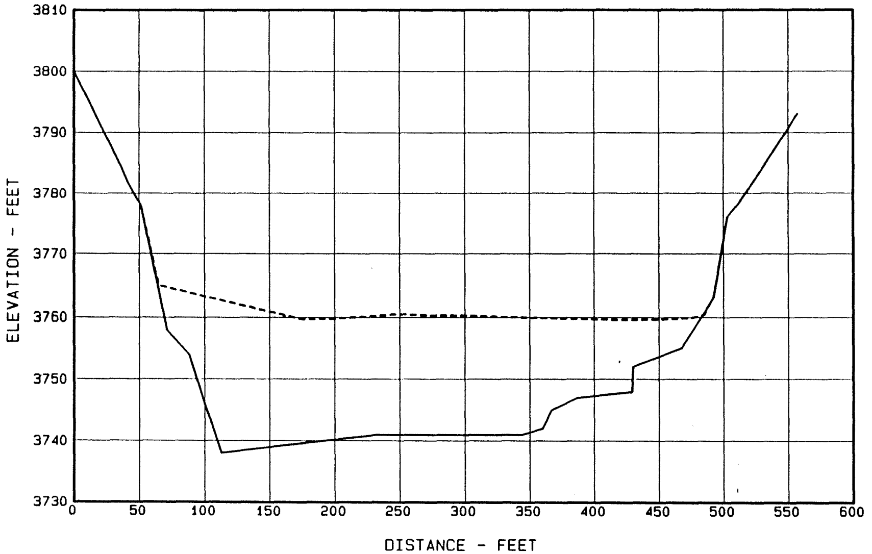
Figure 35. - Sediment Range 103 - Ute Creek.
