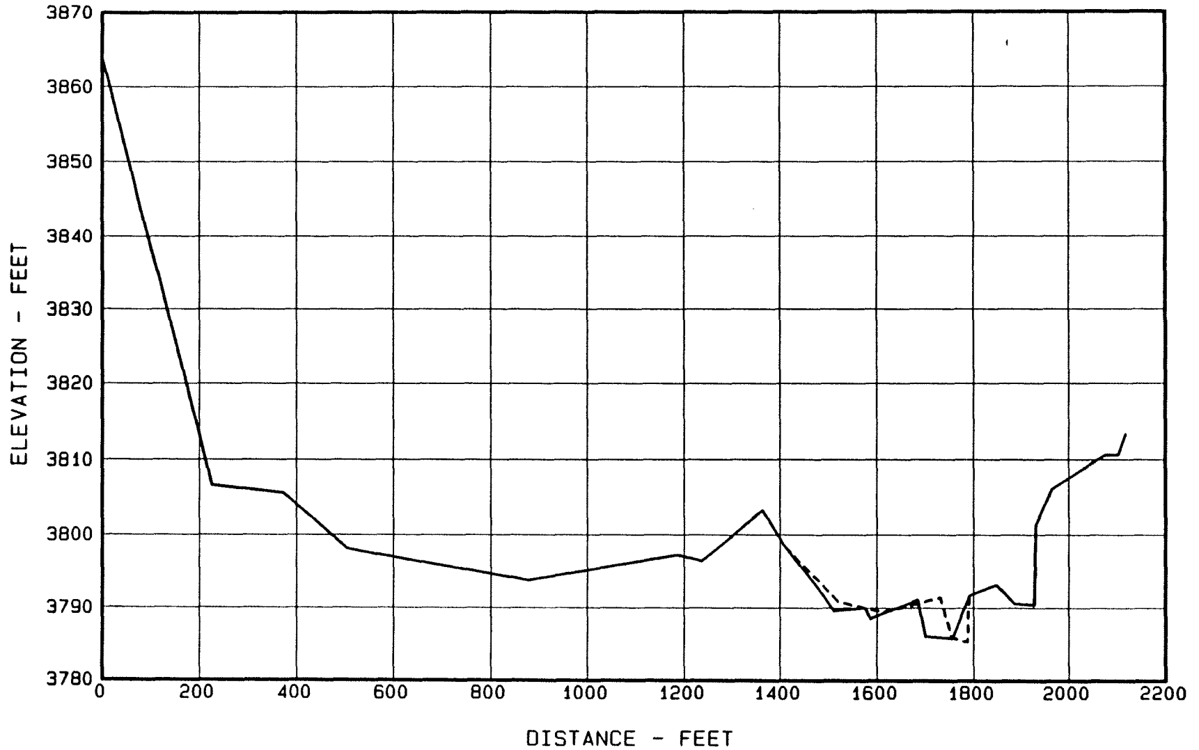
Figure 31. - Sediment Range 21 - Canadian River. 45
