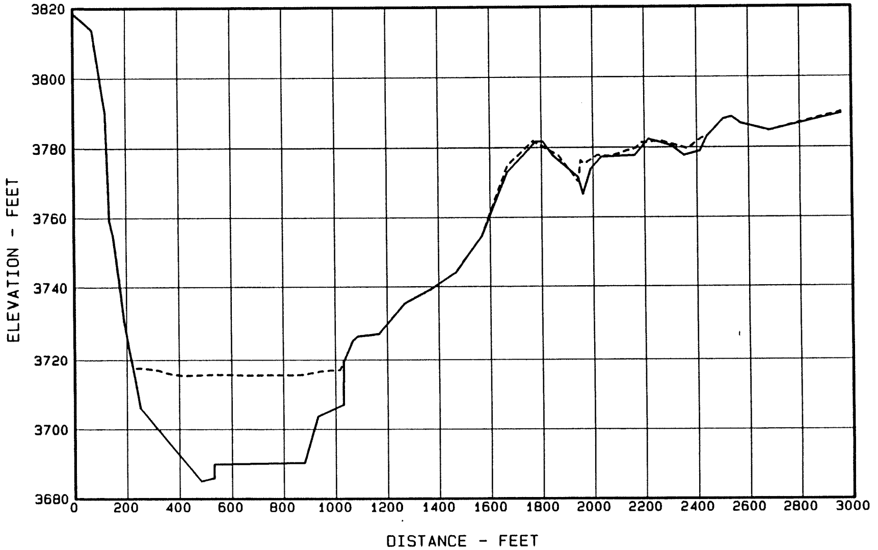
Figure 14. - Sediment Range 4 - Canadian River.
