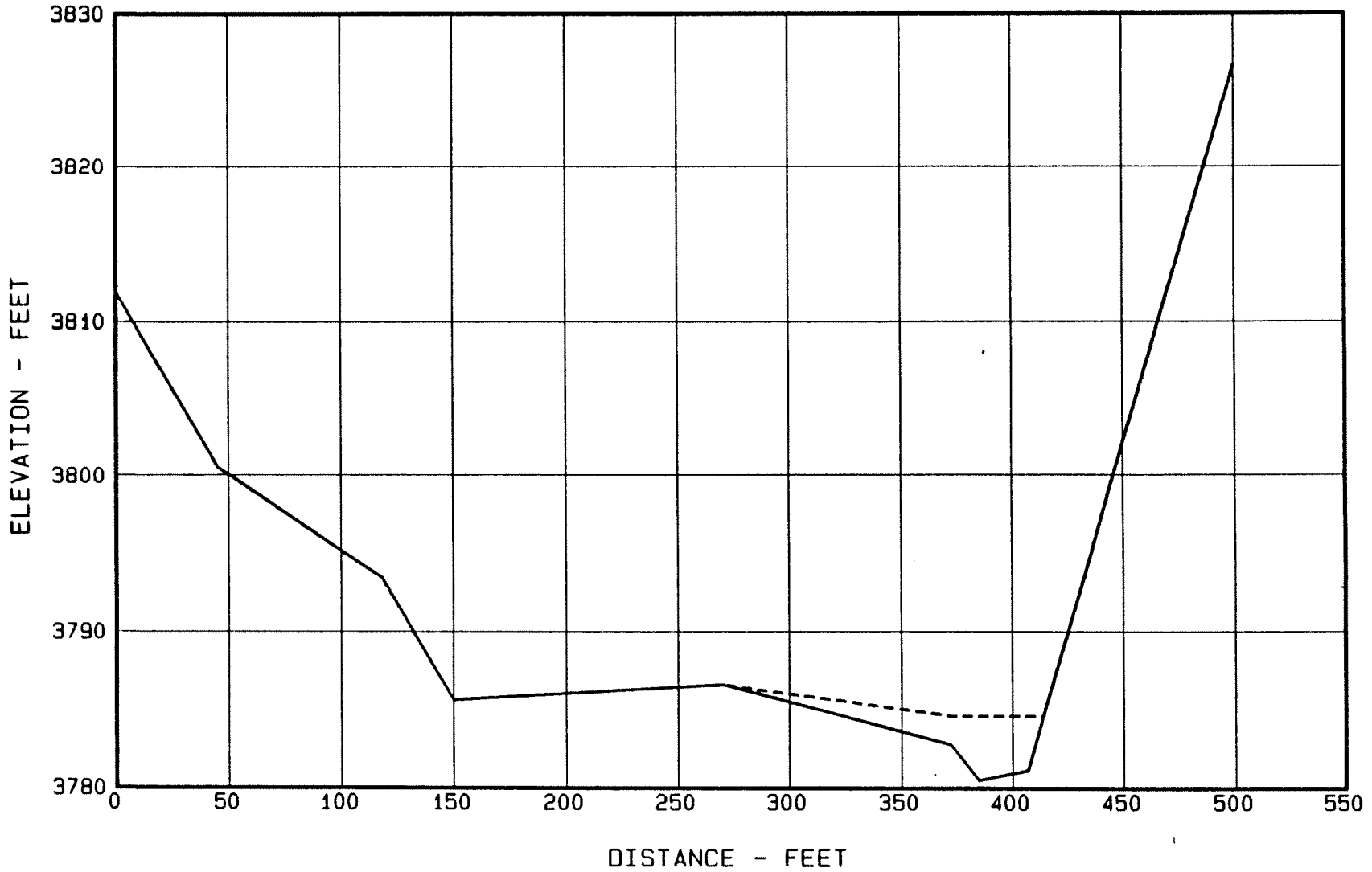
Figure 42. - Sediment Range 302 - Carras Creek.
