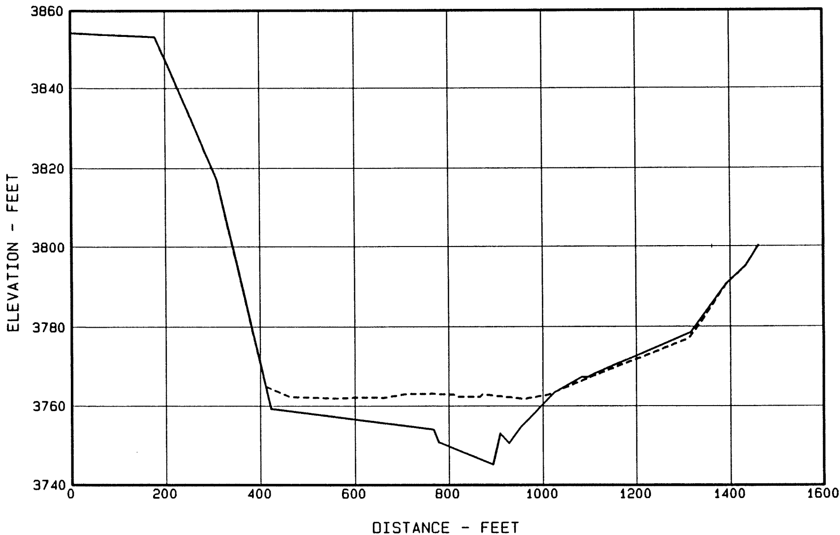
Figure 22. - Sediment Range 12 - Canadian River.
