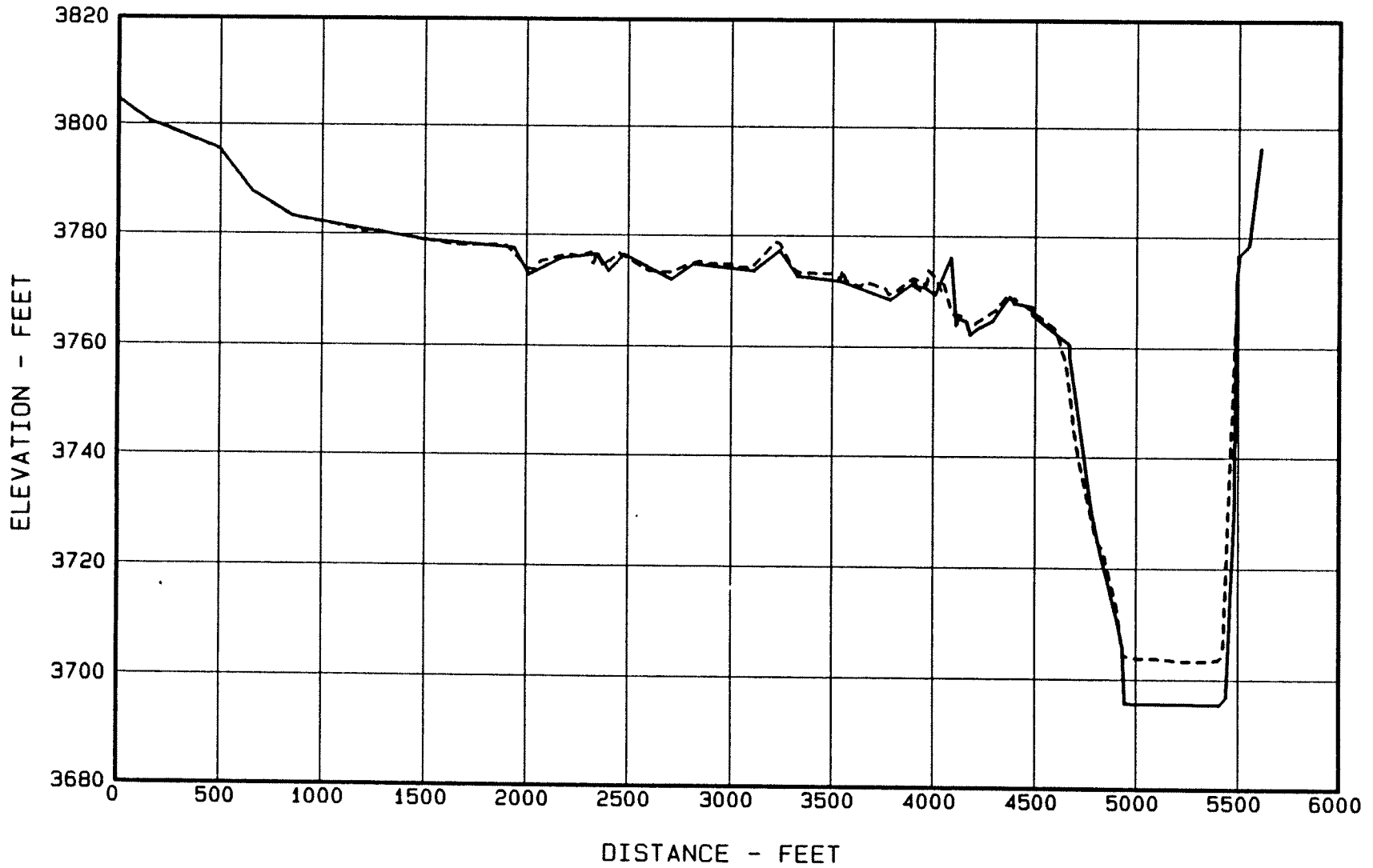
Figure 11. - Sediment Range 1 - Canadian River.
