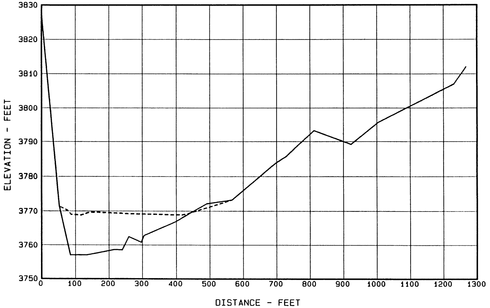
Figure 24. - Sediment Range 14 - Canadian River.
