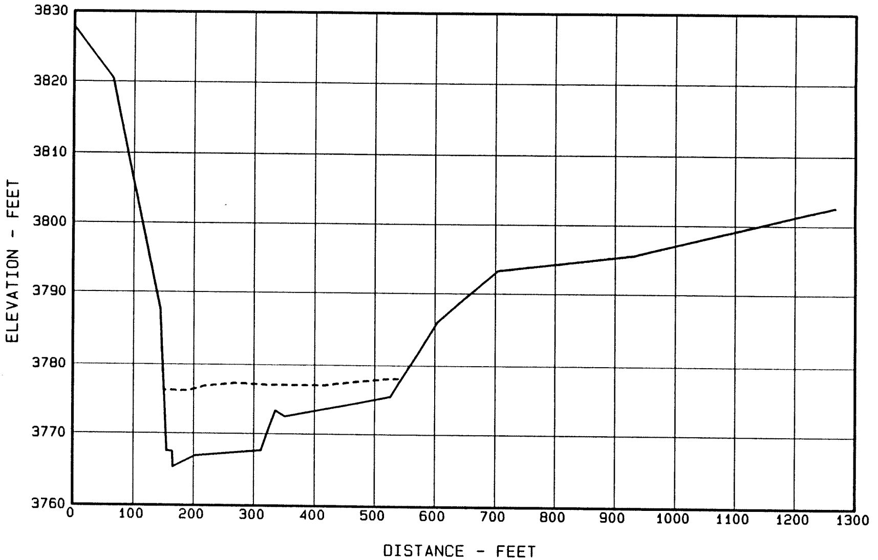
Figure 27. - Sediment Range 17 - Canadian River.
