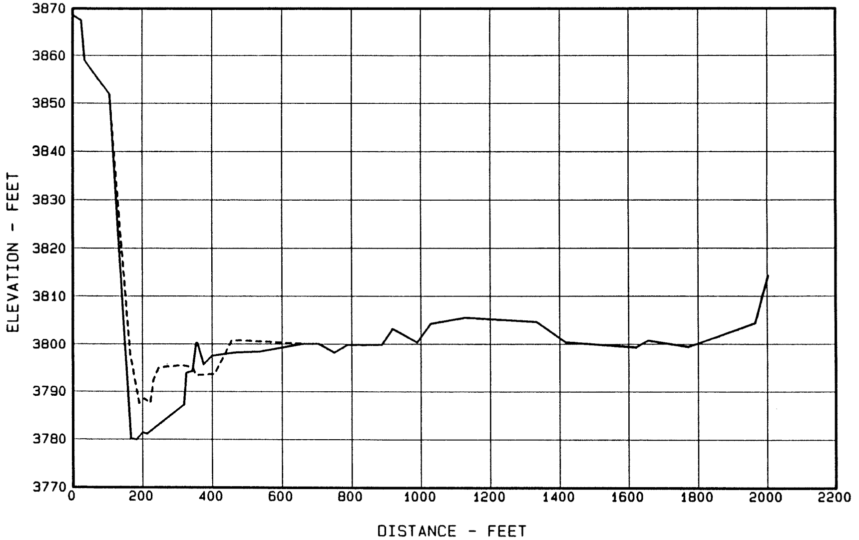
Figure 32. - Sediment Range 22 - Canadian River.
