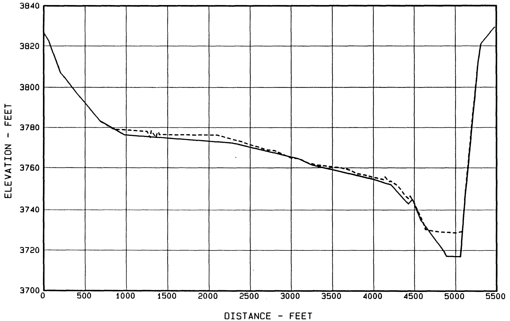
Figure 17. - Sediment Range 7 - Canadian River.
