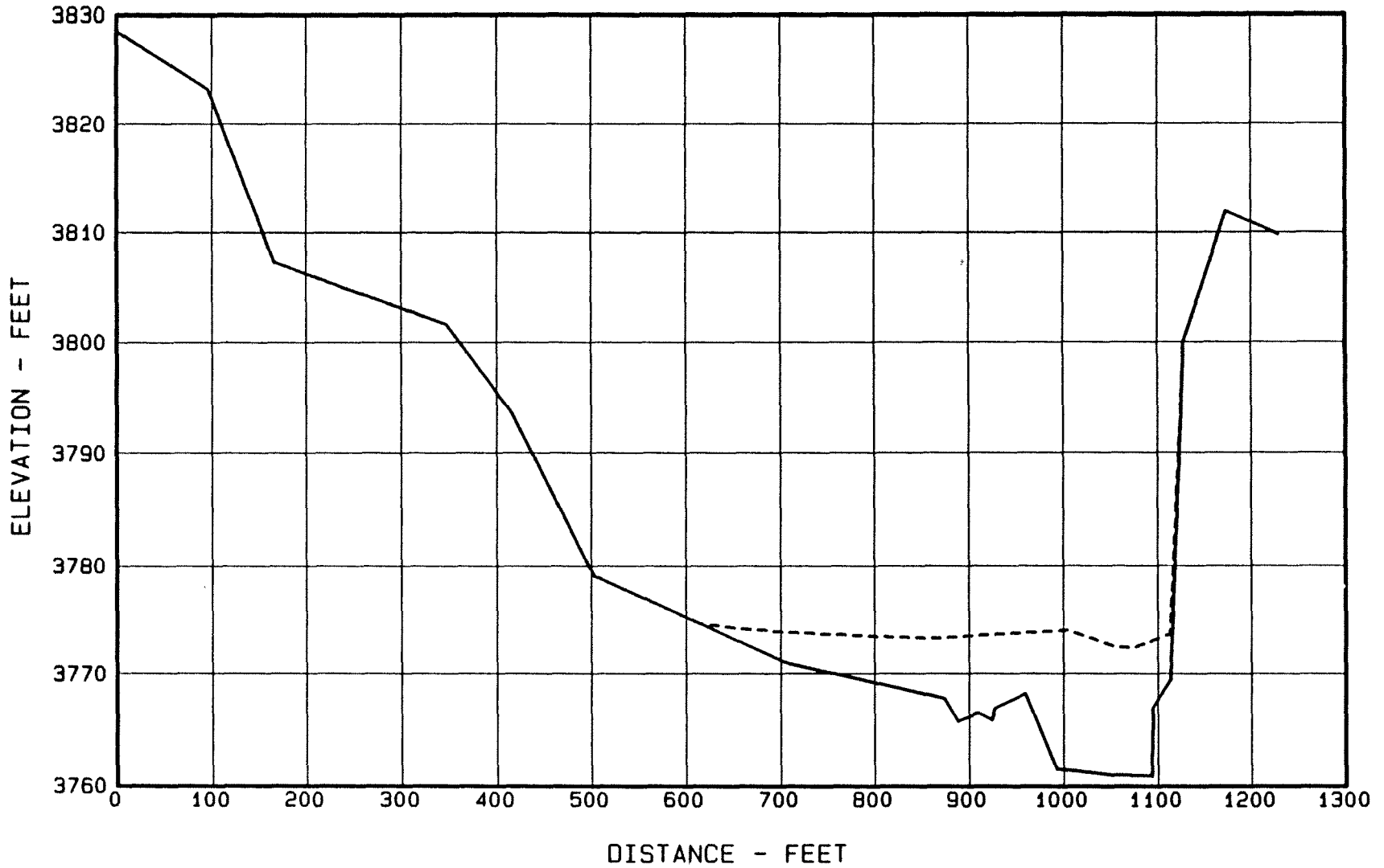
Figure 25. - Sediment Range 15 - Canadian River.
