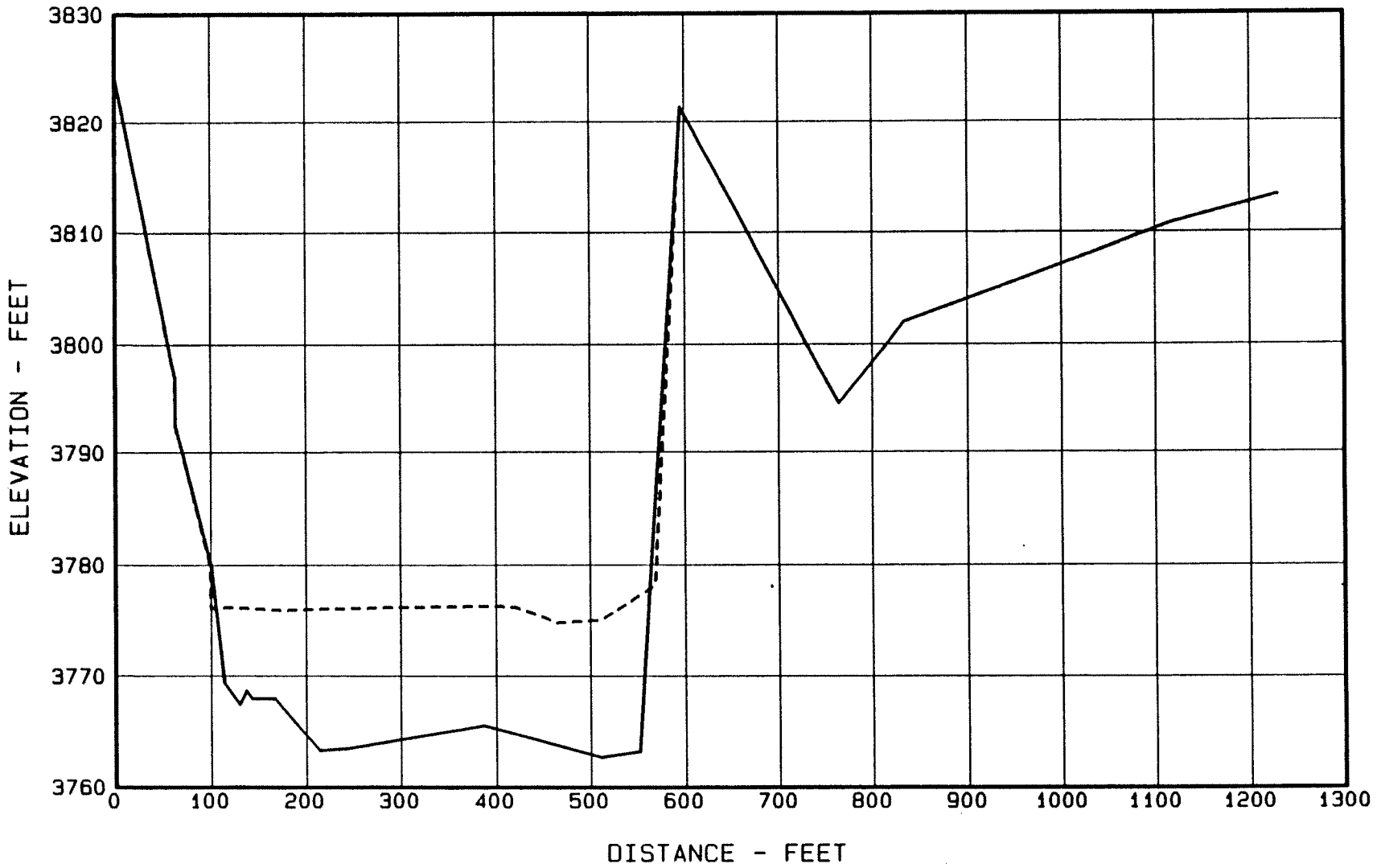
Figure 26. - Sediment Range 16 - Canadian River. 40
