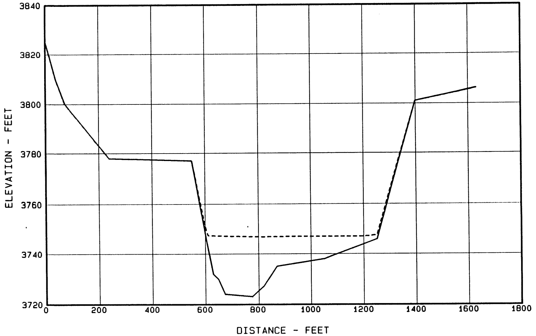
Figure 34. - Sediment Range 102 - Ute Creek.
