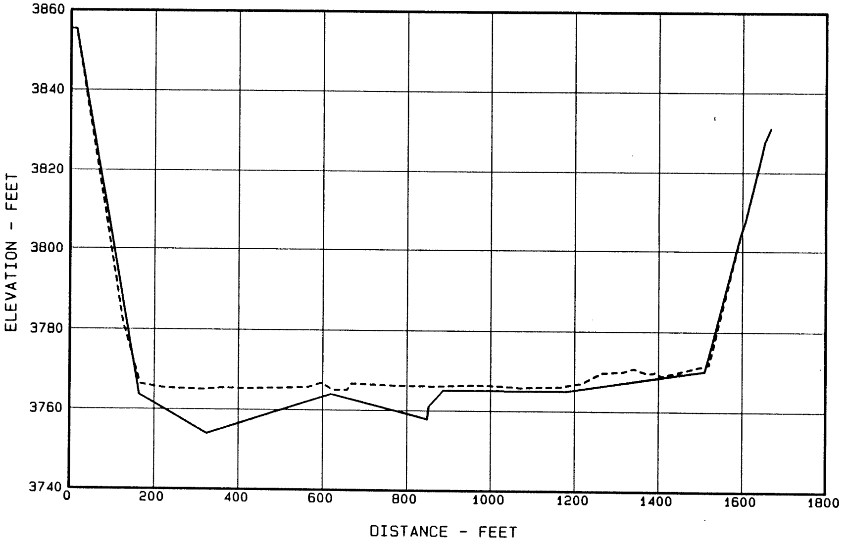
Figure 23. - Sediment Range 13 - Canadian River.
