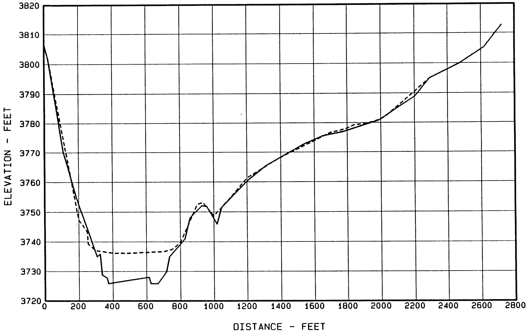
Figure 18. - Sediment Range 8 - Canadian River.
