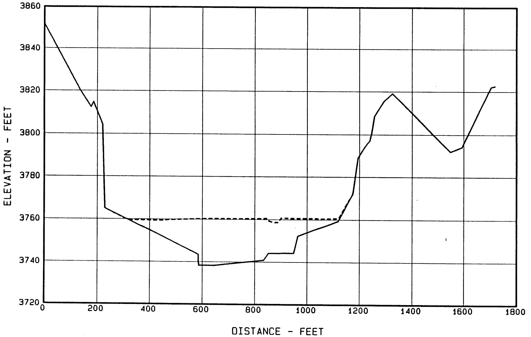
Figure 21. - Sediment Range 11 - Canadian River.
