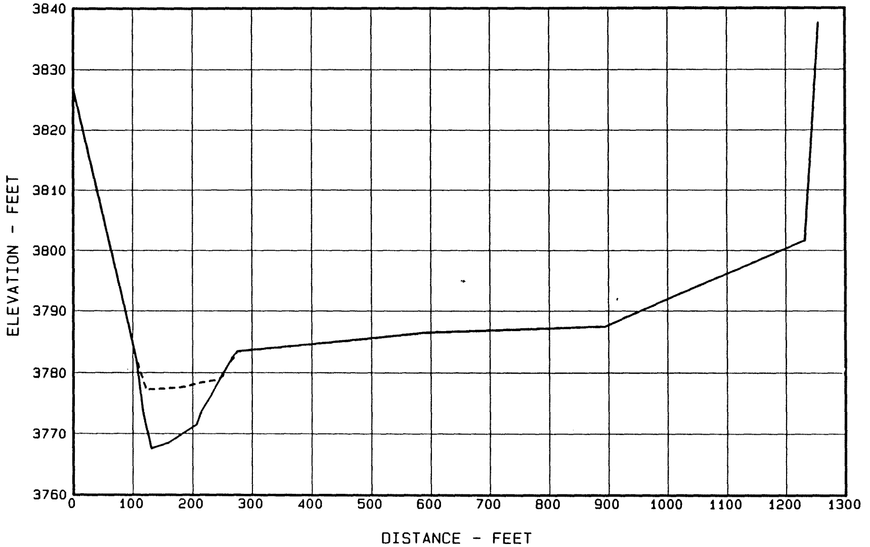
Figure 41. - Sediment Range 301 - Carrizo Creek.
