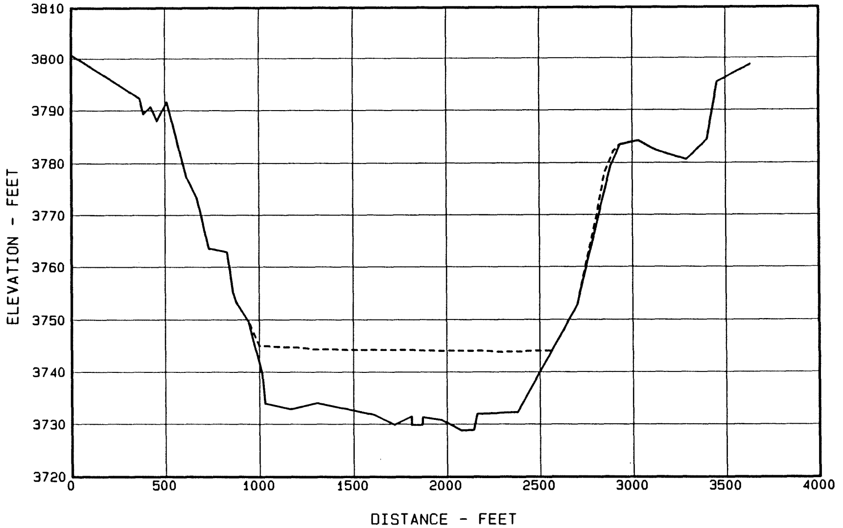
Figure 19. - Sediment Range 9 - Canadian River.
