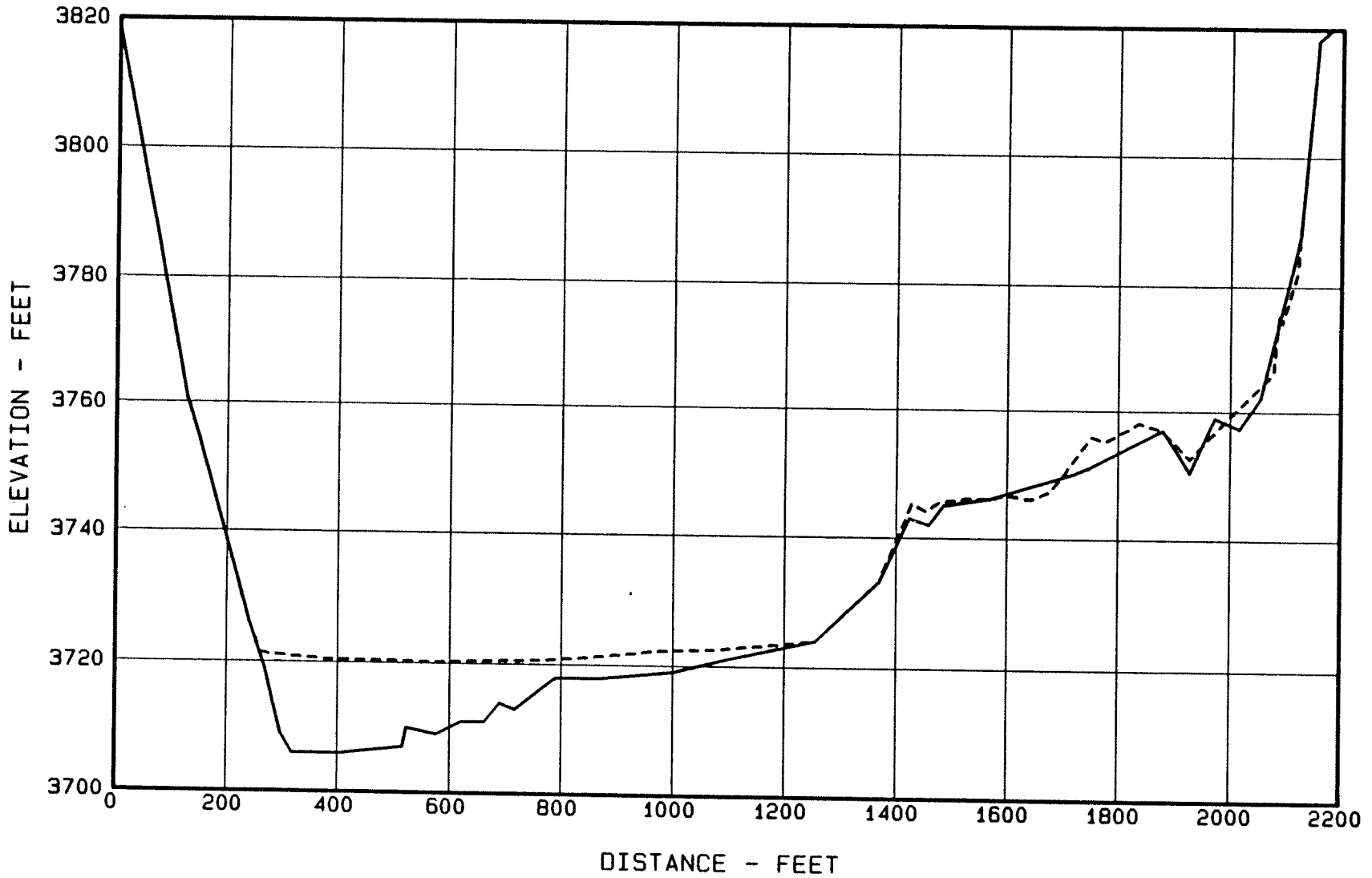
Figure 33. - Sediment Range 101 - Ute Creek.
