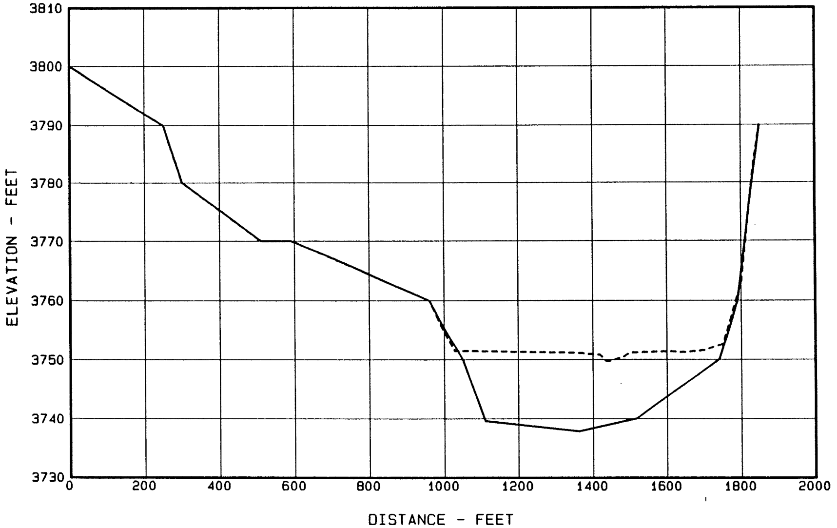
Figure 20. - Sediment Range 10 - Canadian River.
