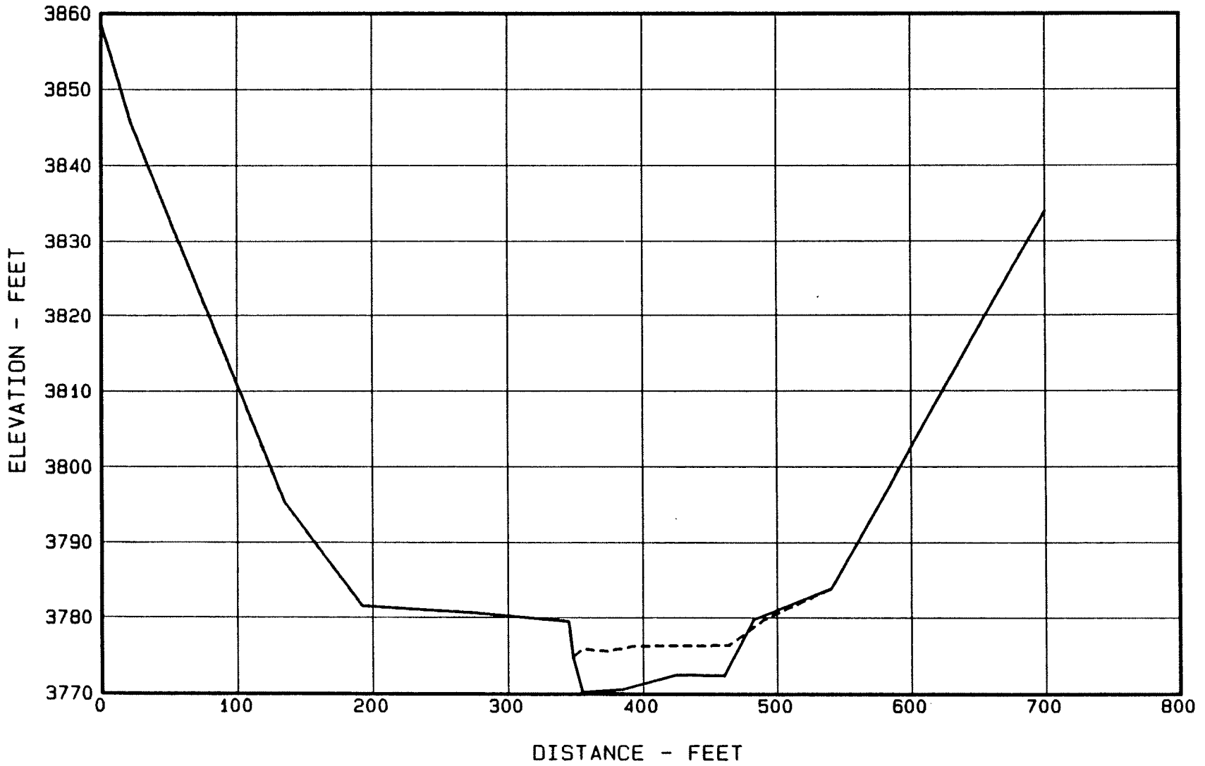
Figure 40. - Sediment Range 201 - Dripping Springs.
