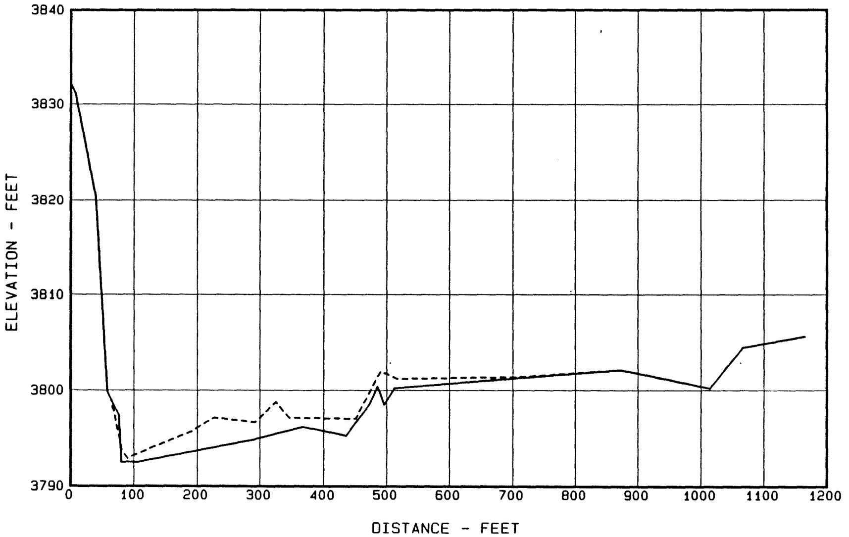
Figure 39. - Sediment Range 107 - Ute Creek.
