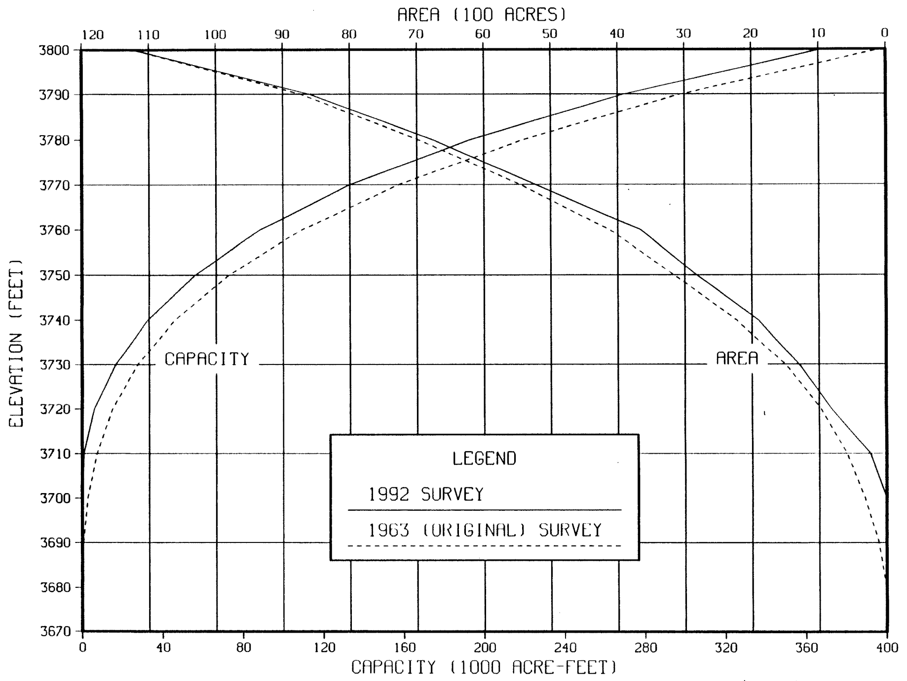
Figure 6. - Area and capacity curves - Ute Reservoir.
