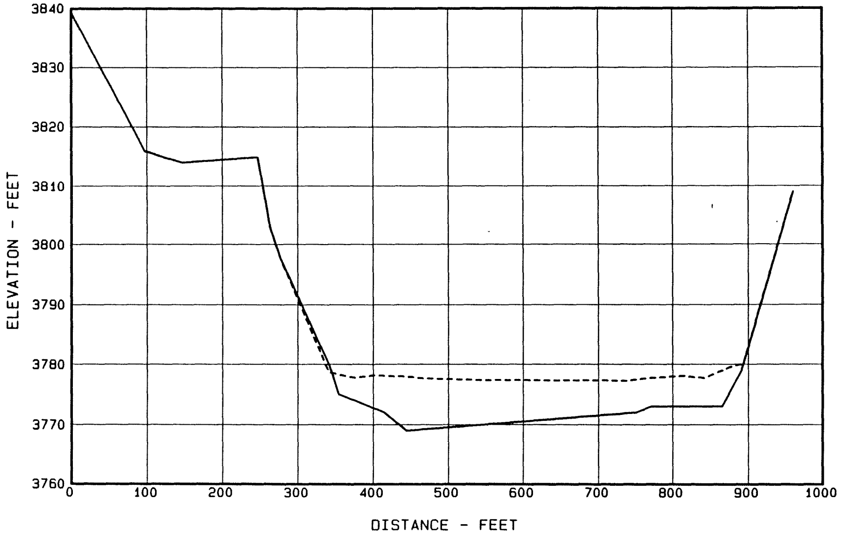
Figure 37. - Sediment Range 105 - Ute Creek.
