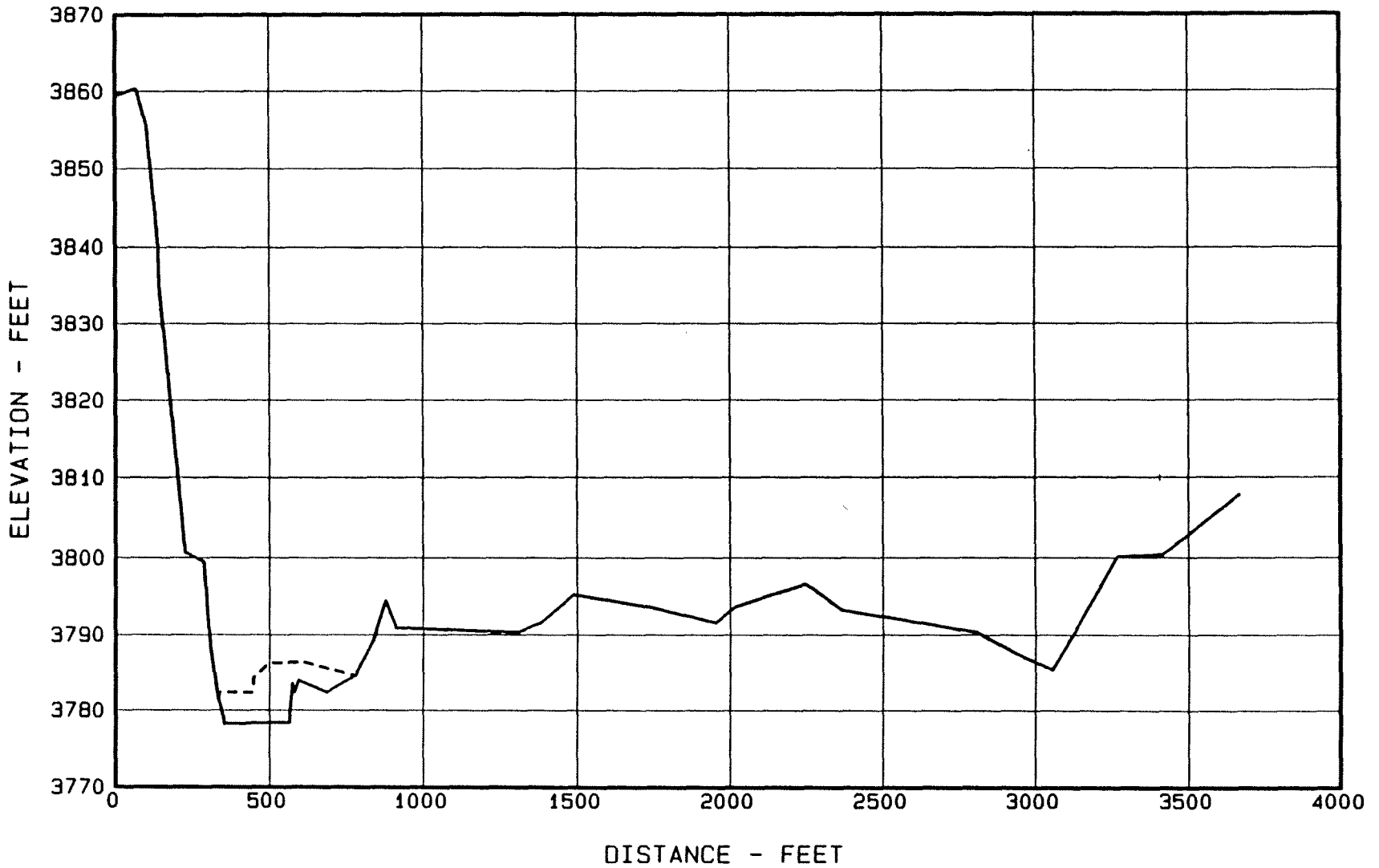
Figure 29. - Sediment Range 19 - Canadian River. 43
