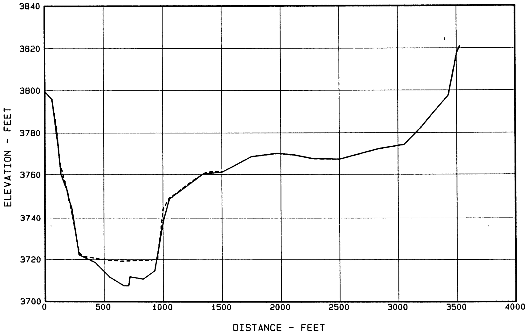
30 Figure 16. - Sediment Range 6 - Canadian River.
