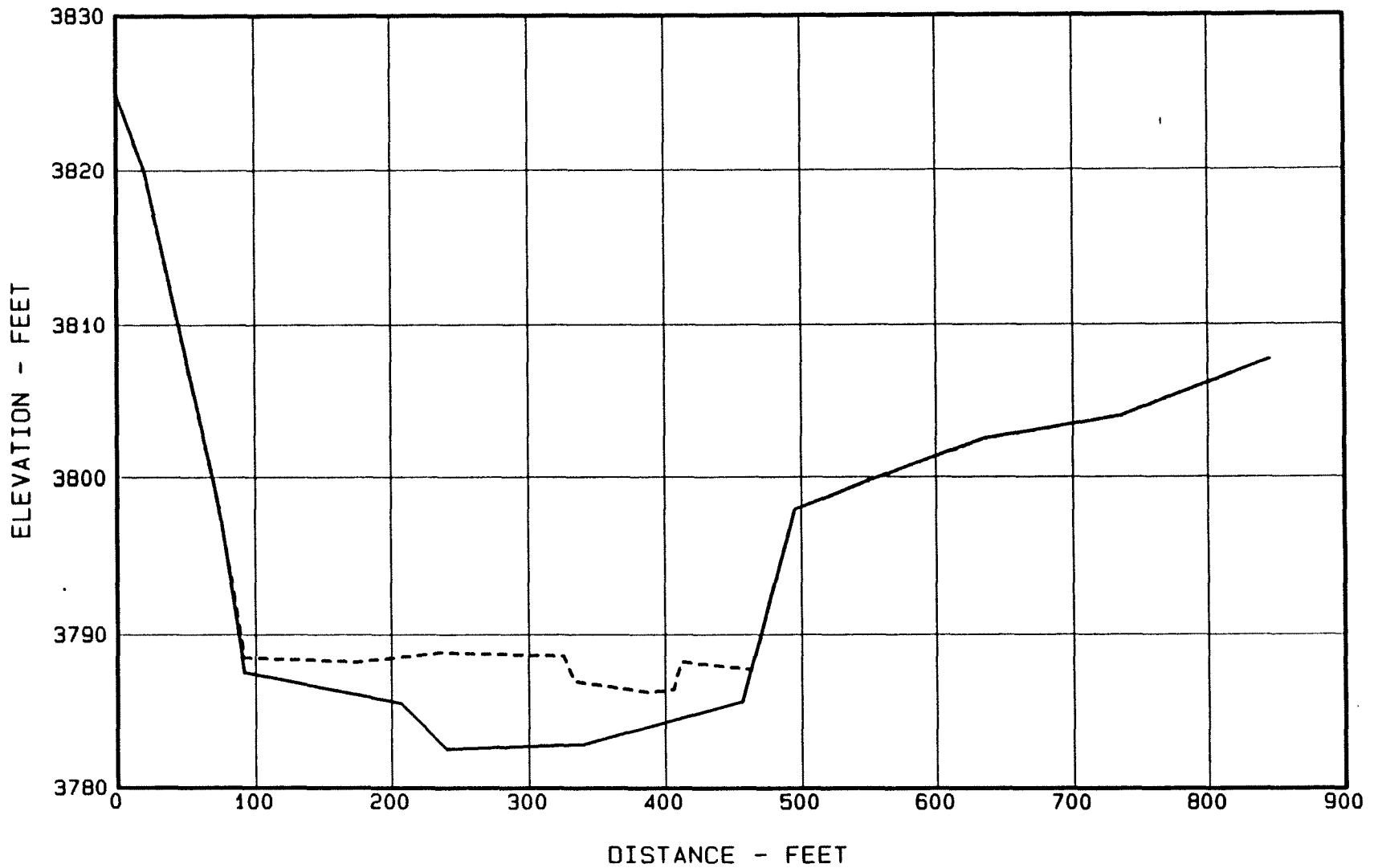
Figure 38. - Sediment Range 106 - Ute Creek.
