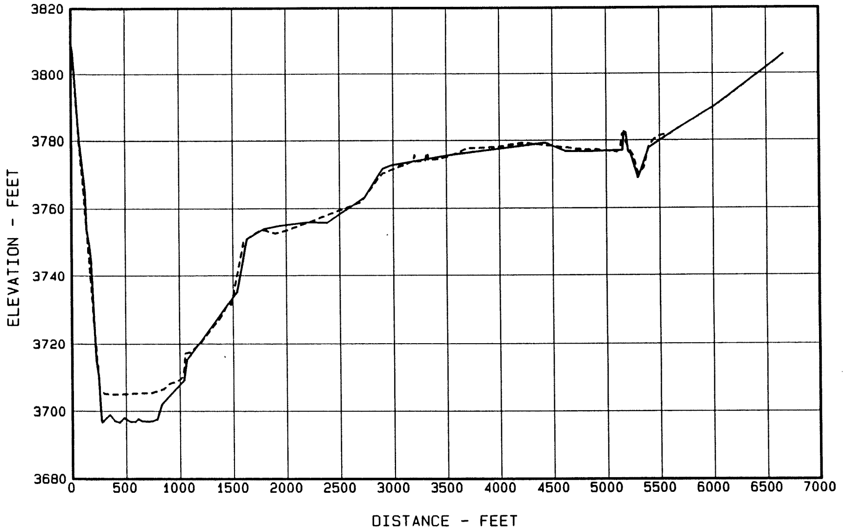
Figure 12. - Sediment Range 2 - Canadian River.
