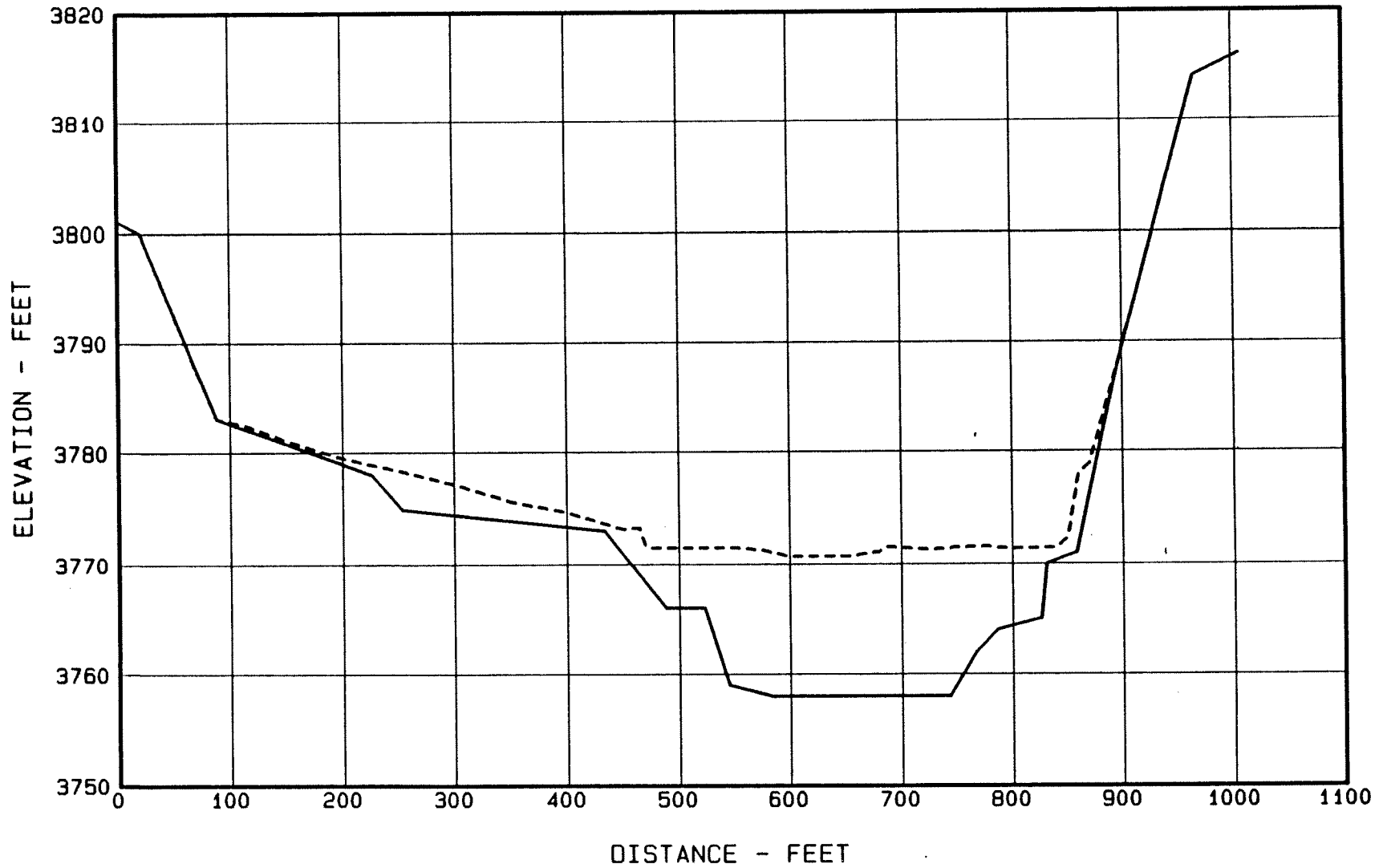
Figure 36. - Sediment Range 104 - Ute Creek.
