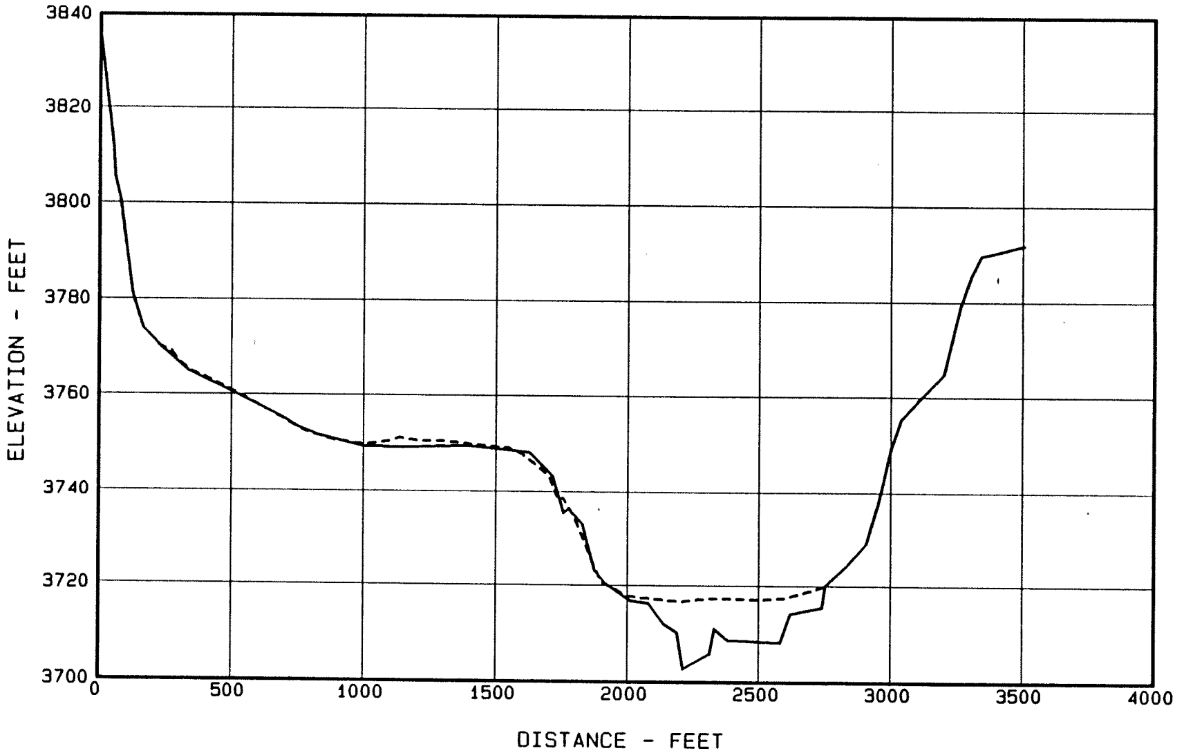
Figure 15. - Sediment Range 5 - Canadian River. 29
