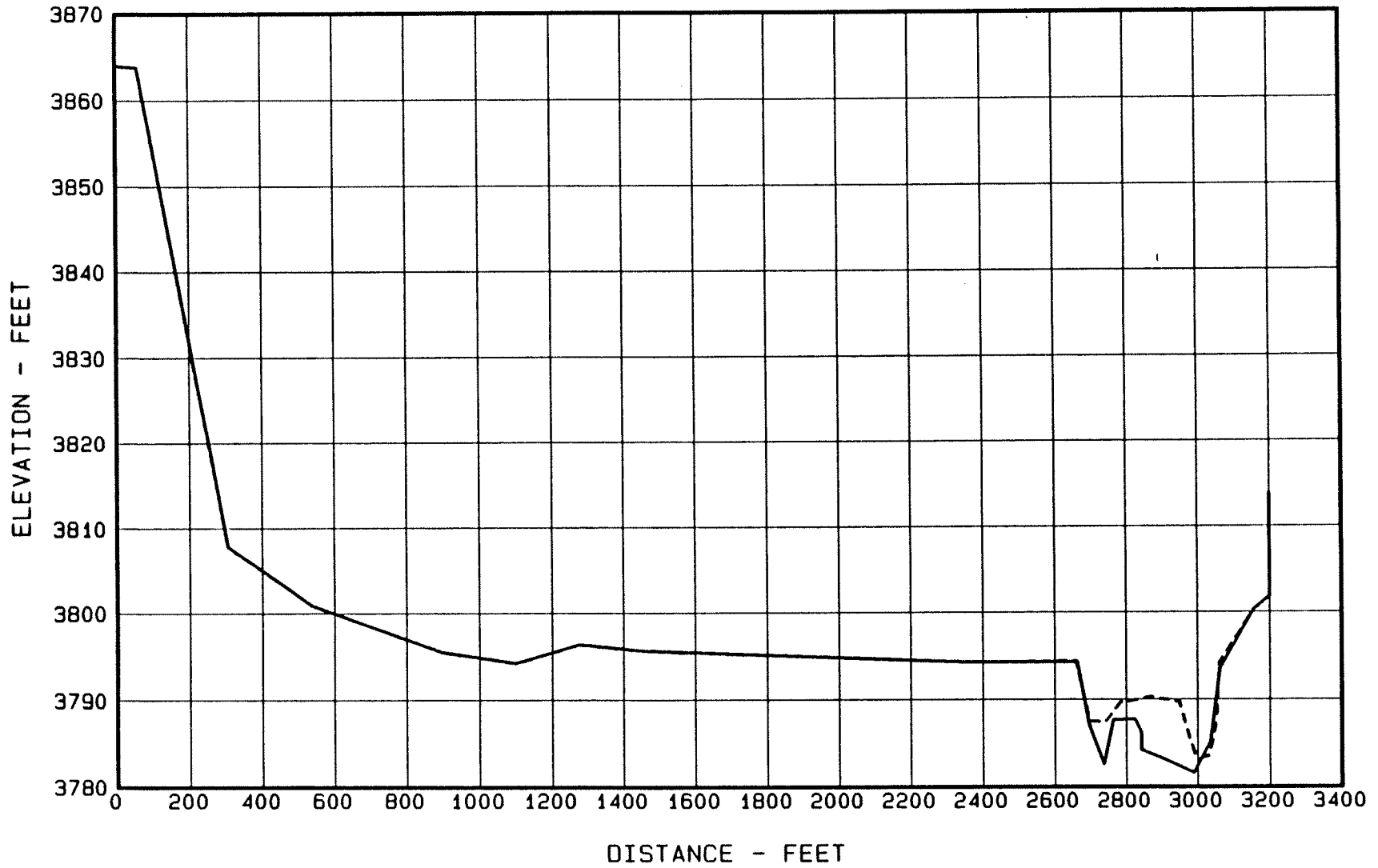
Figure 30. - Sediment Range 20 - Canadian River.
