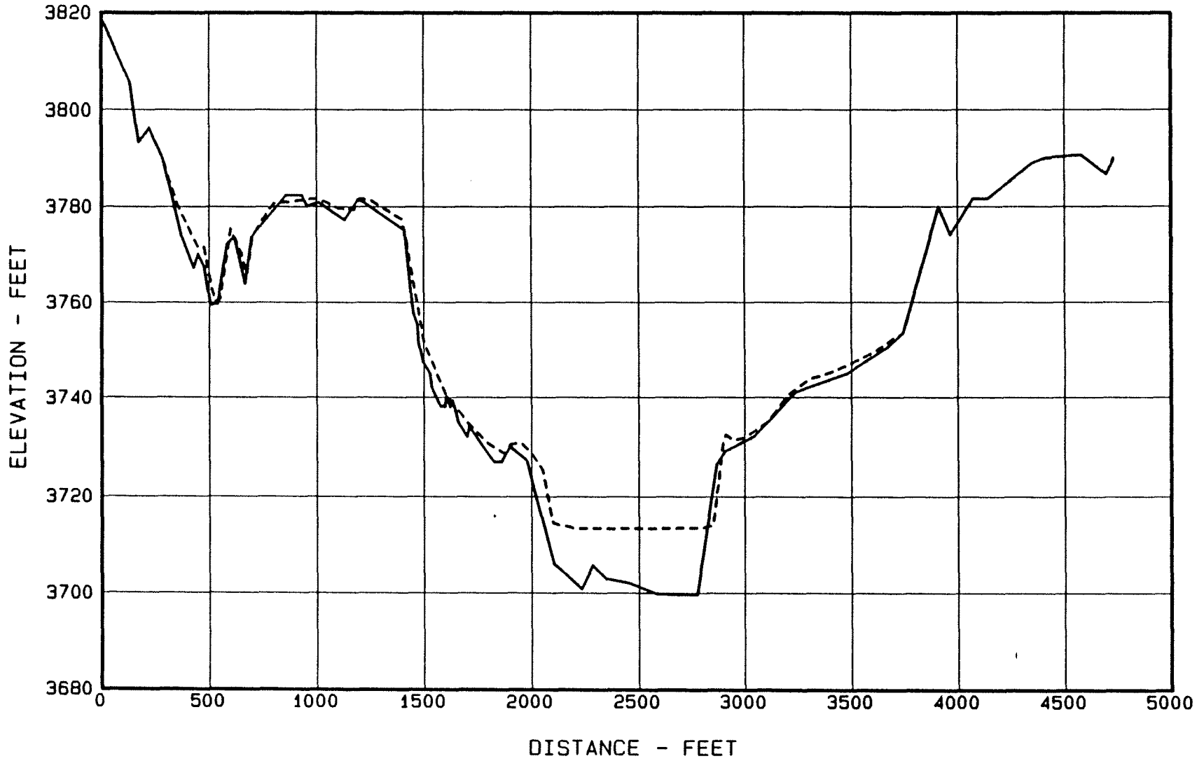
Figure 13. - Sediment Range 3 - Canadian River.
