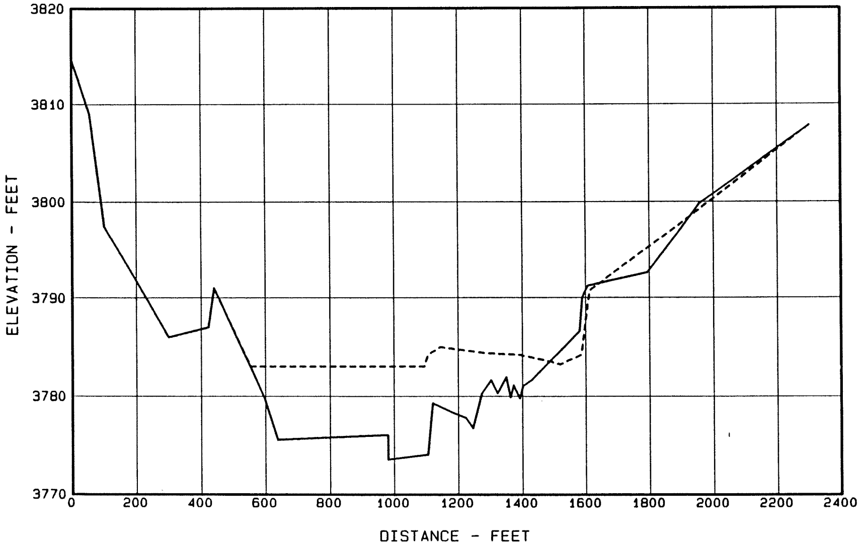
Figure 28. - Sediment Range 18 - Canadian River.
