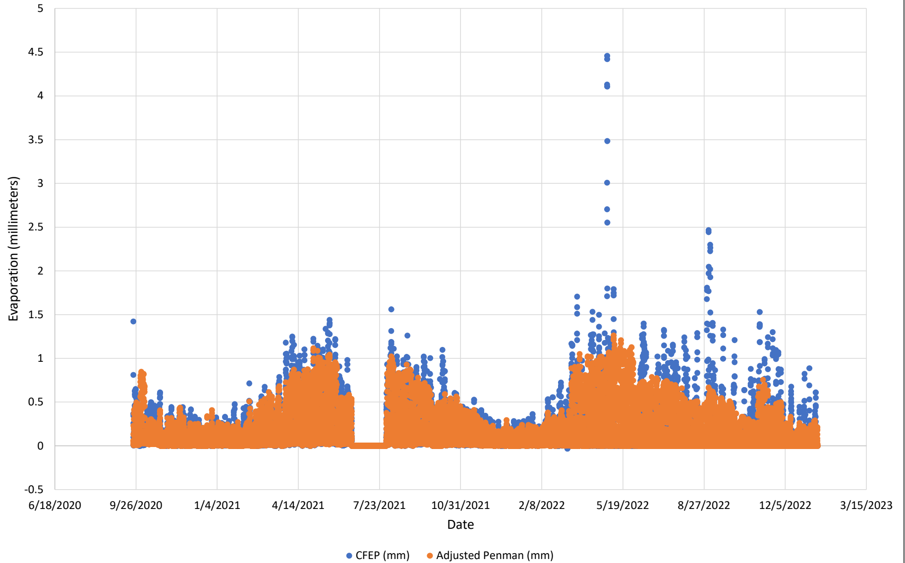
Evaporation Comparison: CFEP vs Adjusted Penman
